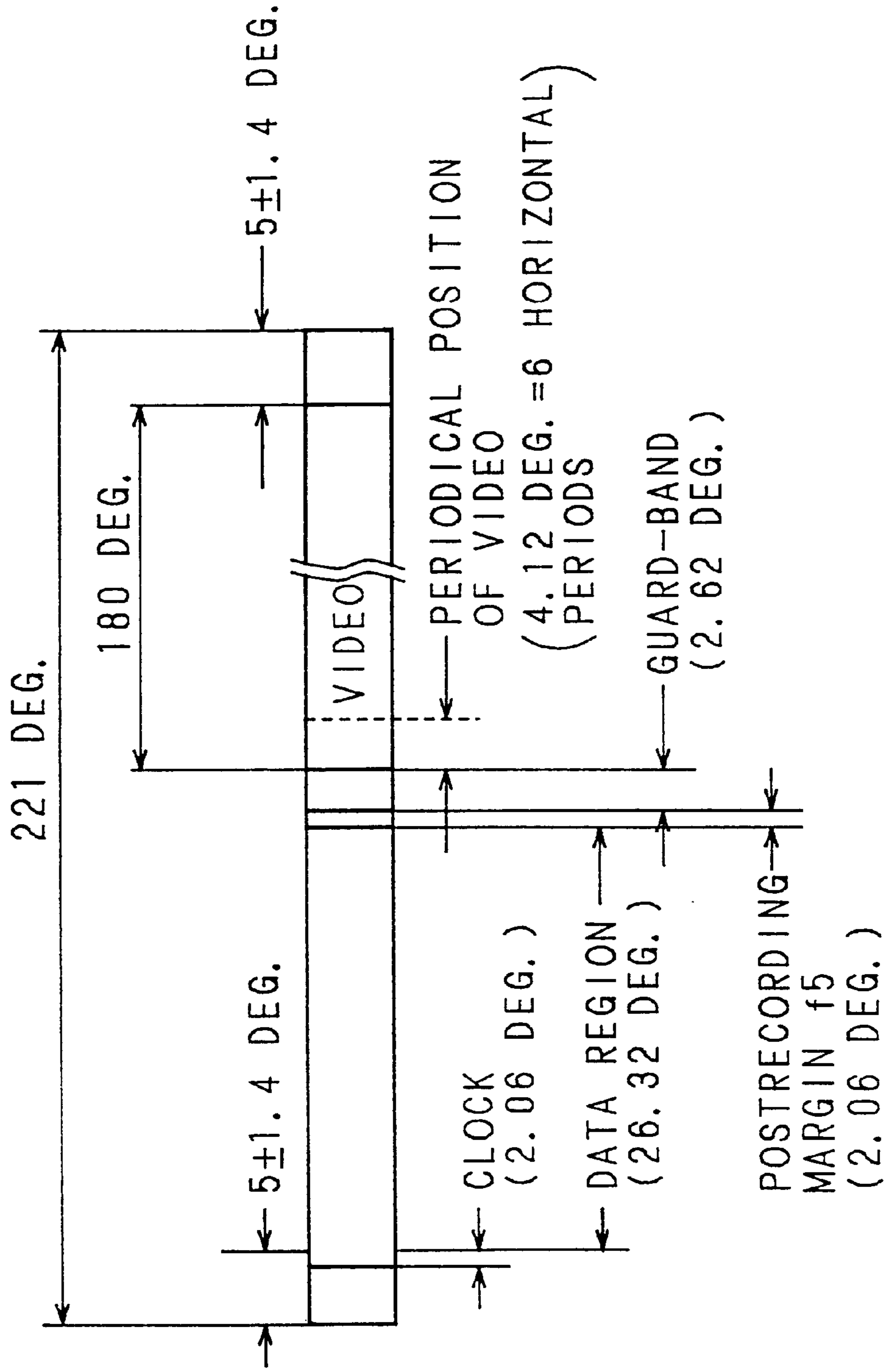
Fig. 10 Prior Art
