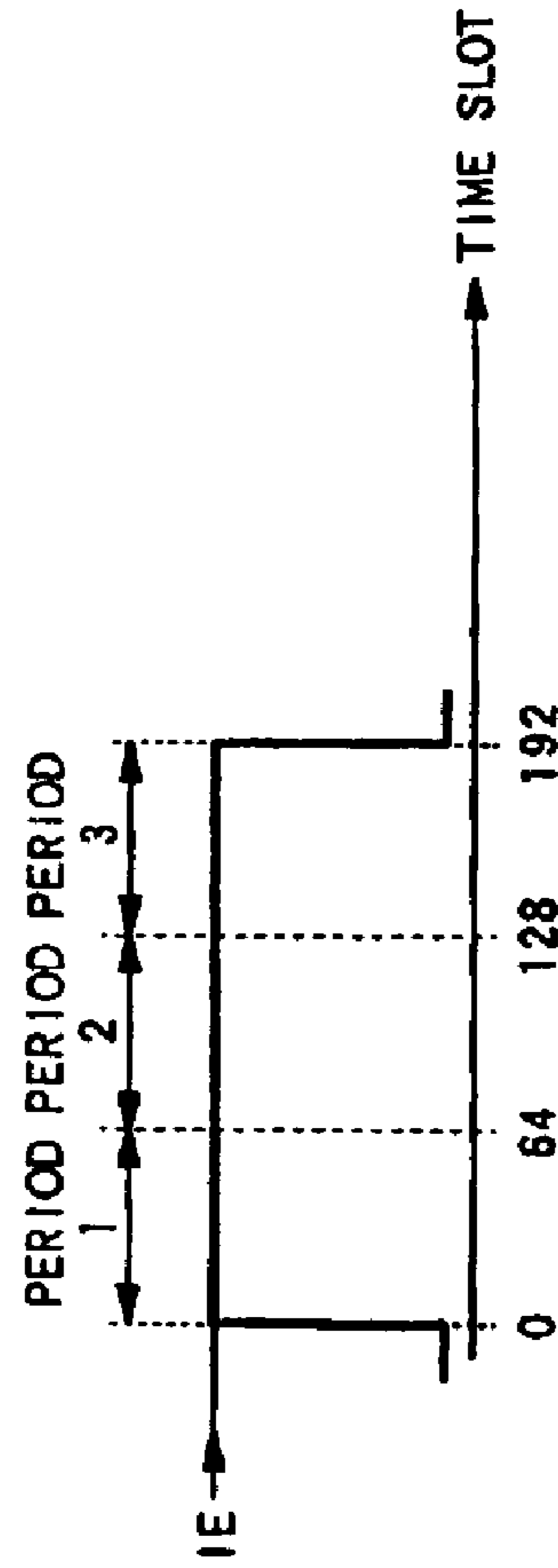
FIG. 11 A EMITTED CURRENT PULSE WHEN THERE IS NOT VOLTAGE DROP
