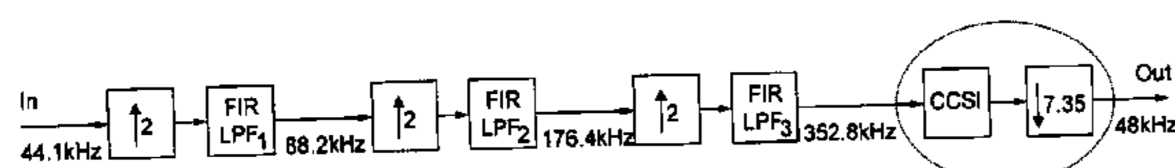
Typical architecture of the sampling rate converter in accordance with the present invention.
