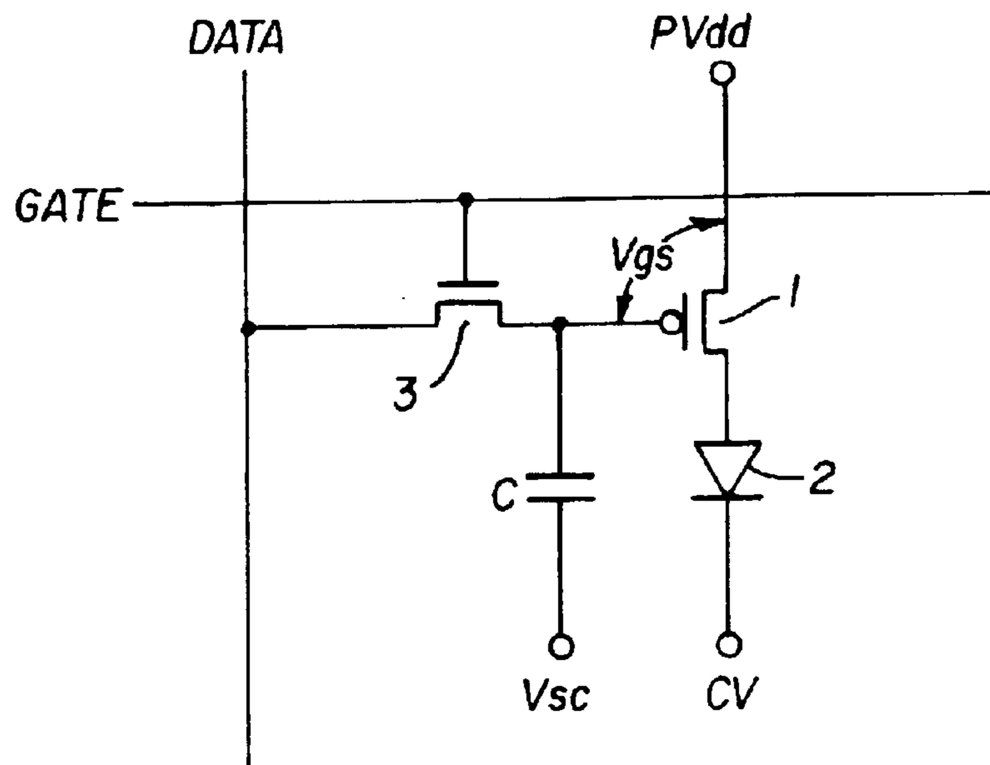
FIG. 1 (Prior Art)
