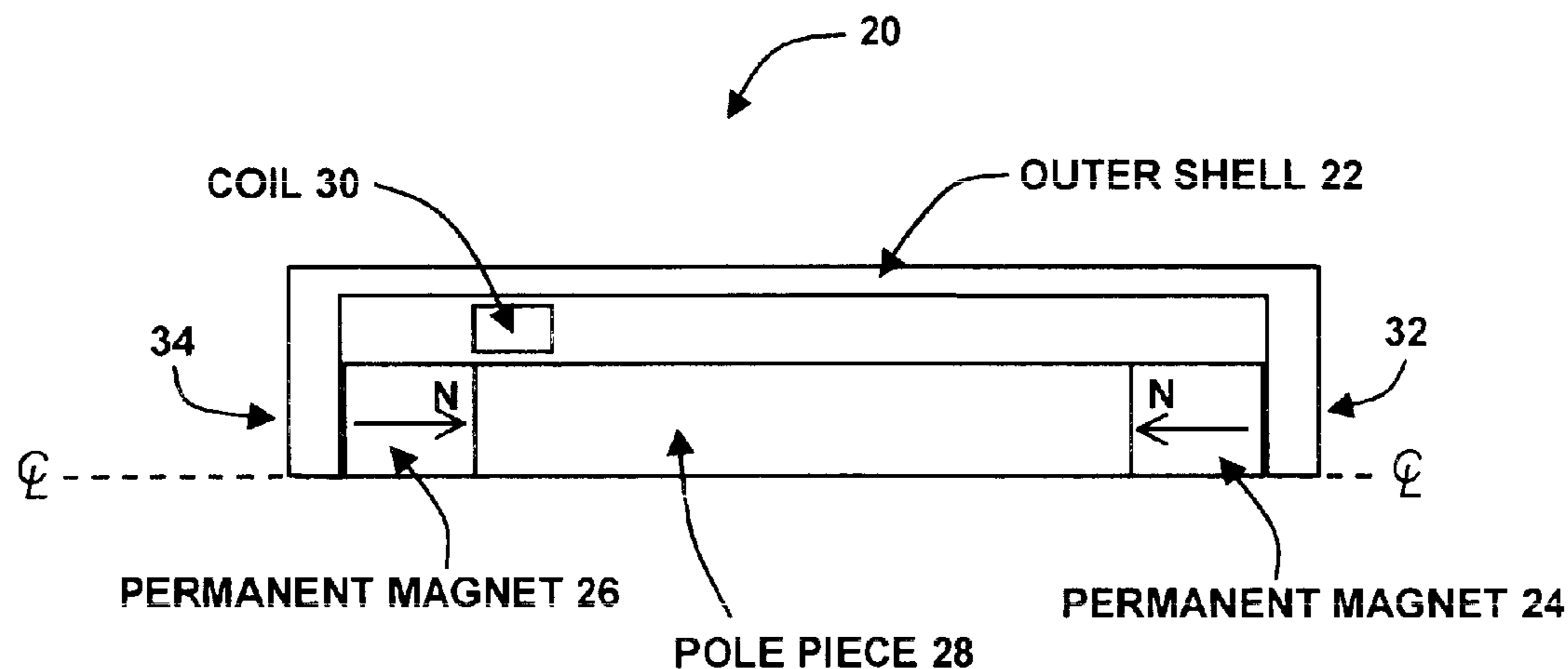
CLOSED-ENDED CYLINDRICAL ACTUATOR
