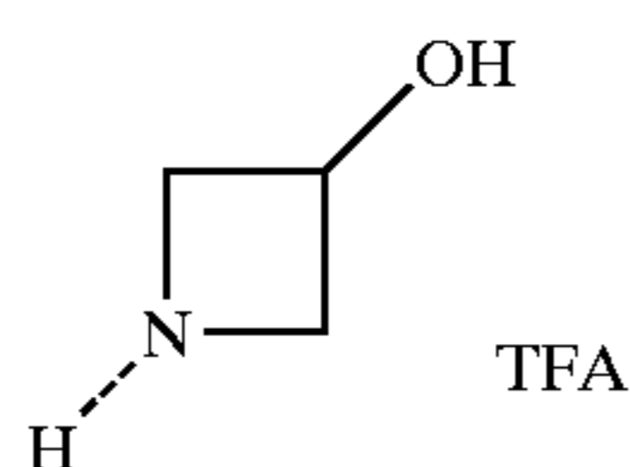
Example 9(c) Azetid-3-ol trifluoroacetic acid salt
