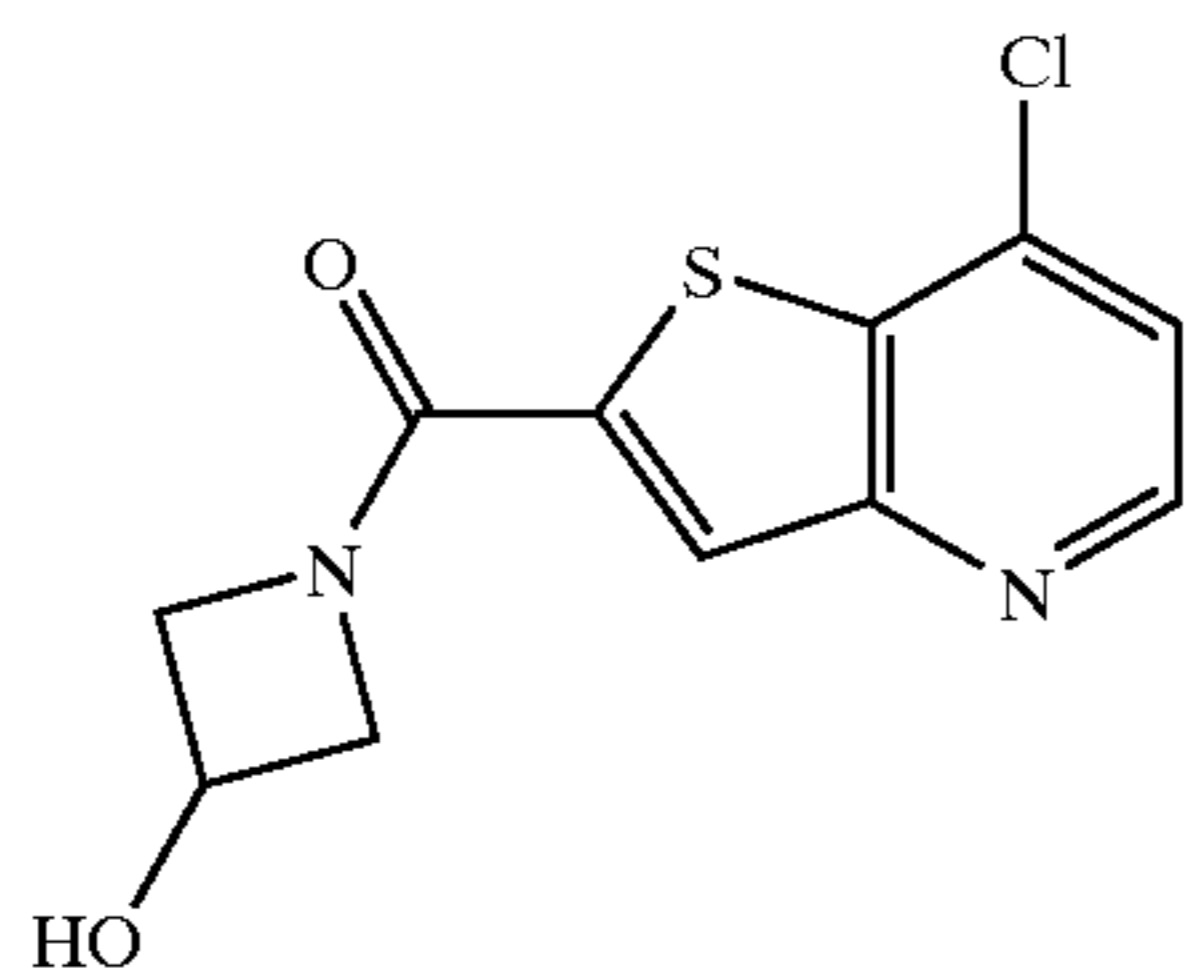
Example 9(d) 7-Chloro-2-[3-hydroxyazetid-1-carbonyl]thieno[3,2-b]pyridine
