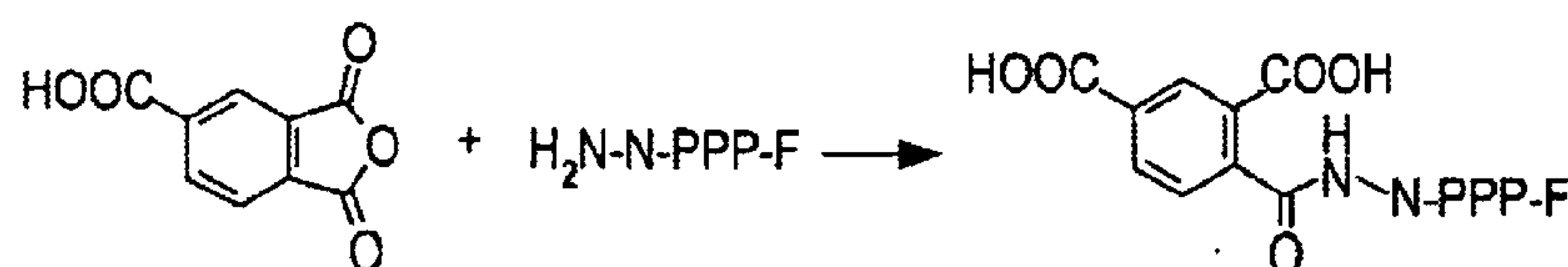
Scheme 10 - g-dNTP With Carboxylated Base
