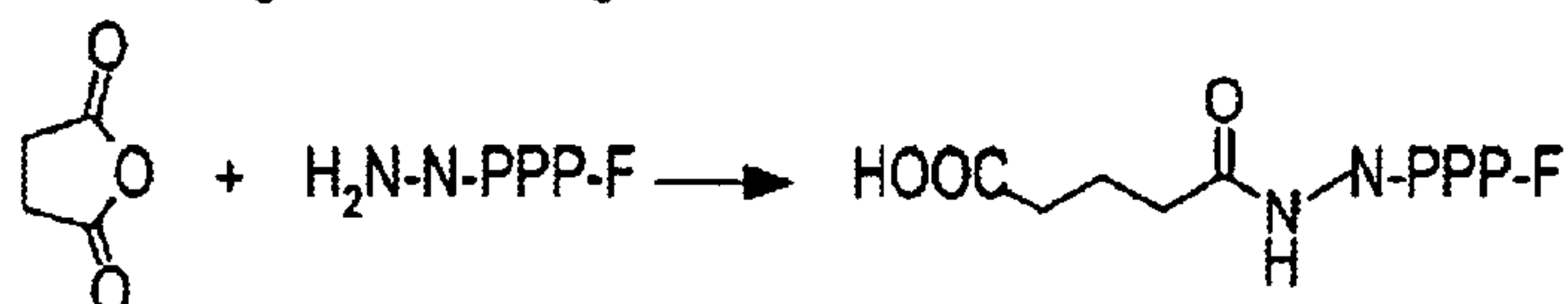
Scheme 9 - Add carboxylate to aminoallyl-dUTP
