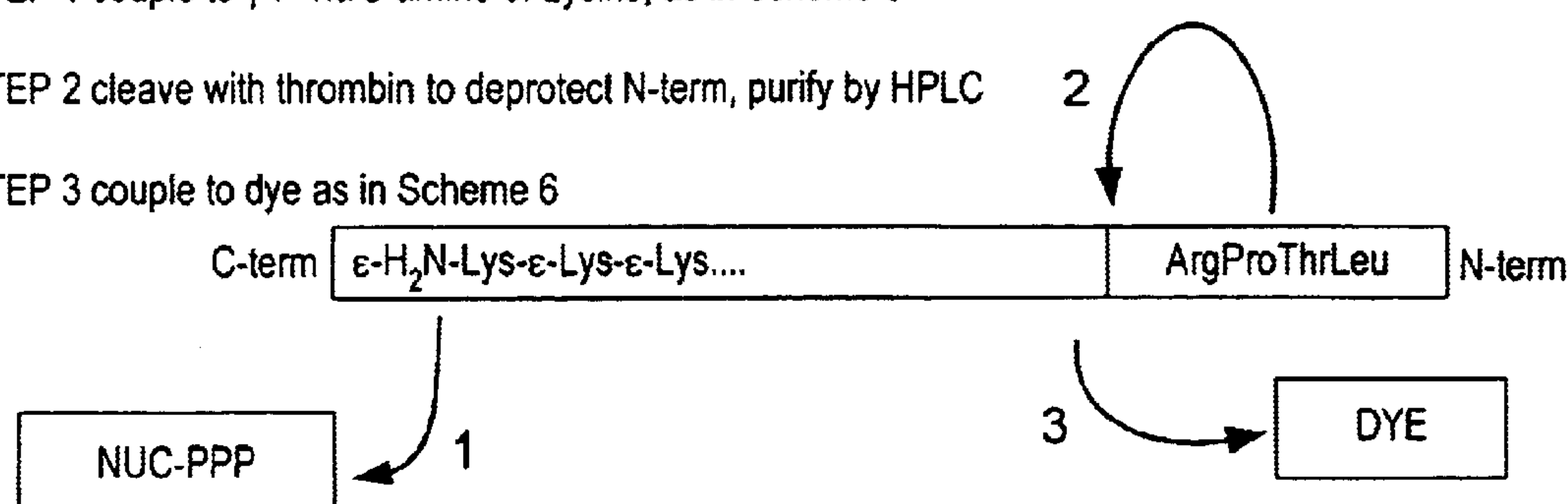
Scheme 8 - Peptide Deprotection By Thrombin Cleavage
