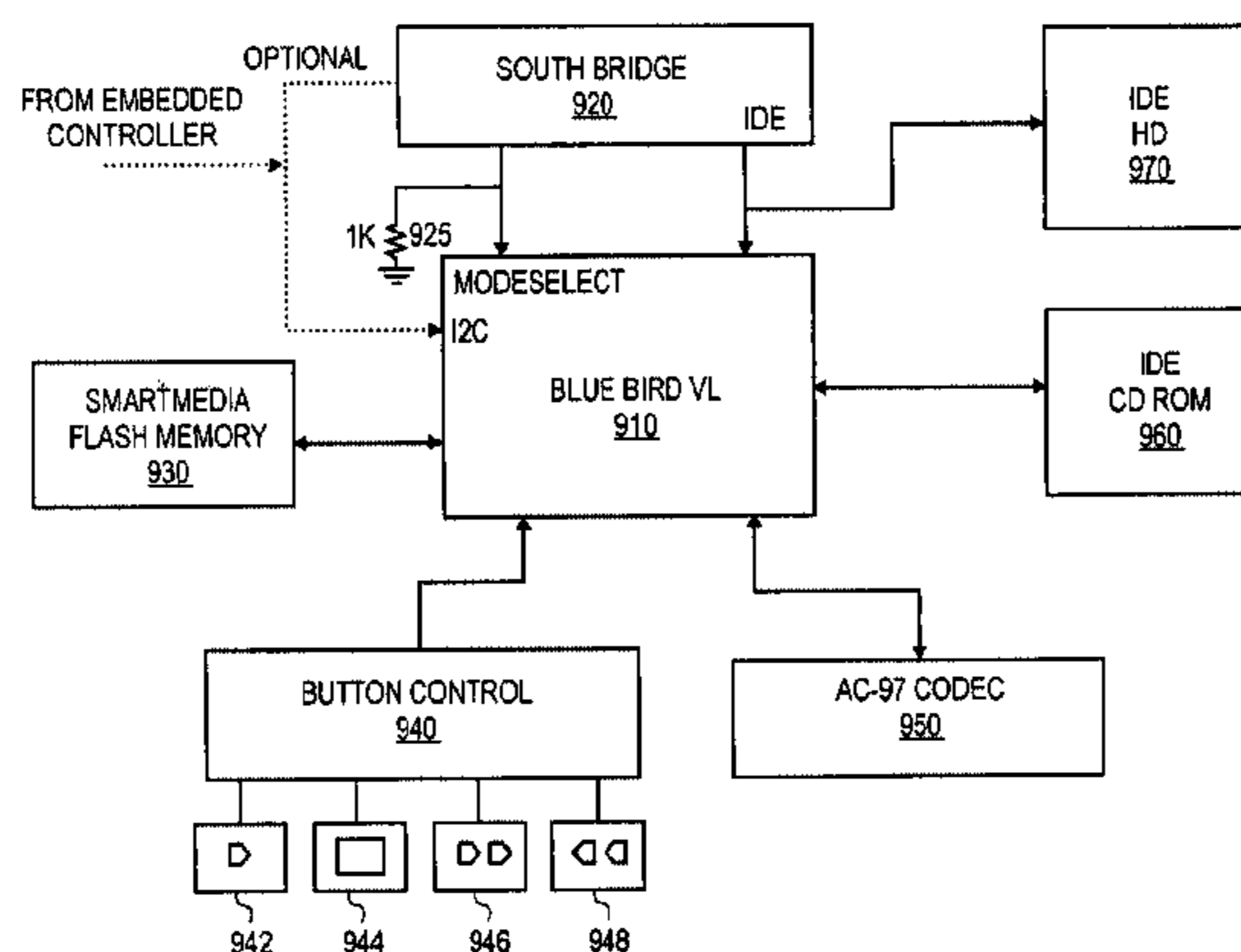
BlueBirdVL Notebook Implementation
