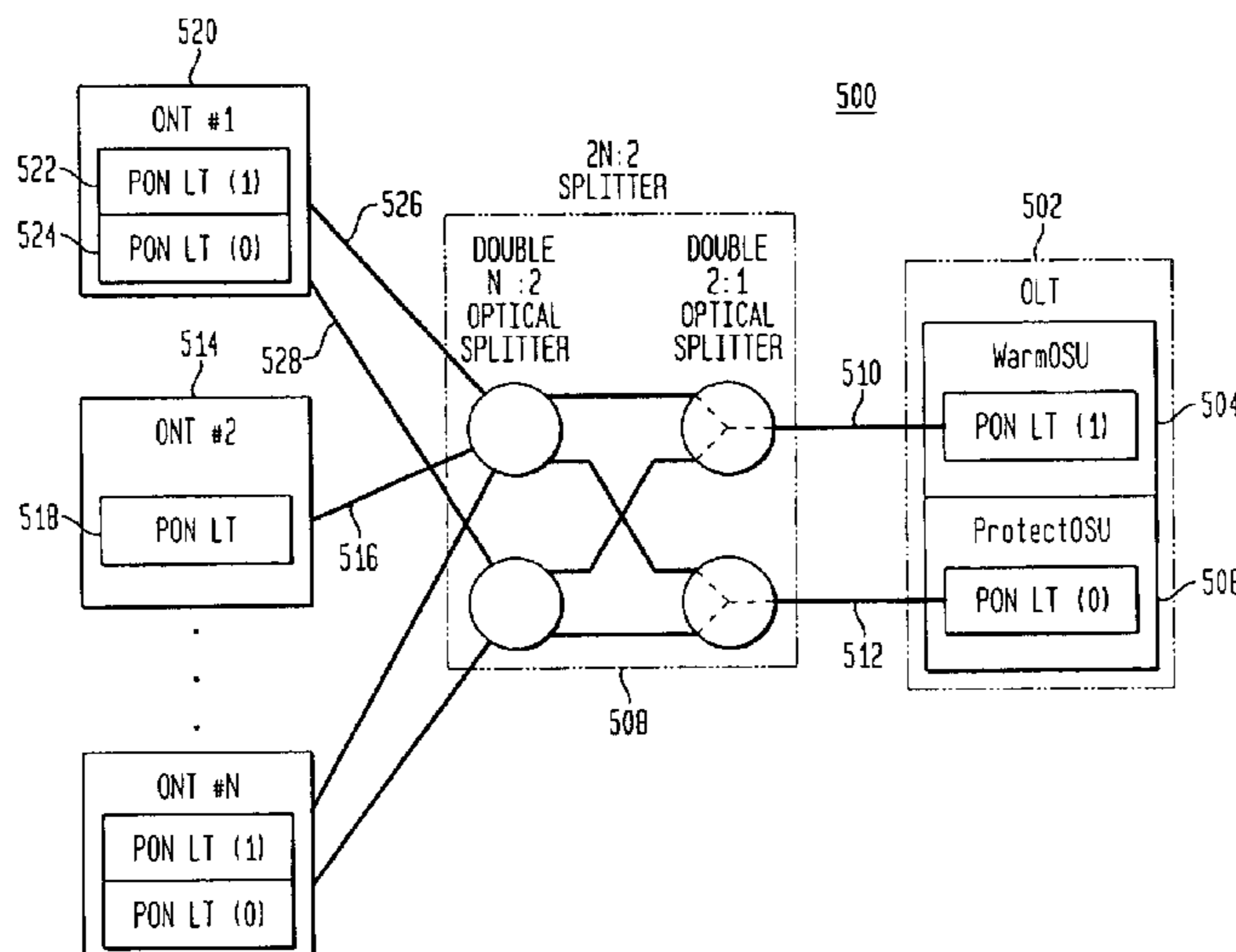
PARTIAL DUPLEX SYSTEM
