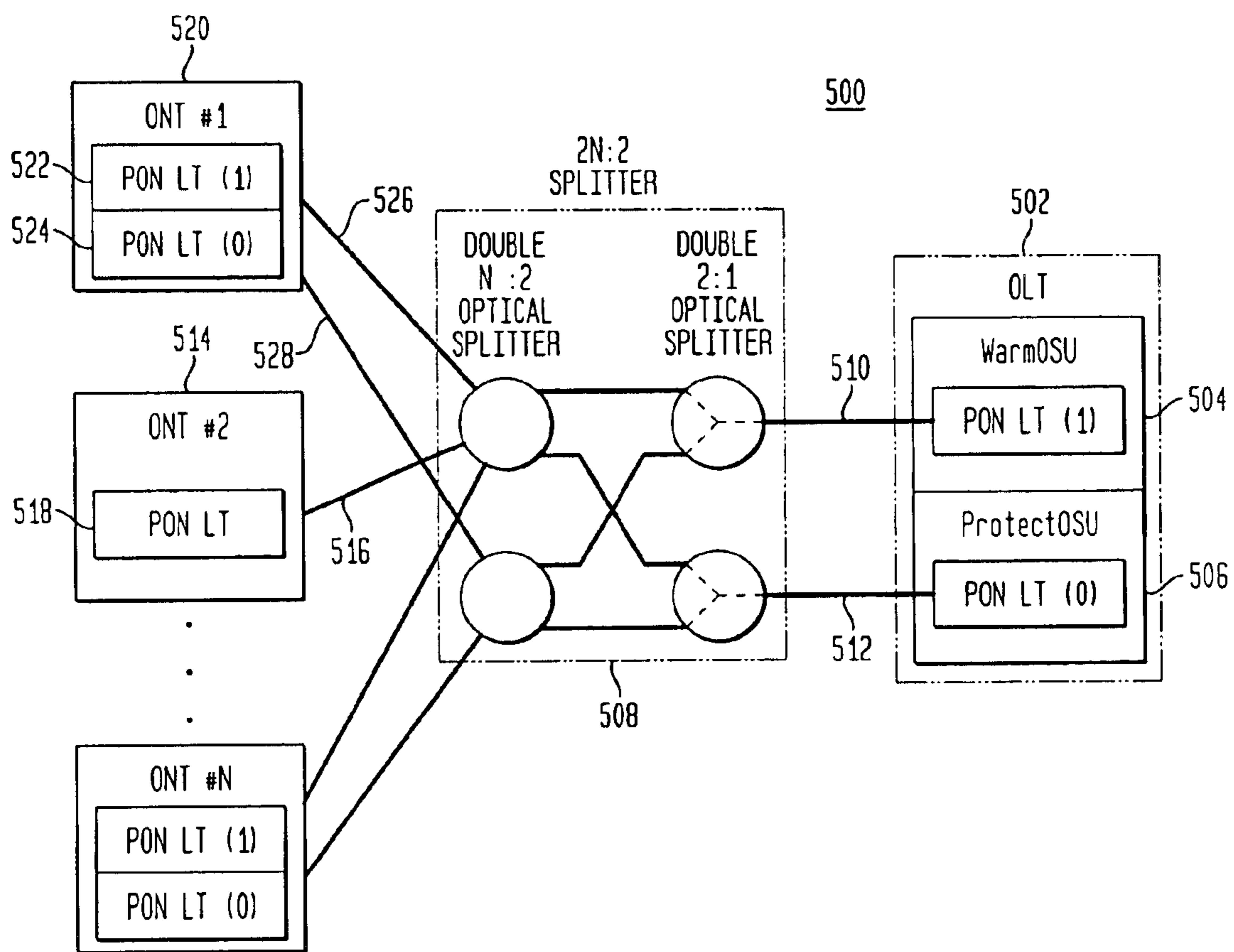
PARTIAL DUPLEX SYSTEM
