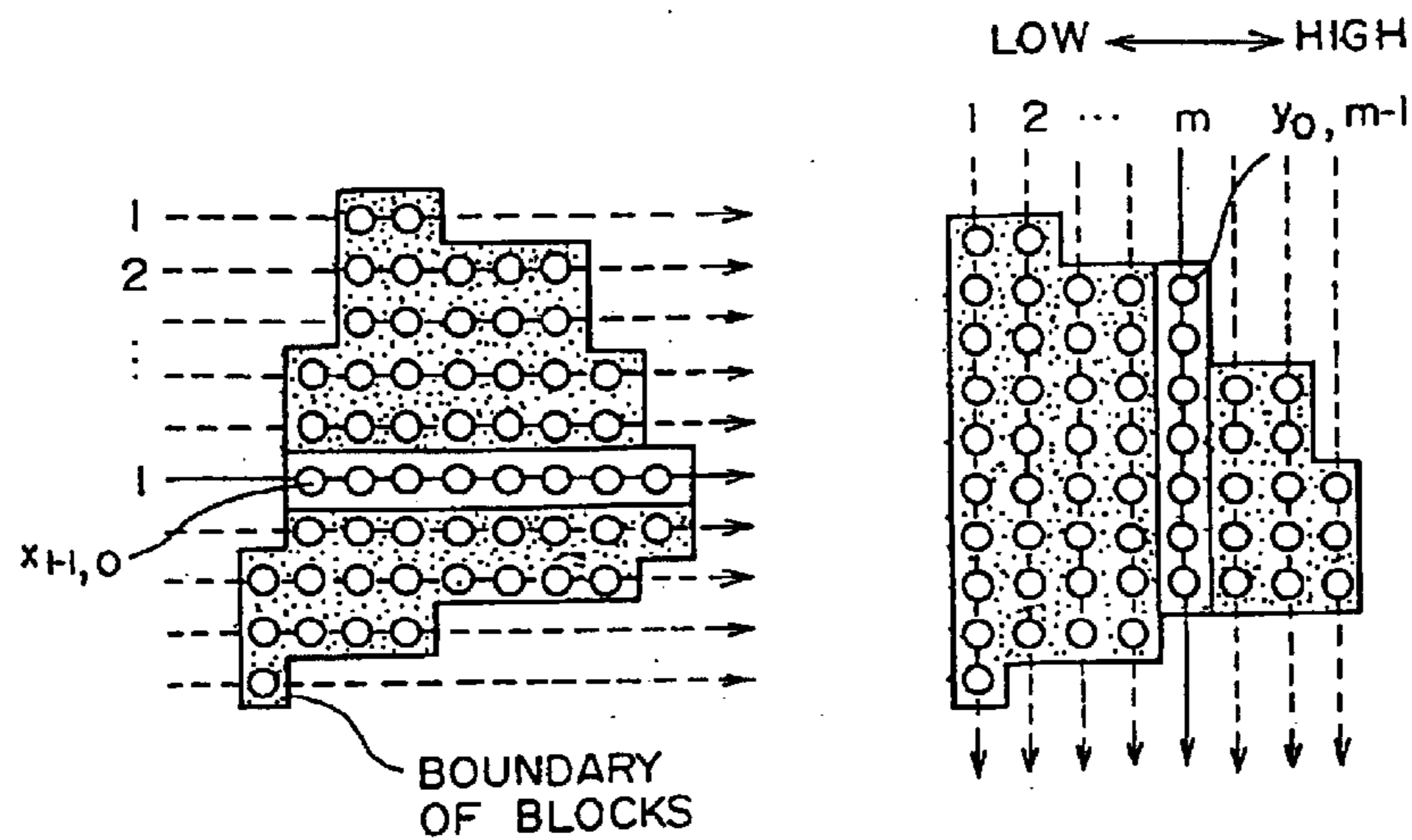
FIG. 58(b) PRIOR ART
