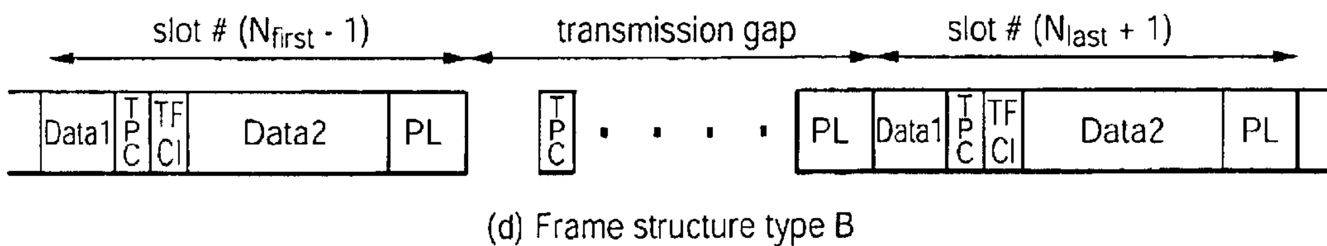
Frame structure types in downlink compressed transmission
