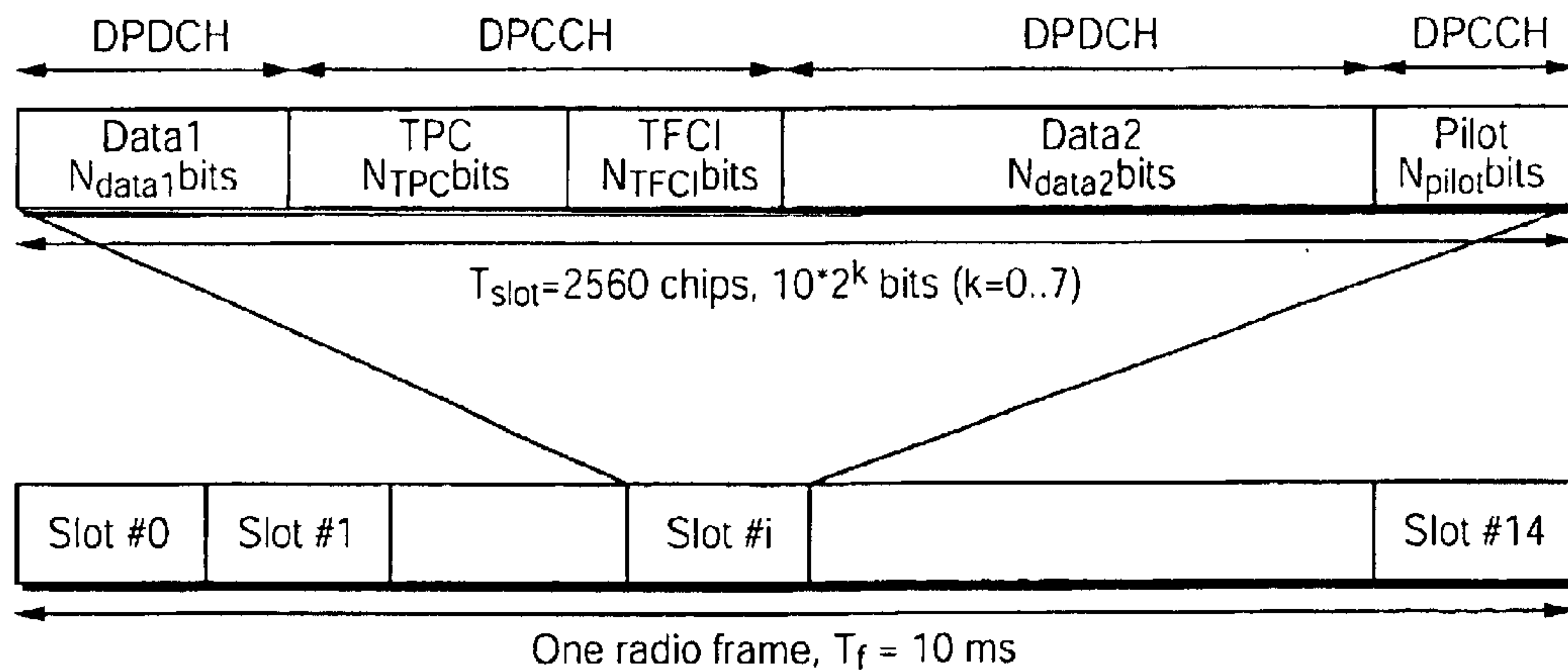
Frame structure for downlink DPCH
