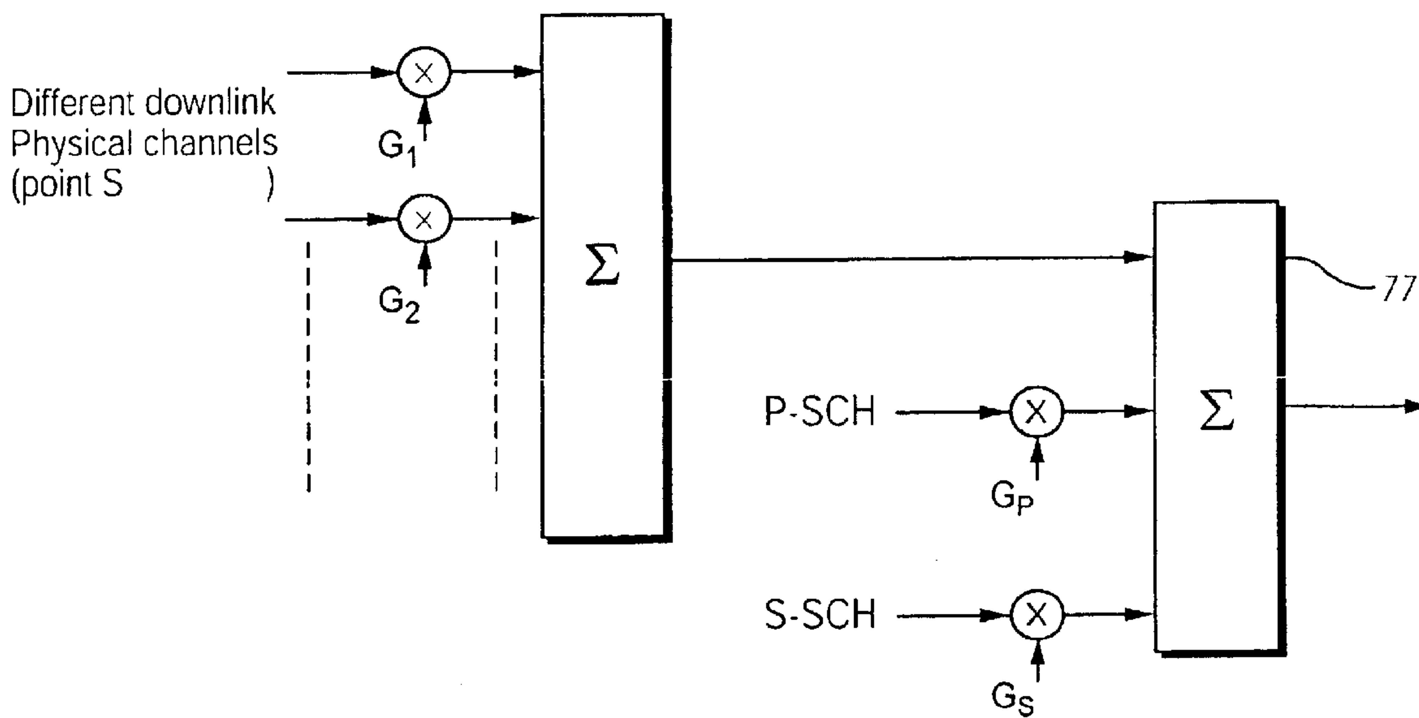
Spreading and modulation for SCH and P-CCPCH
