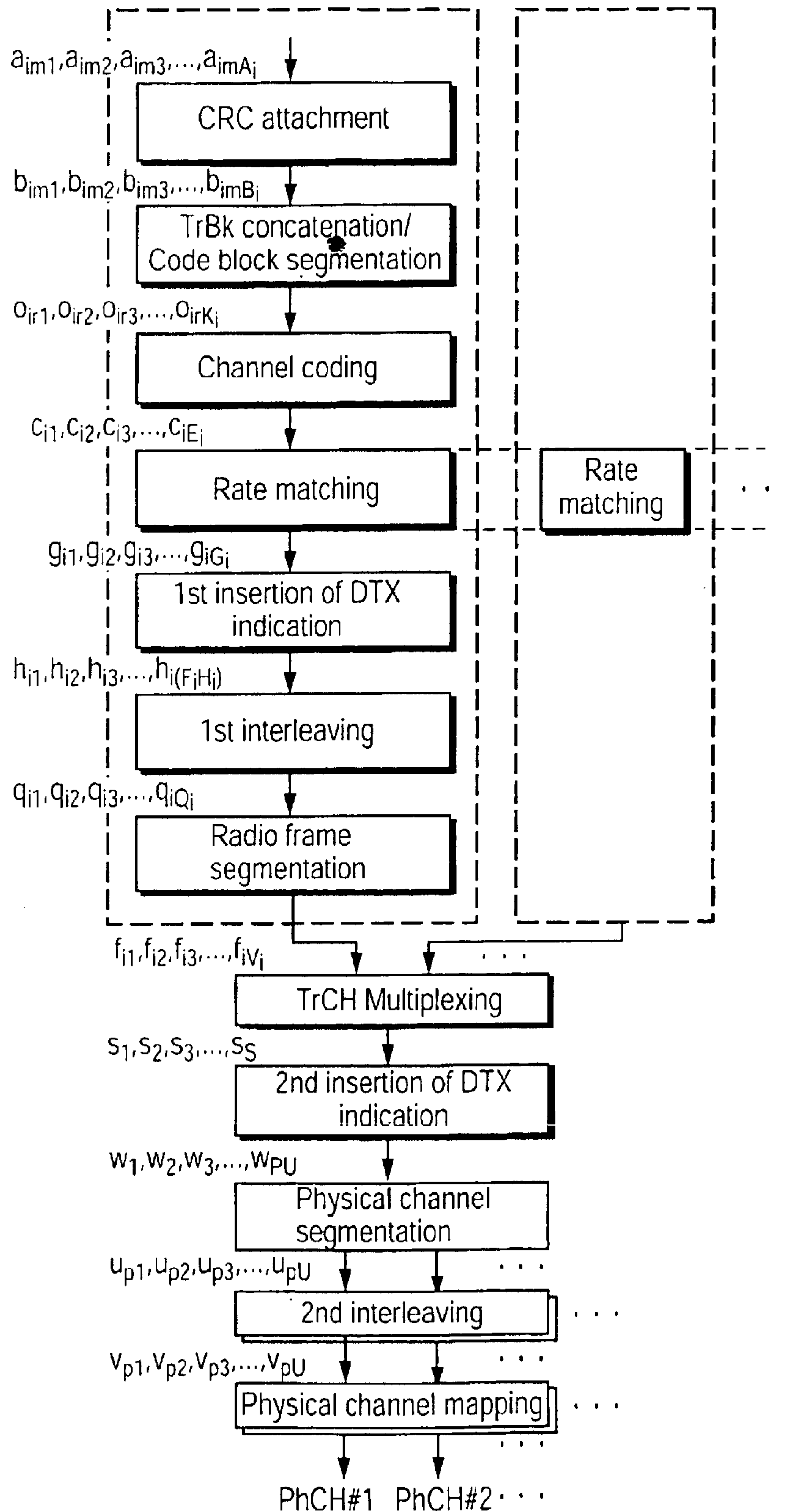
Transport channel multiplexing structure for downlink
