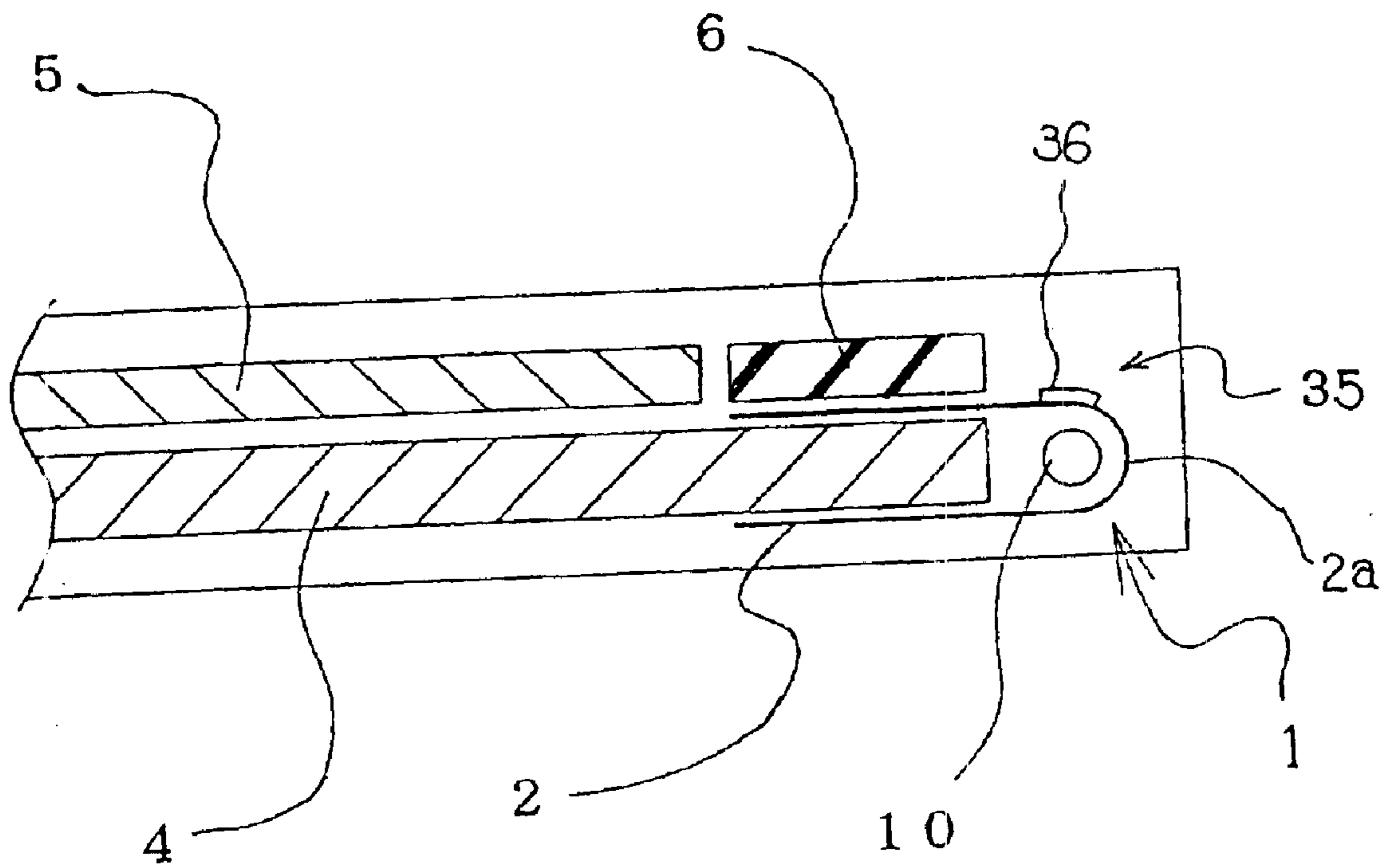
Fig. 6 PRIOR ART
