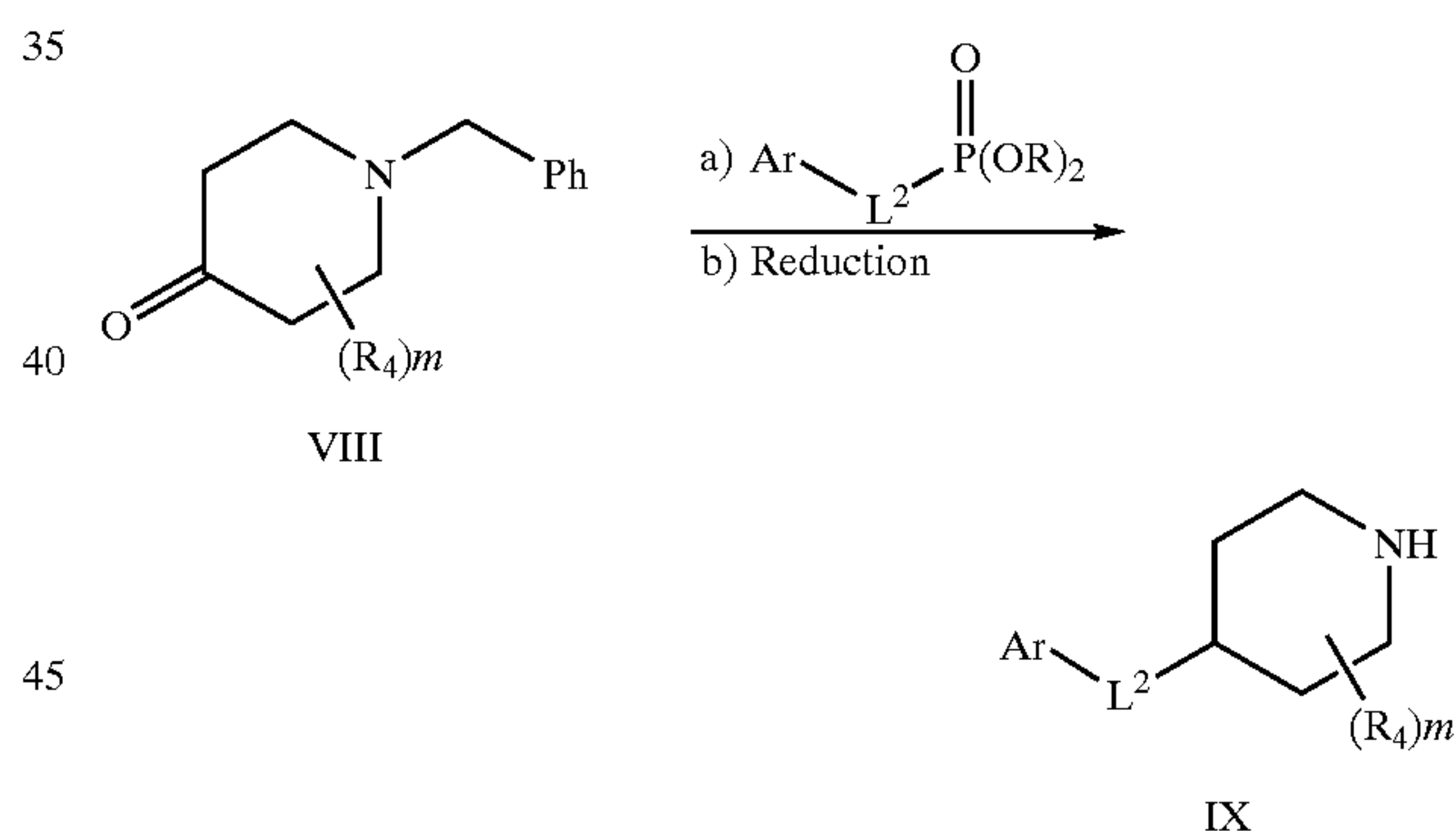
Scheme 4
