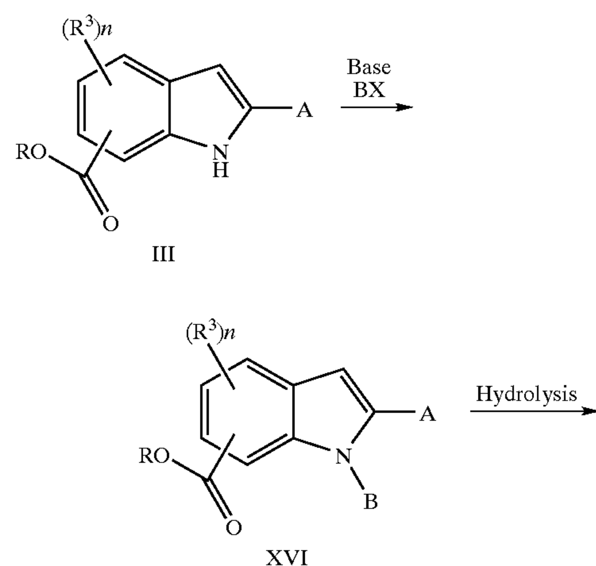
Scheme 7
