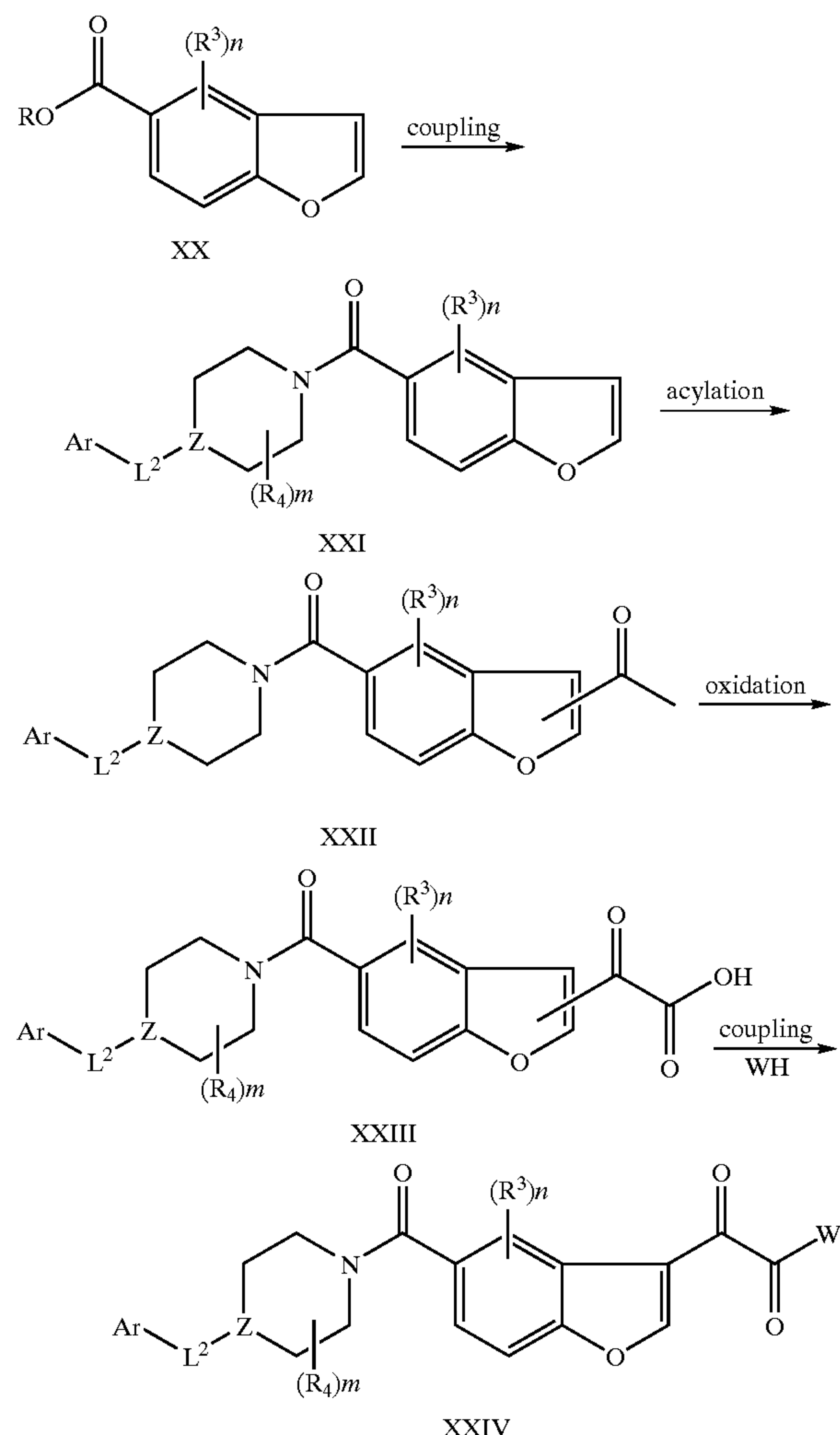
Scheme 9
