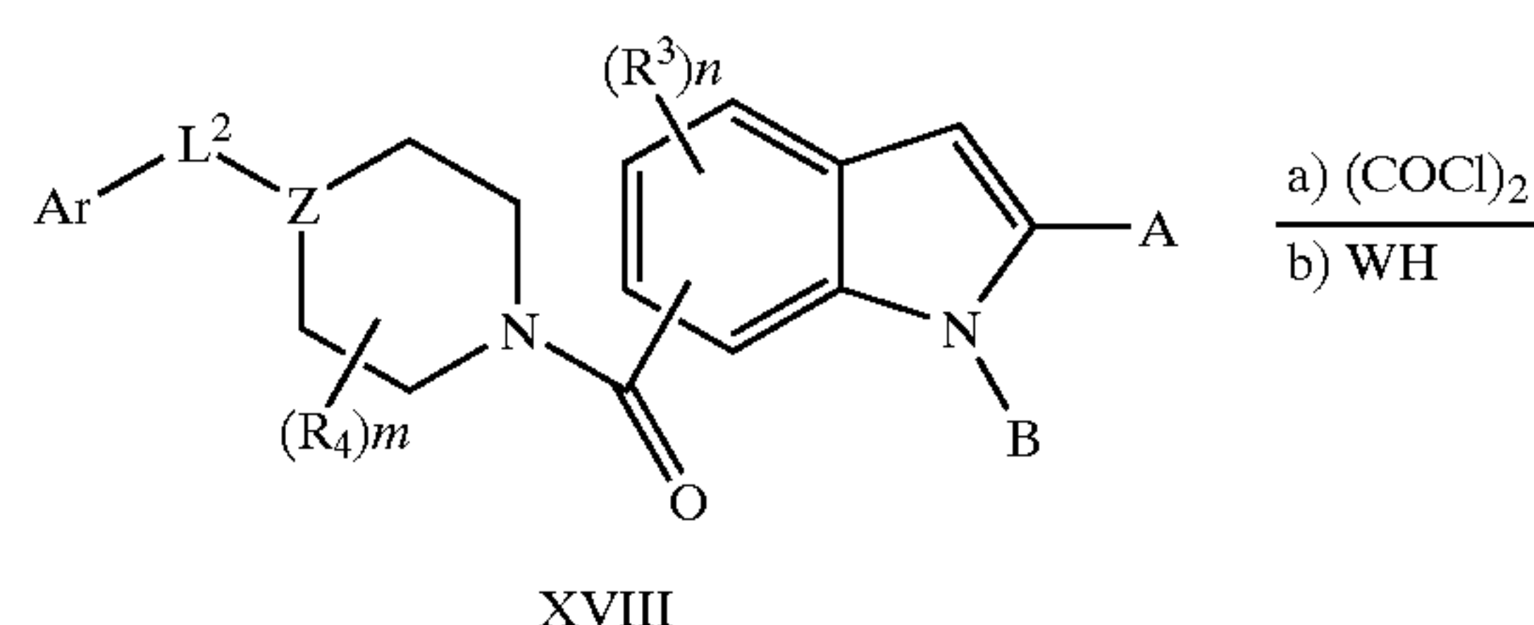
Scheme 8
