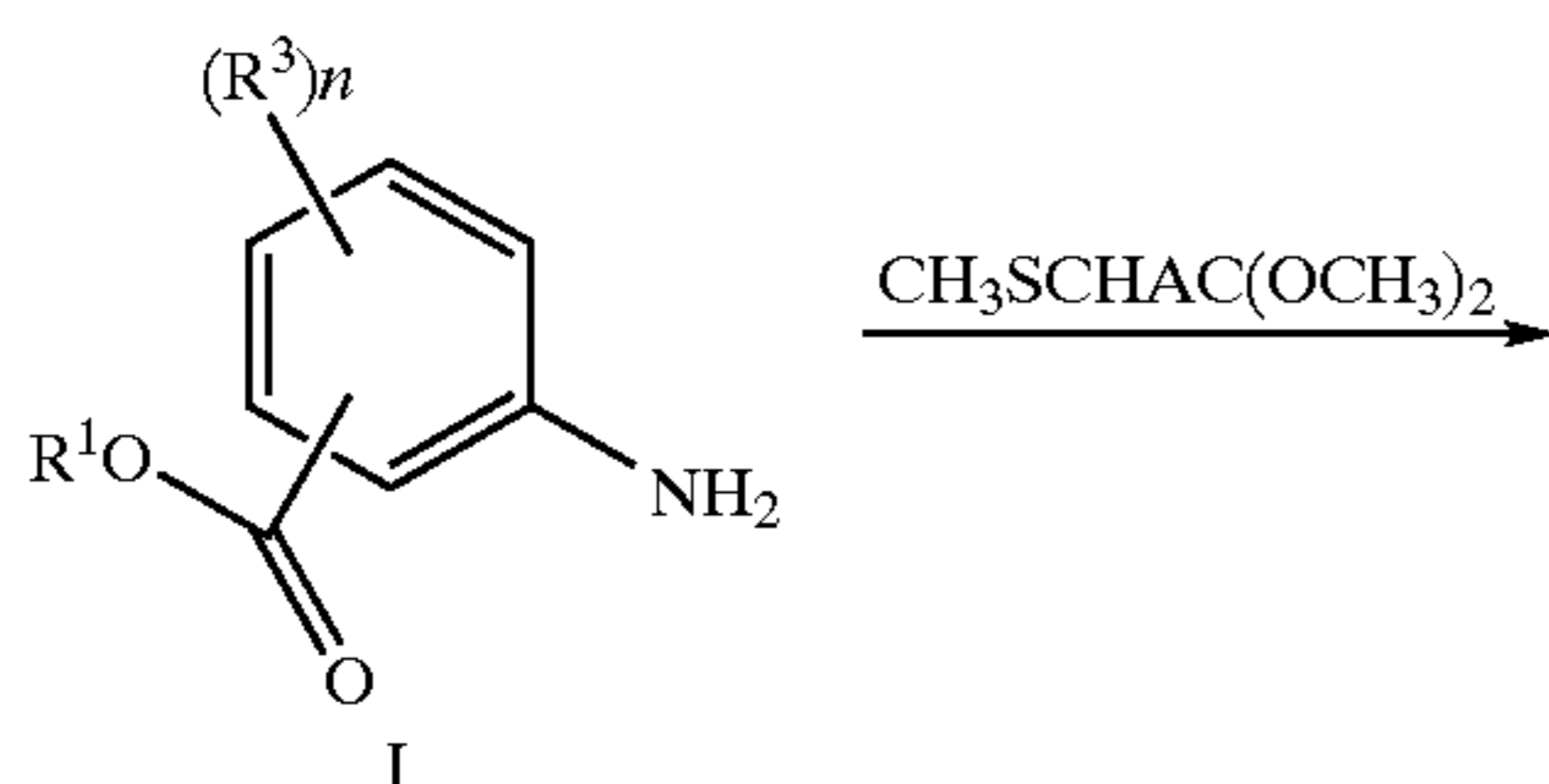
Scheme 1
