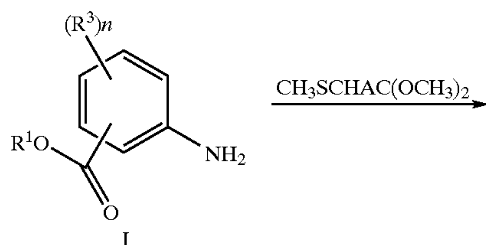
Scheme 1
