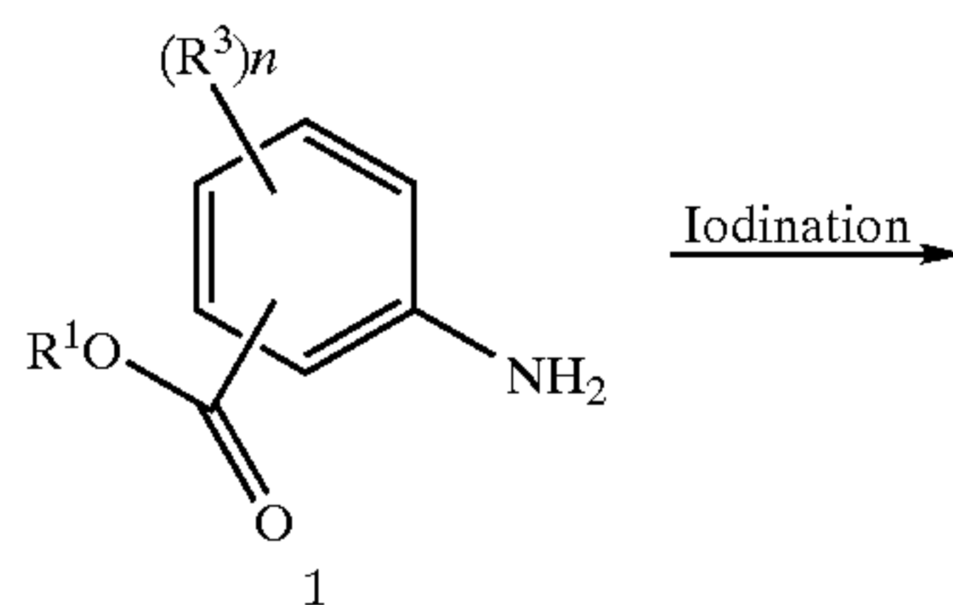
Scheme 3
