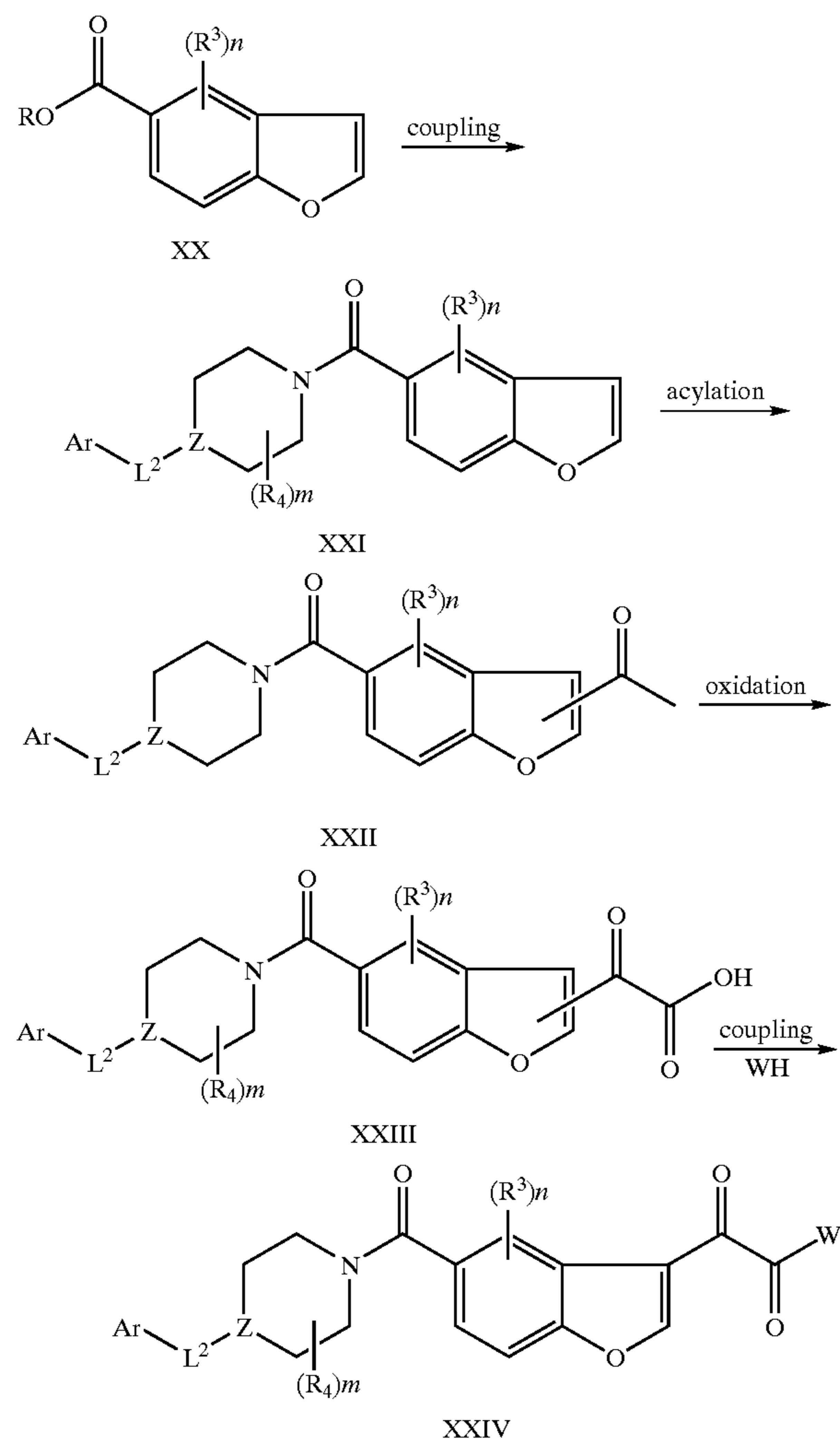
Scheme 9
