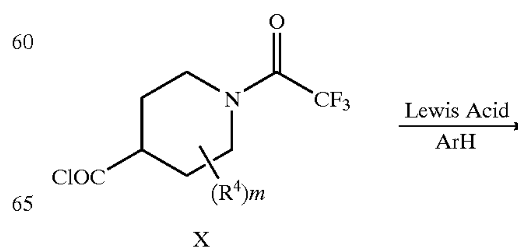
Scheme 5
