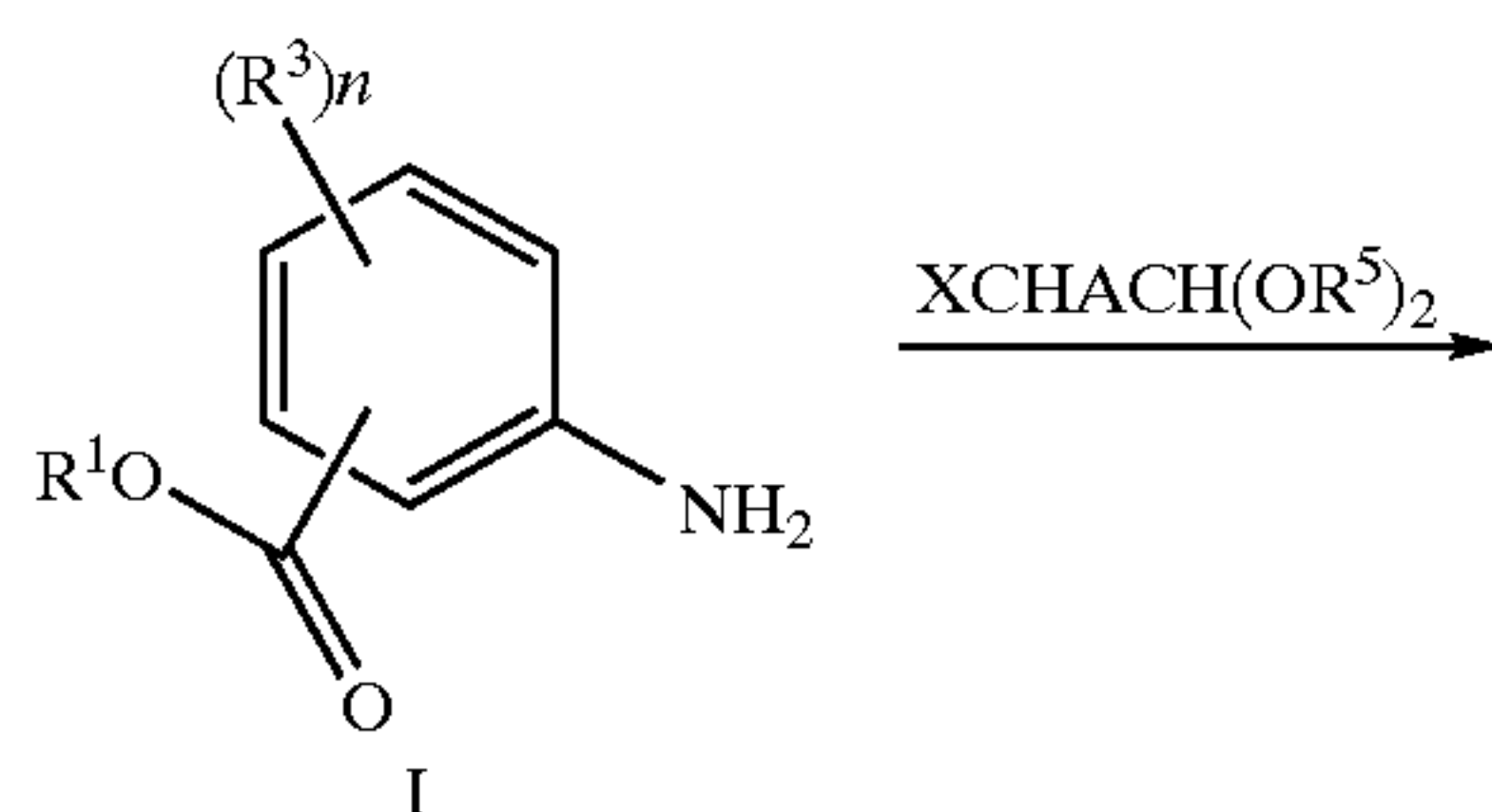
Scheme 2
