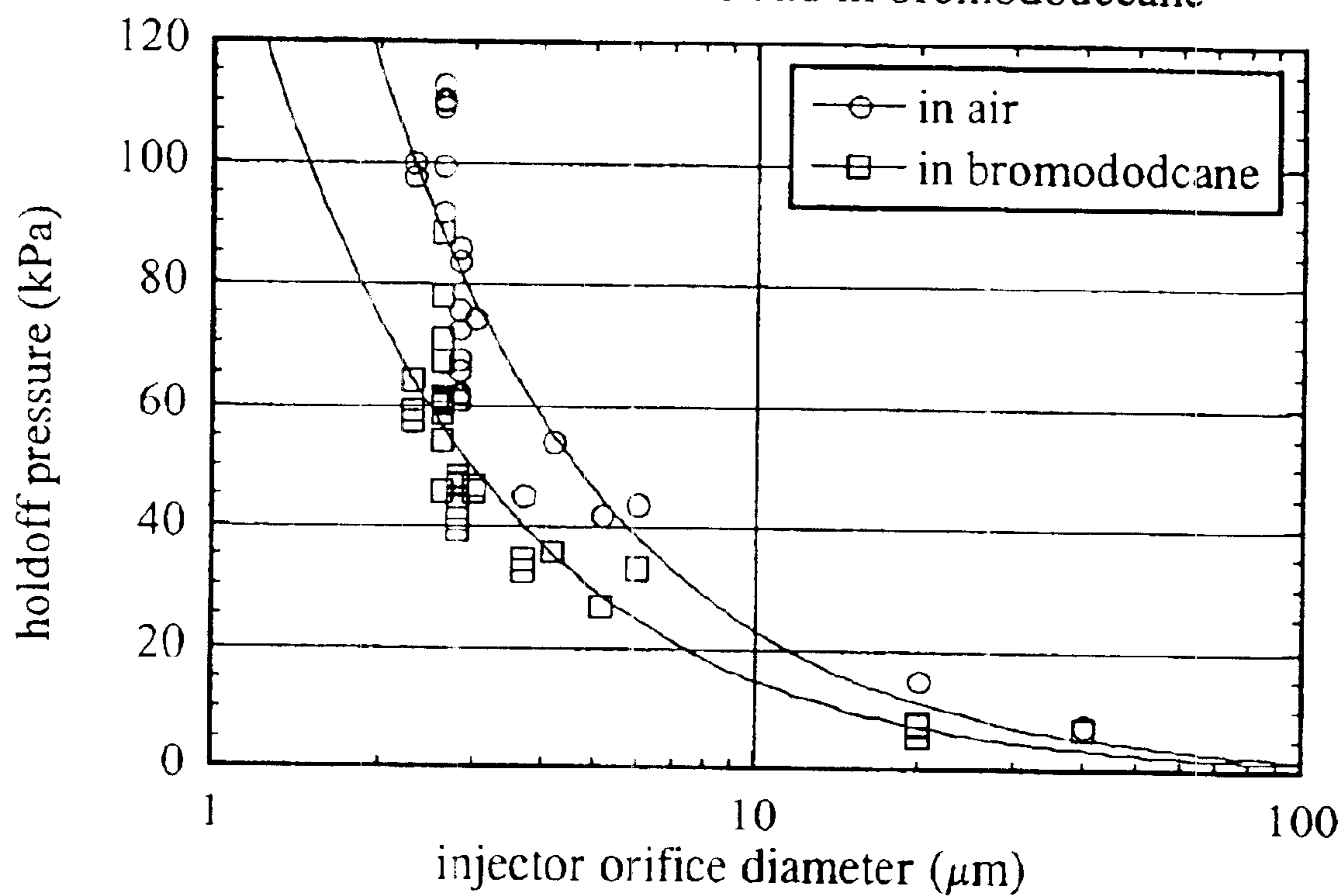
Pressure to eject 3 \times H_2O droplets from injectors of various diameters in air and in bromododecane
