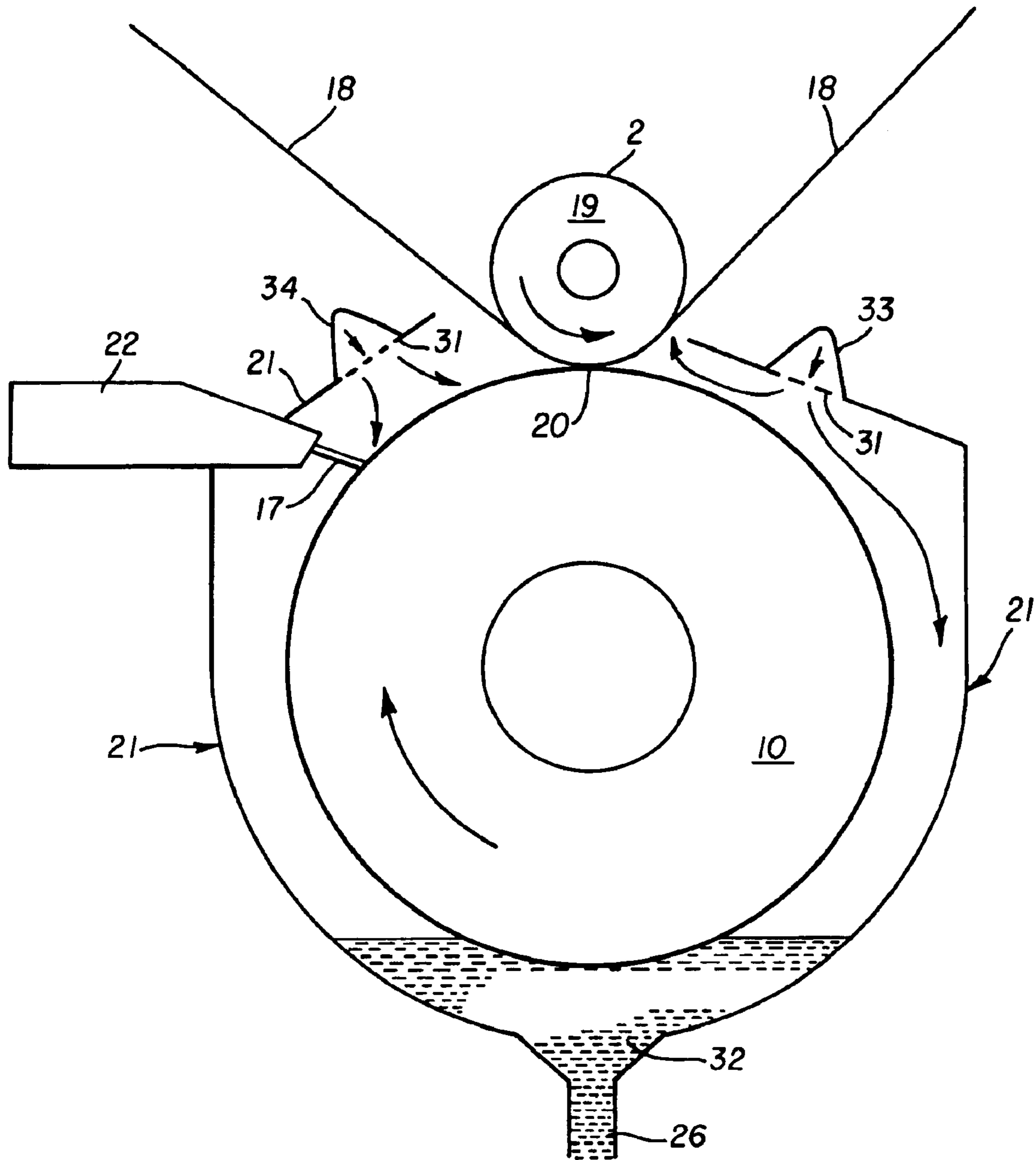
FIG. 1 (Prior Art)
