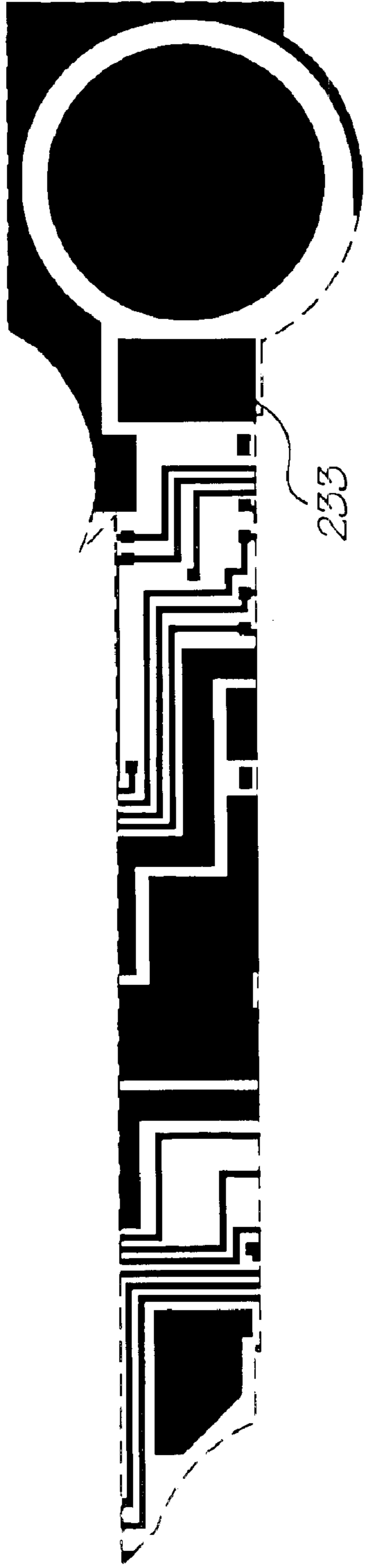
Metal 2 mask
