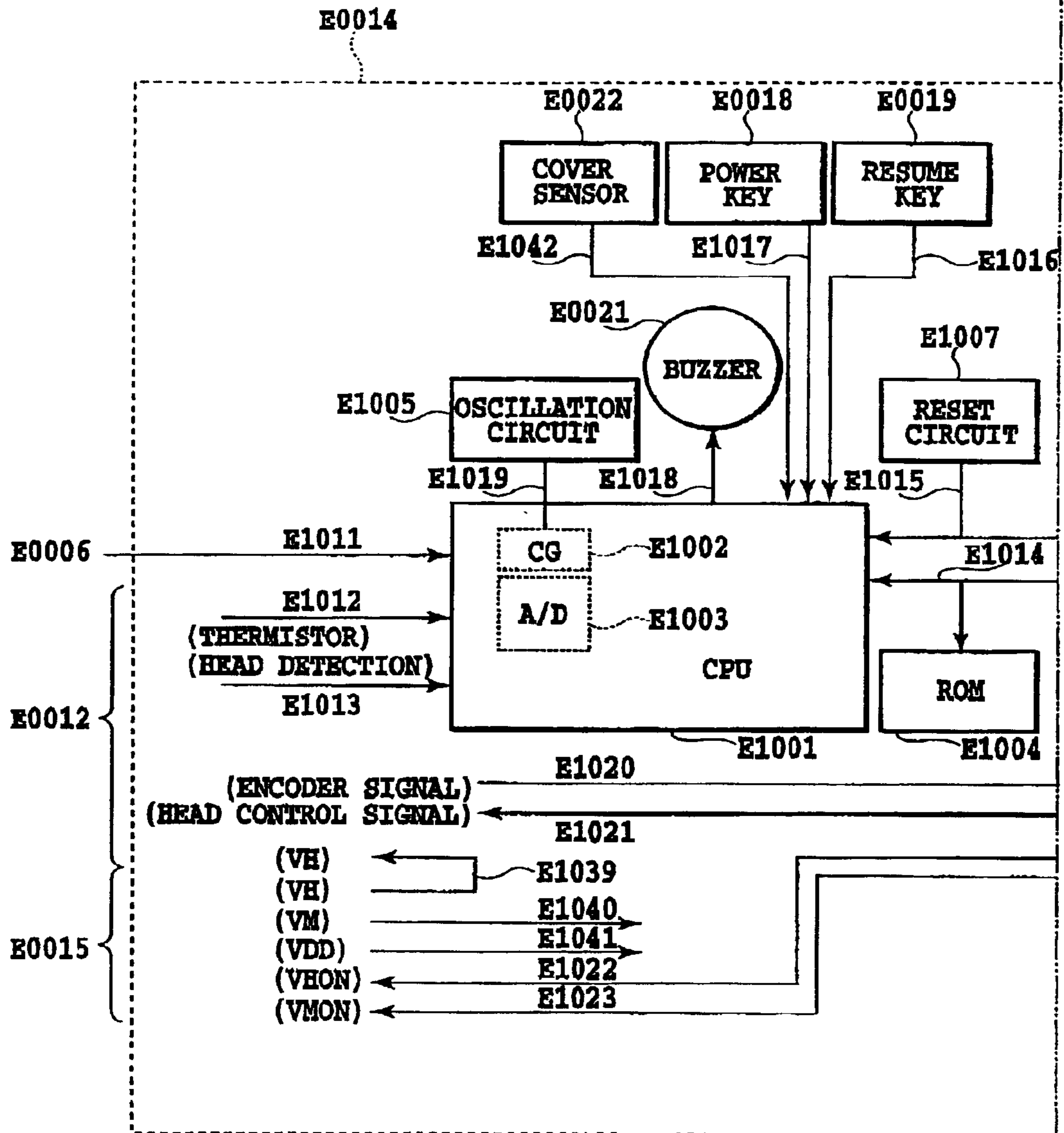
FIG.8A
