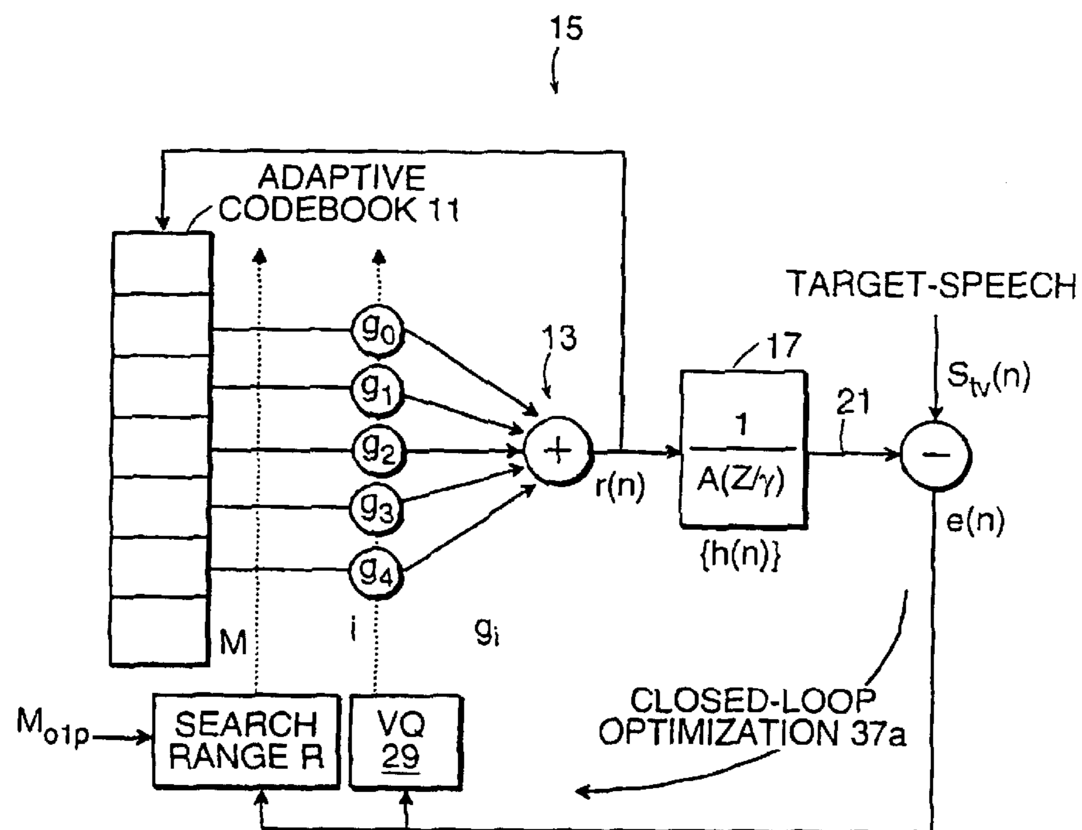
MULTI-TAP PITCH PREDICTOR VQ
