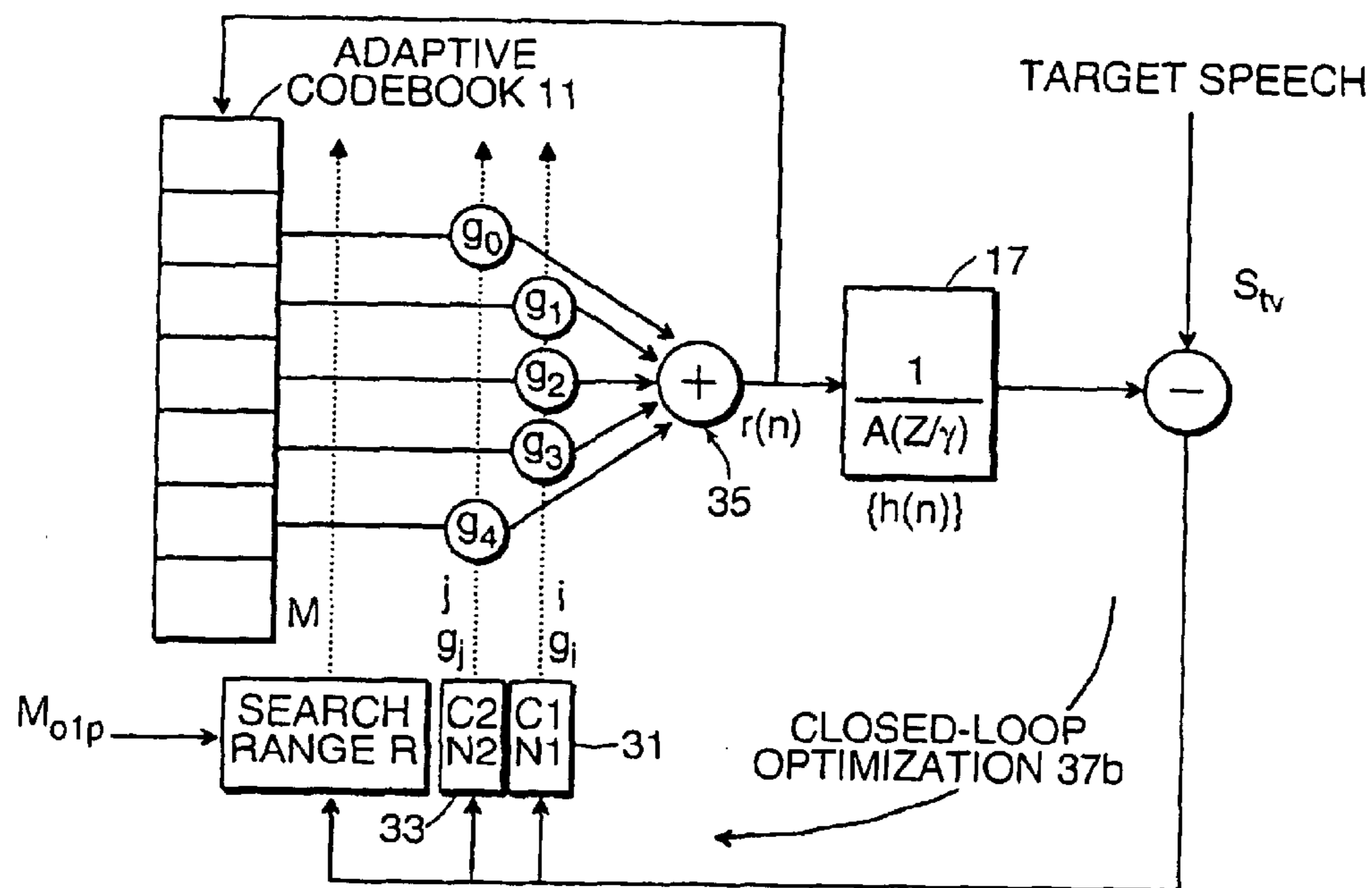
MULTI-TAP PITCH PREDICTOR PRODUCT VQ
