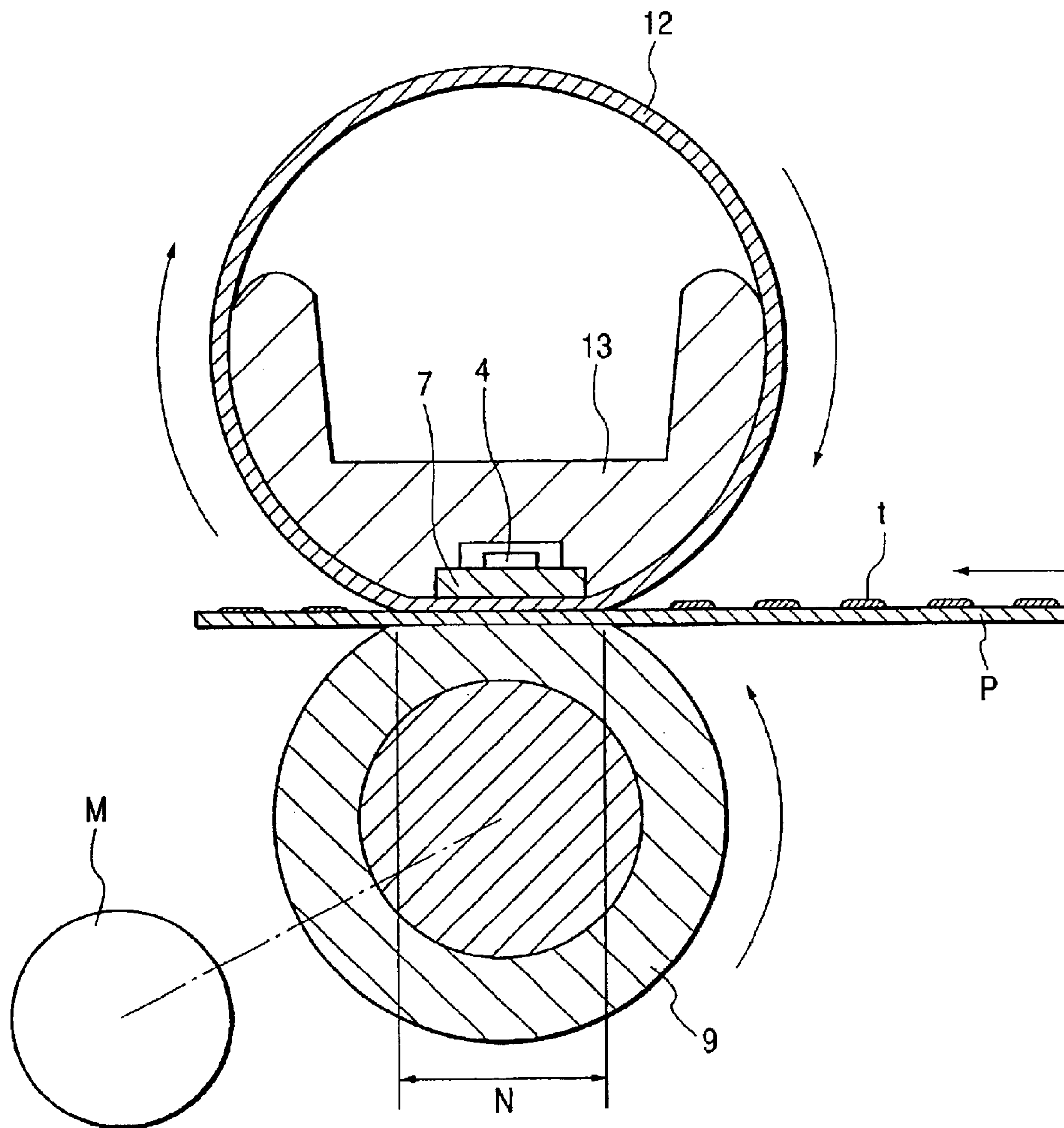
FIG. 6 PRIOR ART
