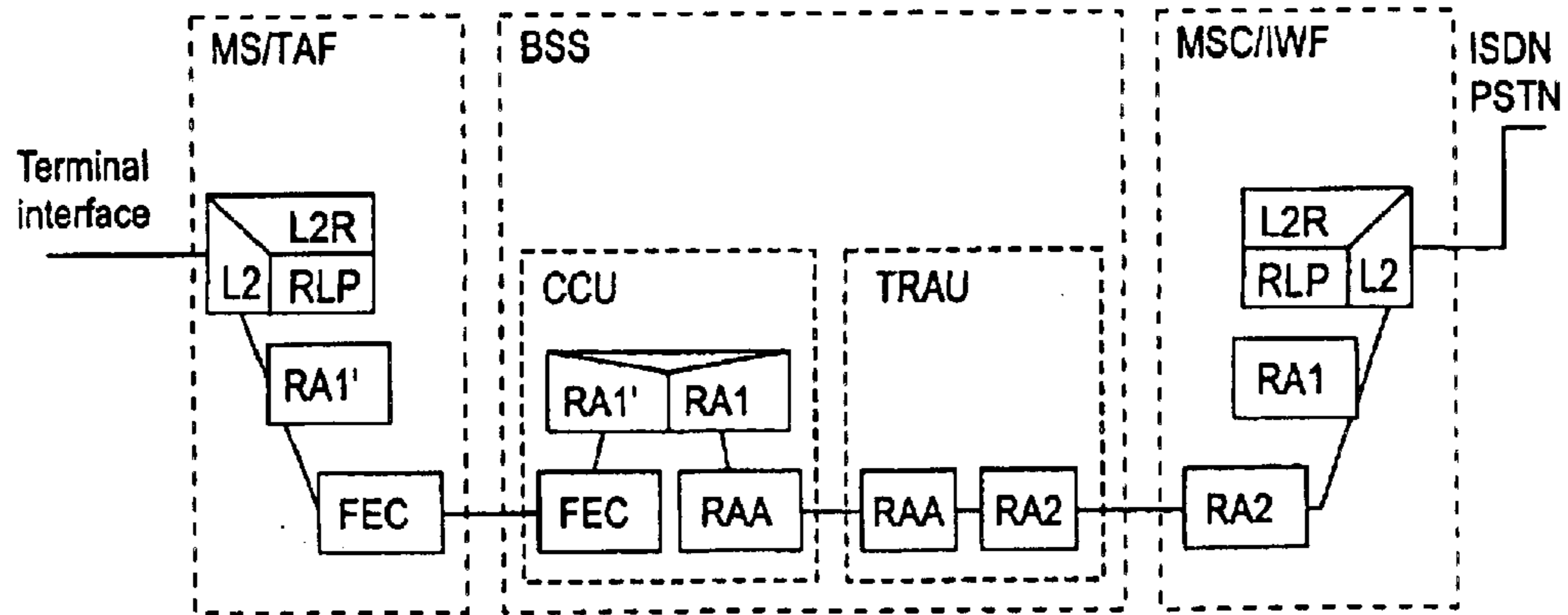
Fig. 3 (Prior art)
