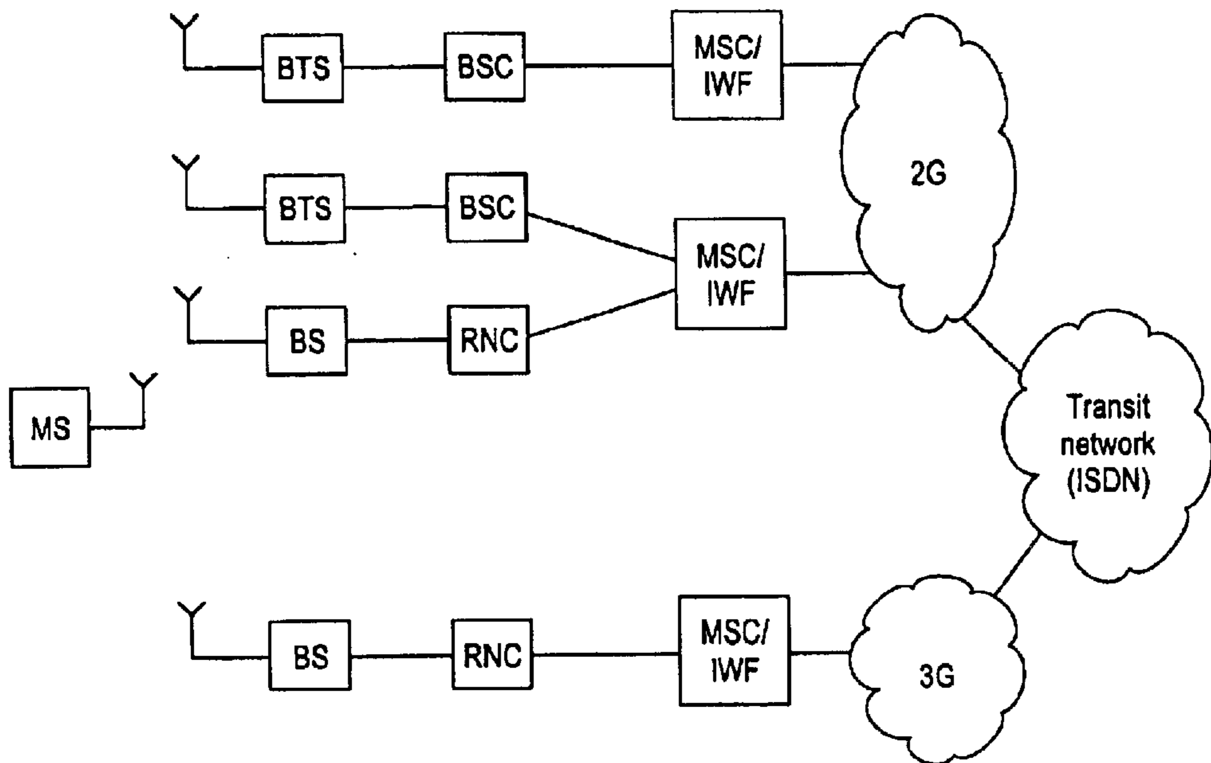
Fig. 3 (Prior art)
