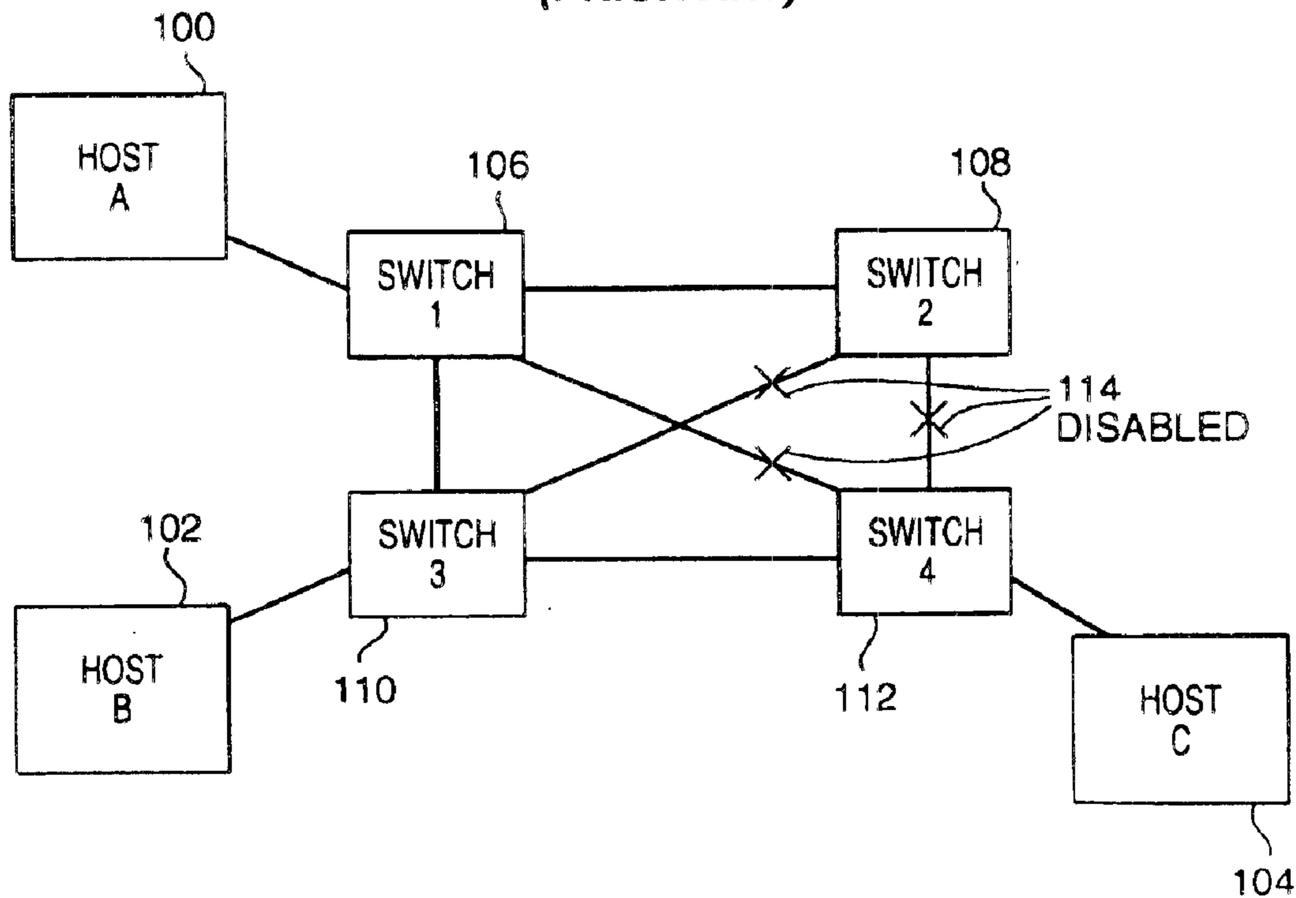
FIG. 2 (PRIOR ART)
