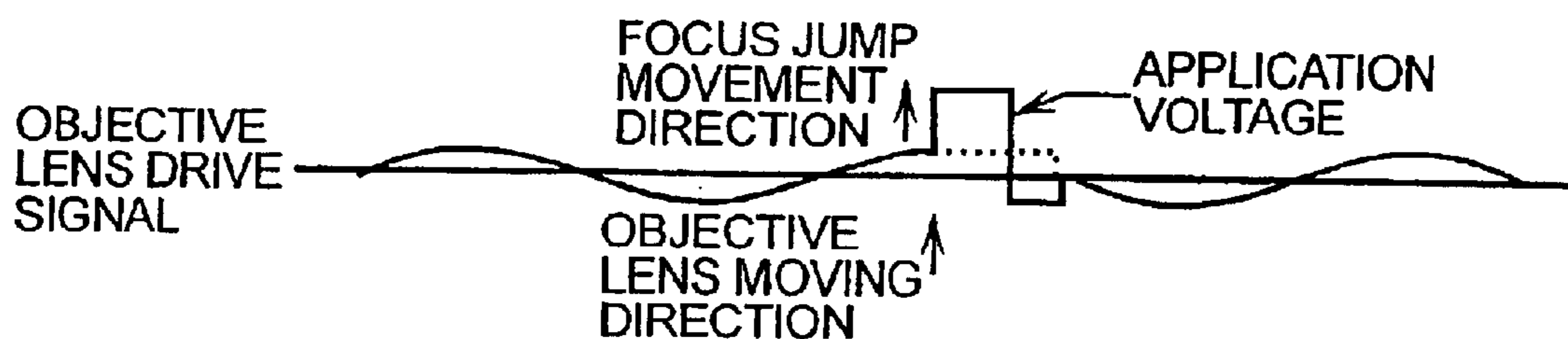
Fig. 4 (b) CASE WHERE A VOLTAGE IS APPLIED TO A PEAK OF A SURFACE VIBRATION COMPONENT (Prior Art)
