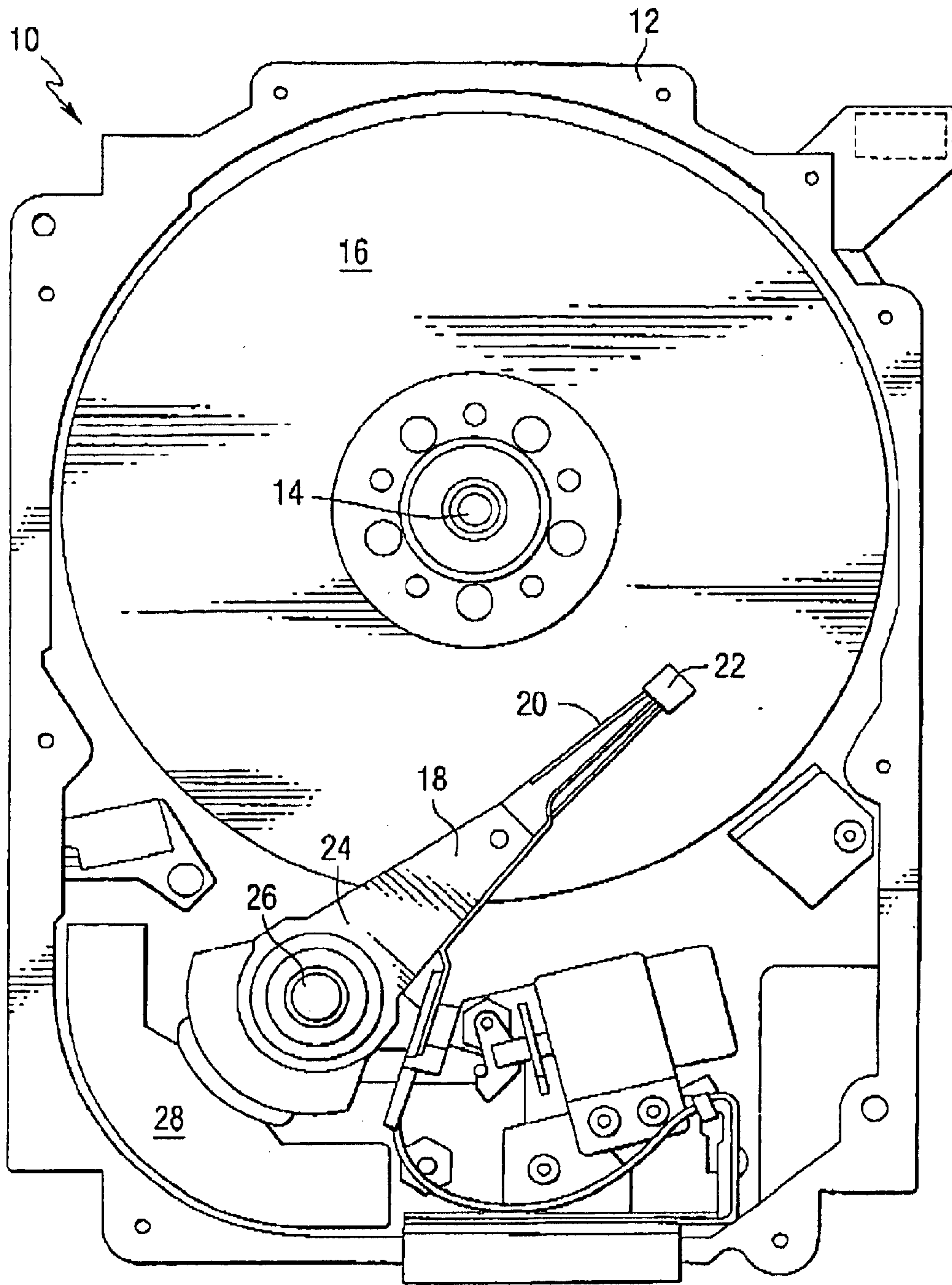
FIG. 1 PRIOR ART
