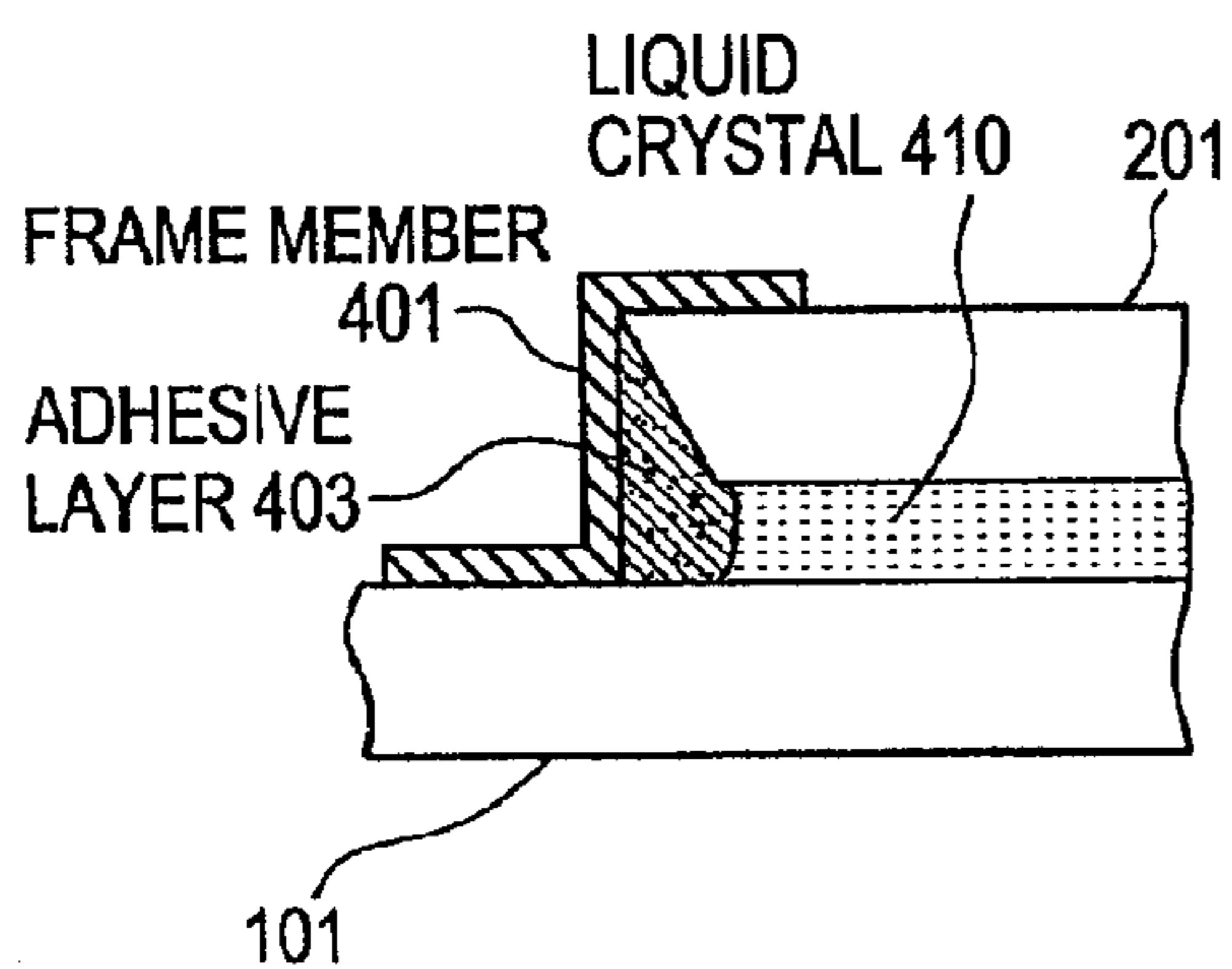
SECTIONAL VIEW OF PORTION a
