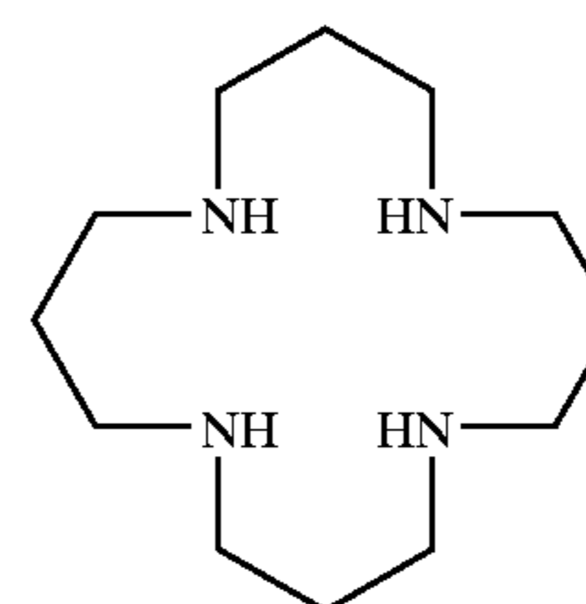
1,5,9,13-tetraazacyclohexadecane
