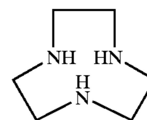
1,4,7,10-triazacyclononane
