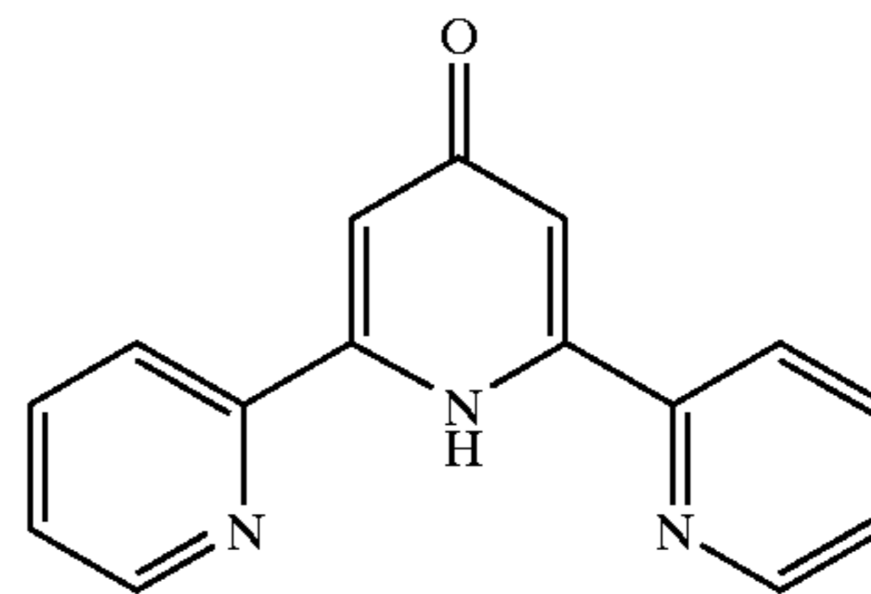
2,6-bis(2-pyridyl)-4(1H)-pyridone
