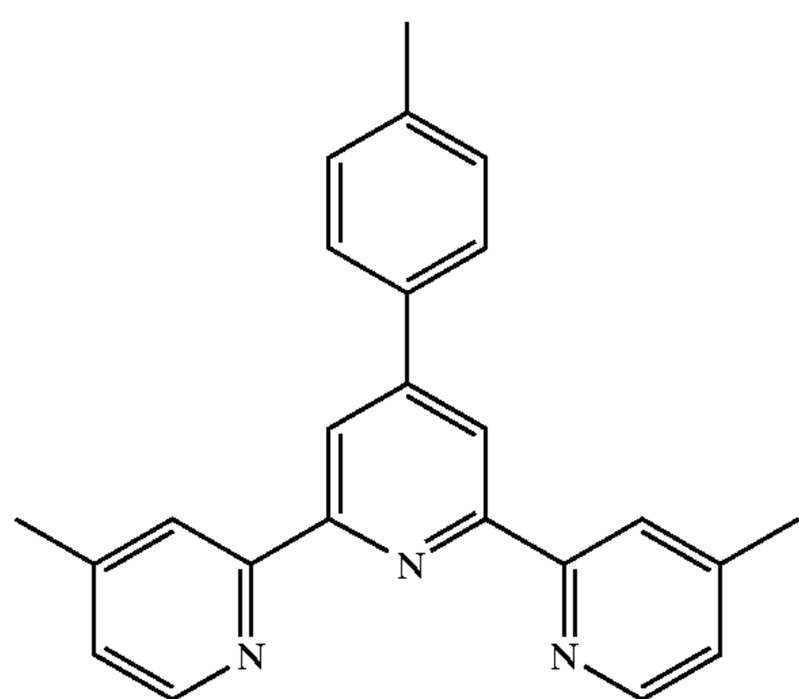
4-4'-dimethyl-4'-(4-methylphenyl)-2,2': 6',2''-terpyridine
