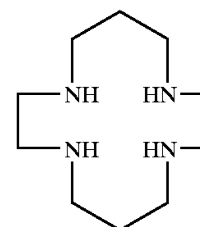
1,4,8,11-tetraazacyclotetradecane
