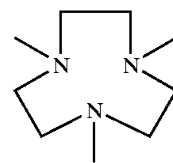
1,4,7,10-trimethyl-1,4,7-triazacyclononane
