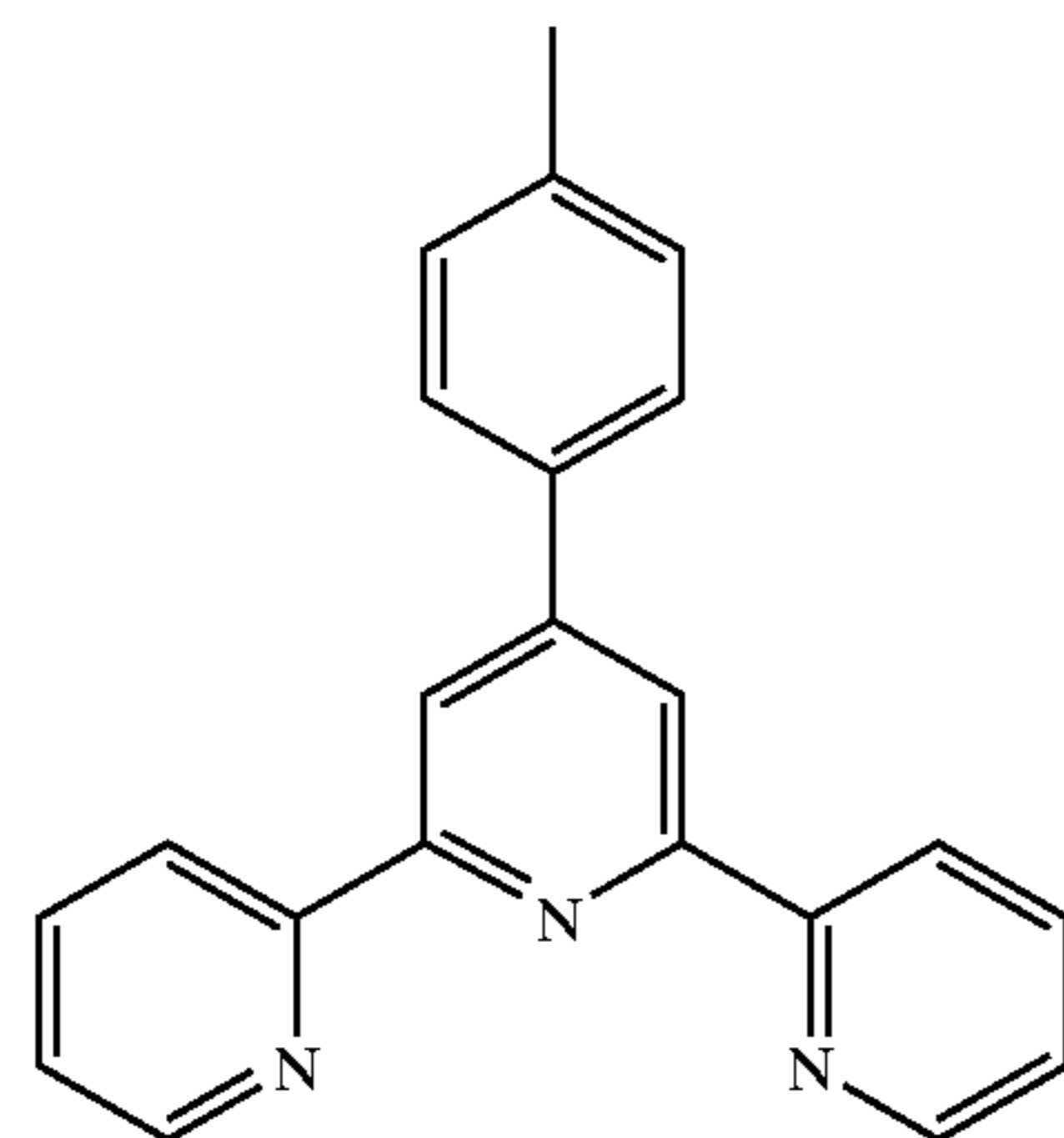
4'-(4-methylphenyl)-2,2': 6',2''-terpyridine
