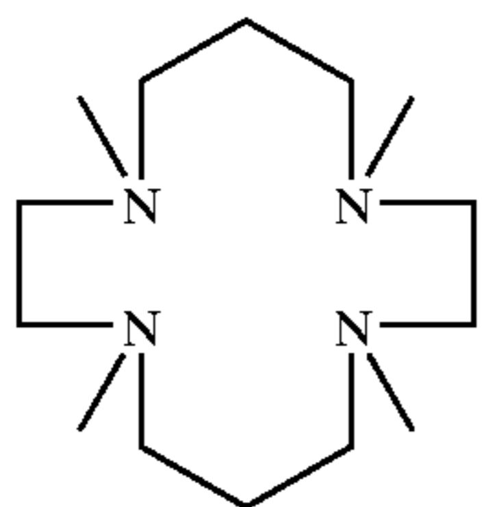
1,4,8,11-Tetramethyl-1,4,8,11-tetraazacyclotetradecane
