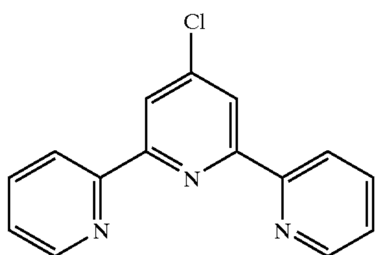
4-chloro-2,2': 6',2''-terpyridine
