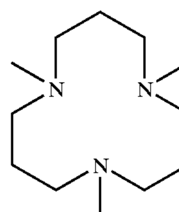
1,5,9-Trimethyl-1,5,9-triazacyclododecane
