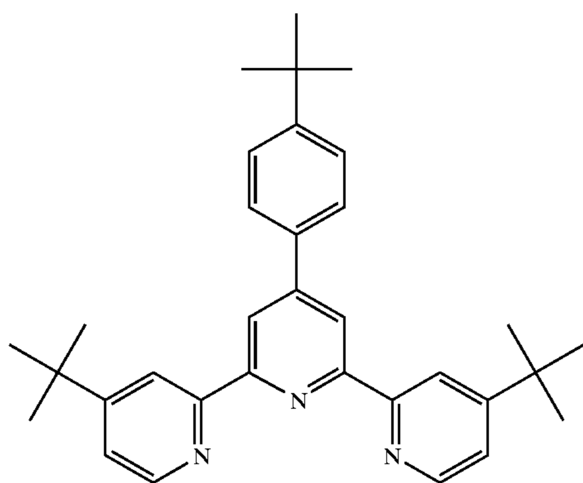
4-4'-4''-tri-tert-butyl-2,2': 6',2''-terpyridine
