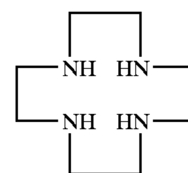
Cyclen(1,4,7,10-tetraazacyclododecane)
