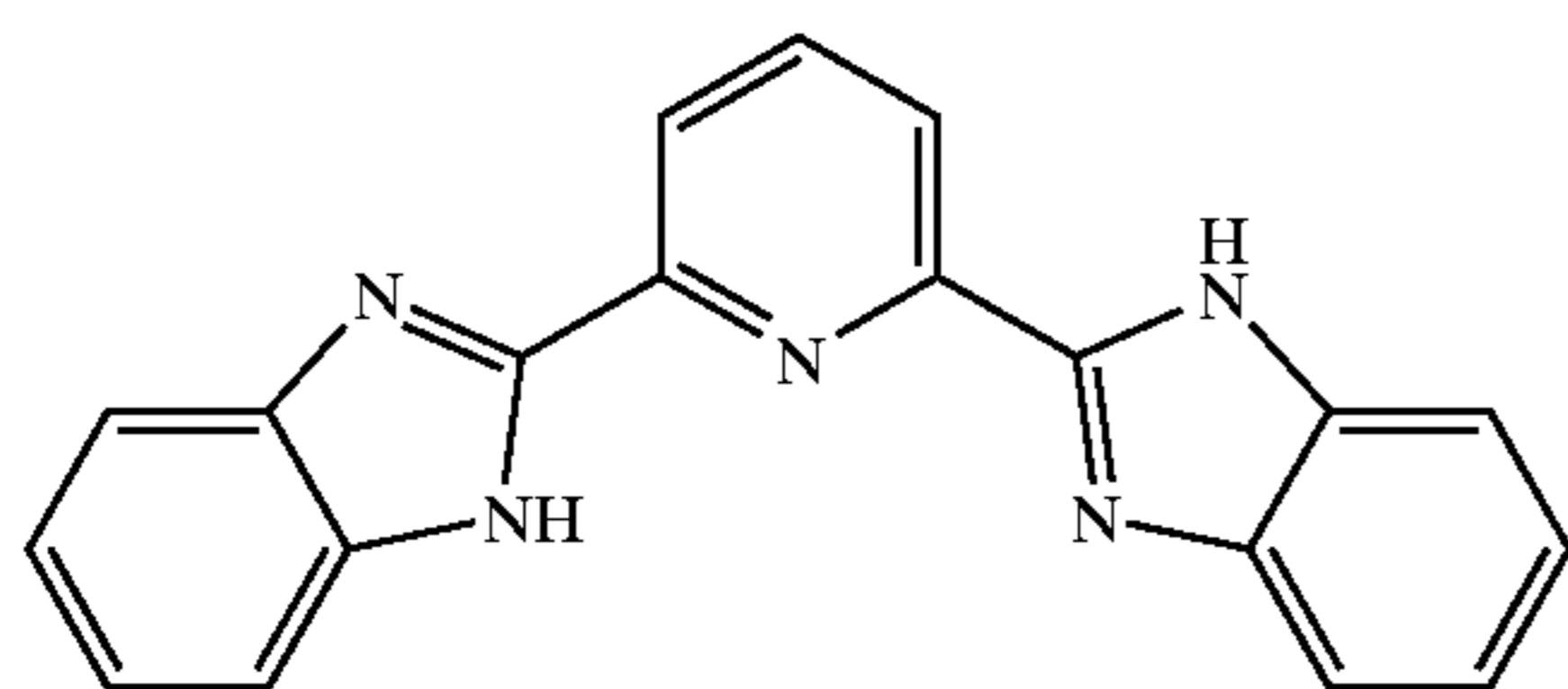
2,6-bis(1-hydrobenzimidazol-2-yl)pyridine
