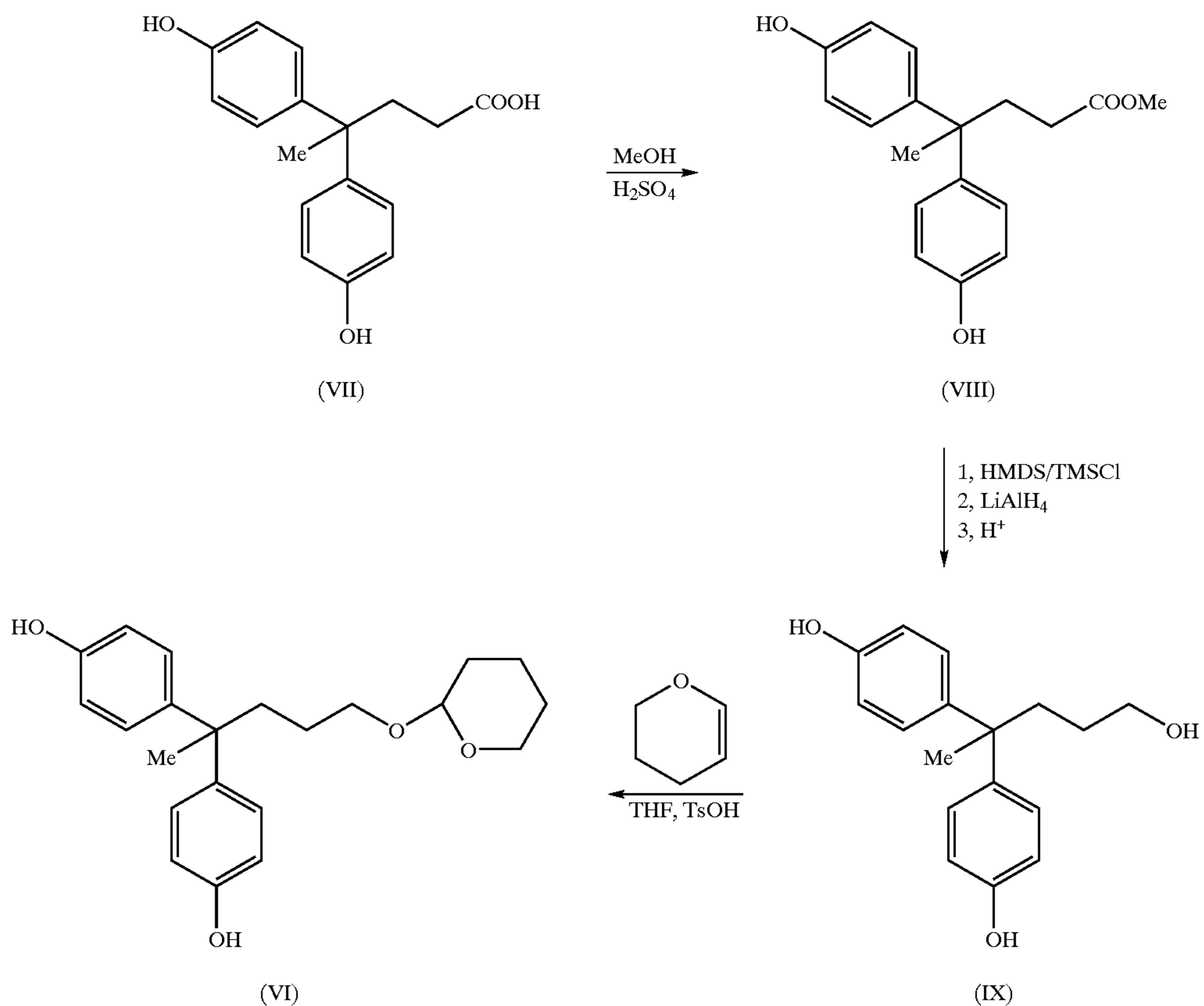
Scheme (III)
