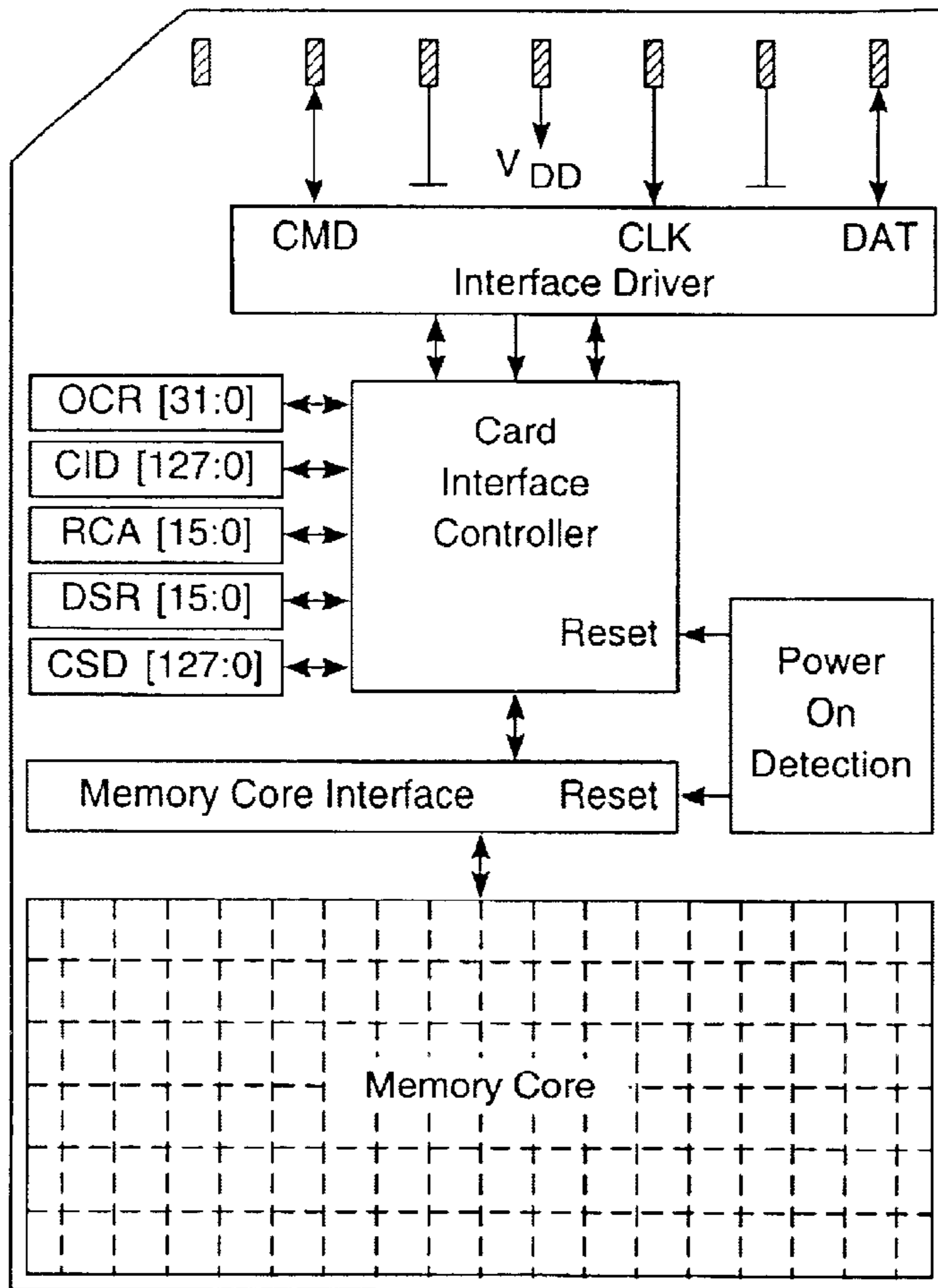
FIG. 6 (PRIOR ART)
