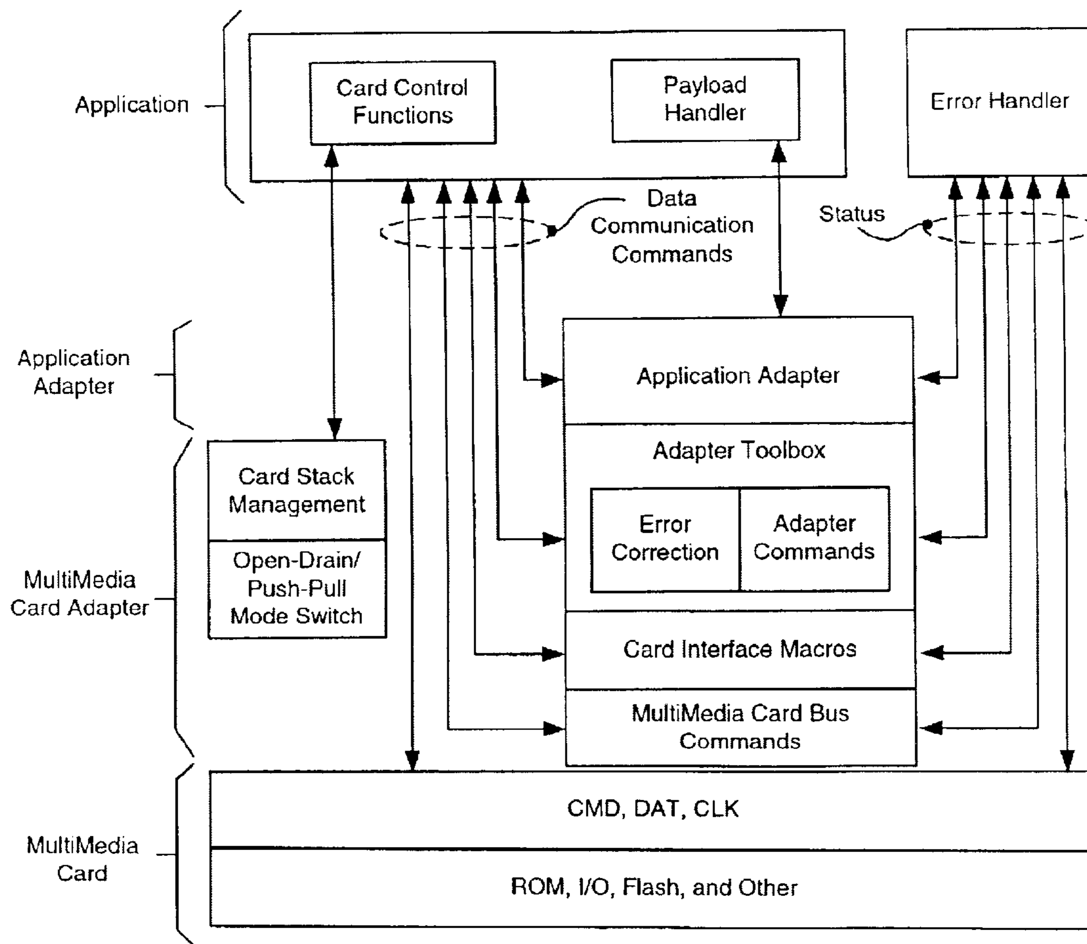
FIG. 8 (PRIOR ART)
