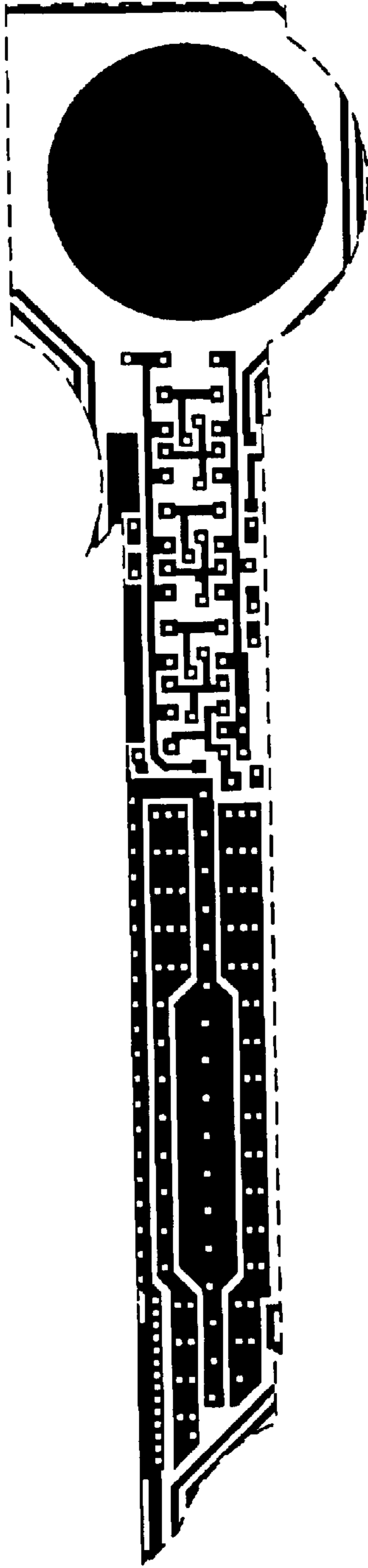
Metal 1 mask
