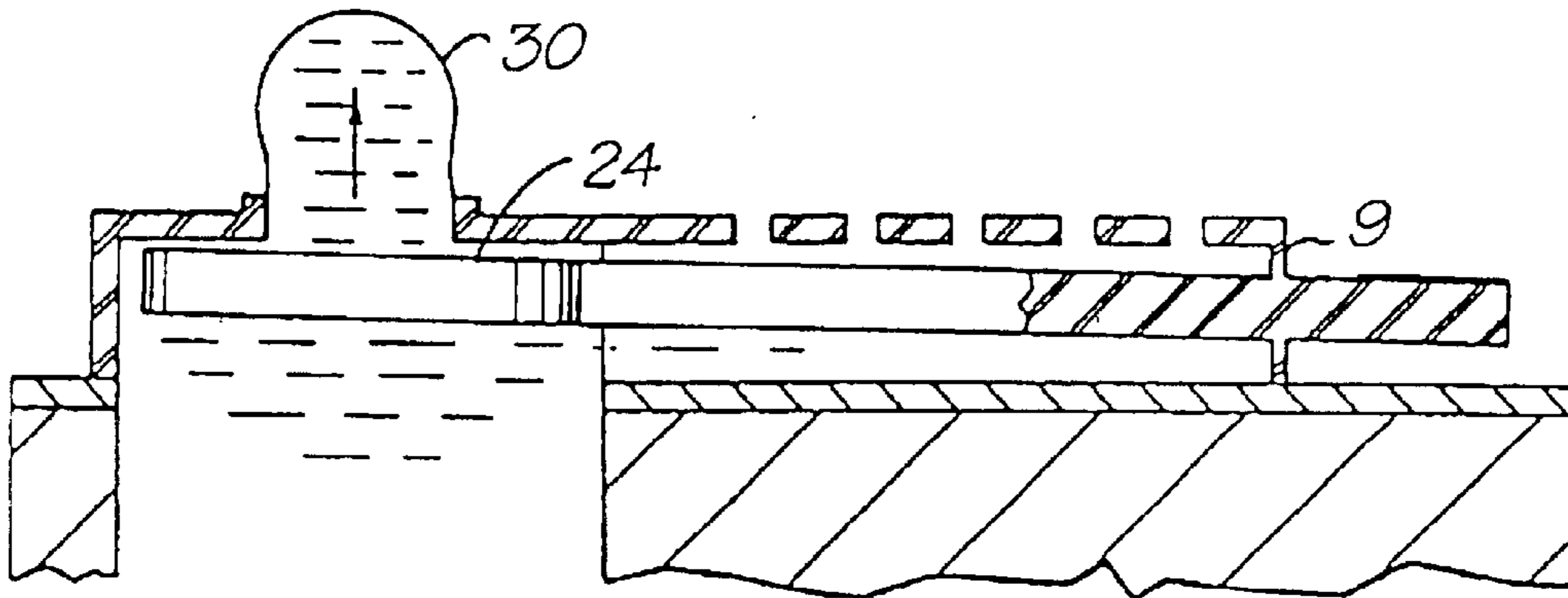
FIG. 4 (PRIOR ART)
