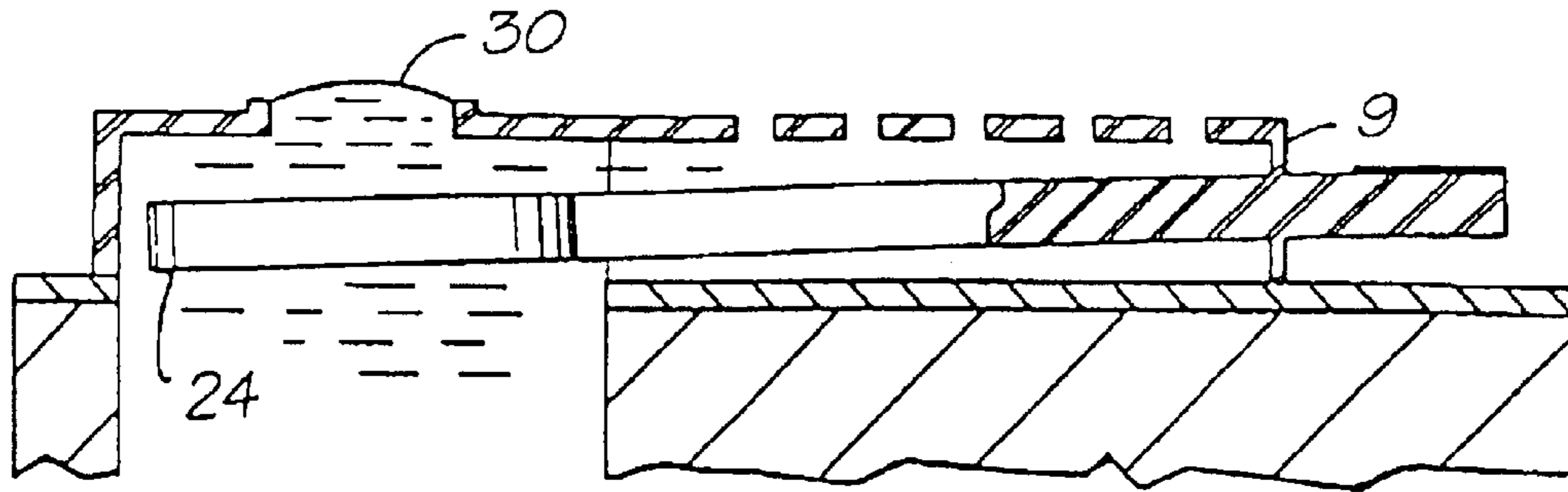
FIG. 3 (PRIOR ART)
