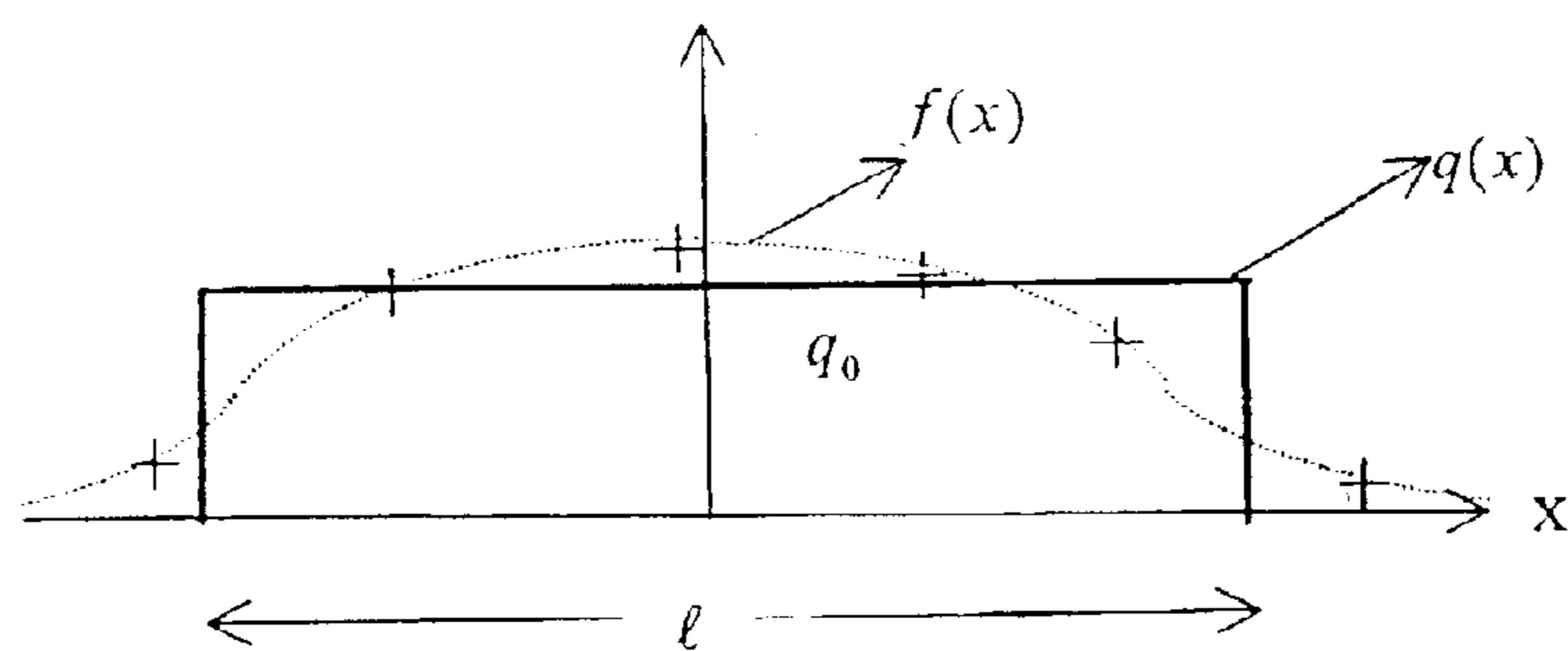
Fig. 6 Determination of Effective Heat flux, q_0 , and length, l , of a Measured Heat Flux Distribution, f(x) .
