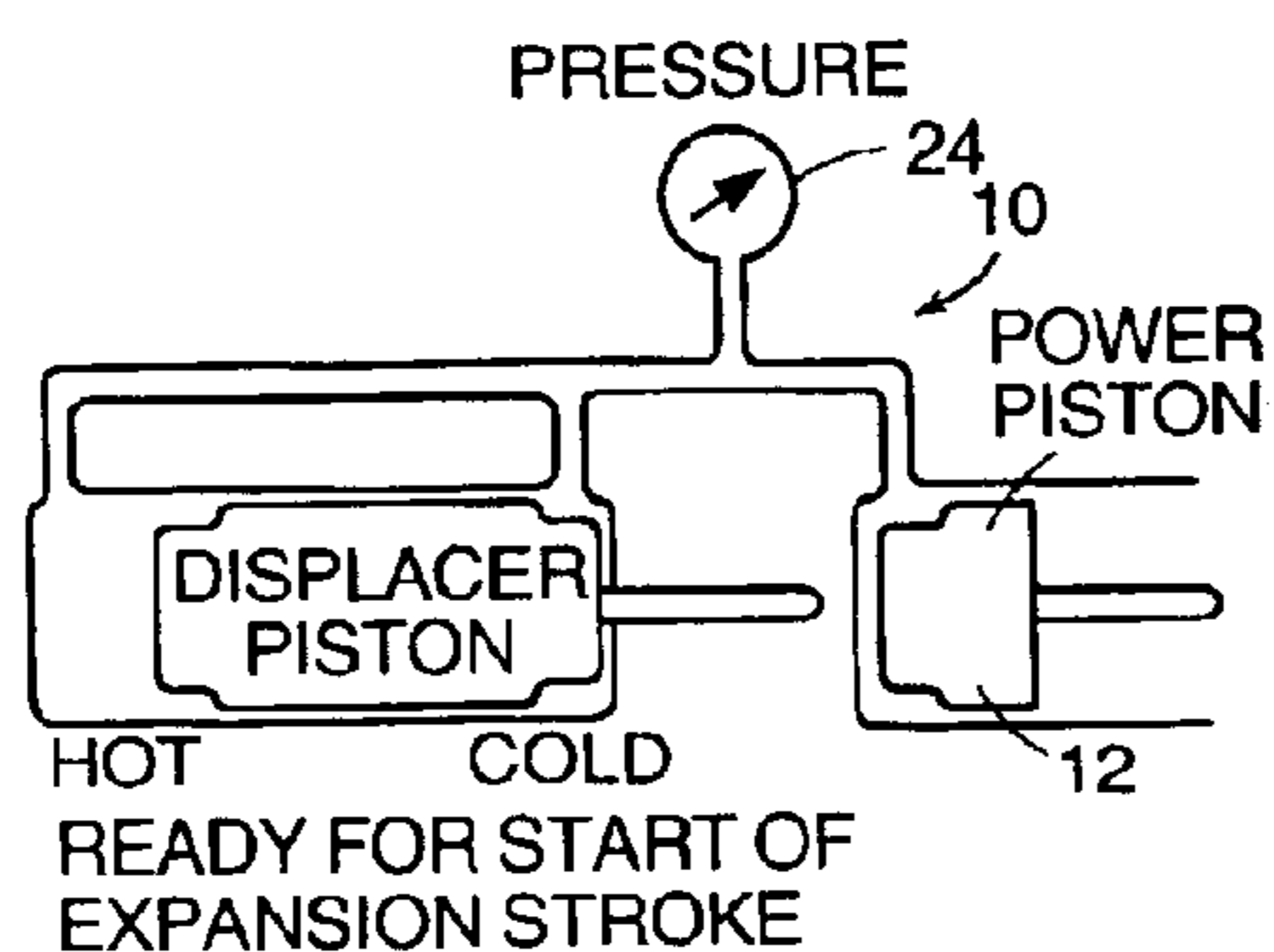
FIG. 1c PRIOR ART
