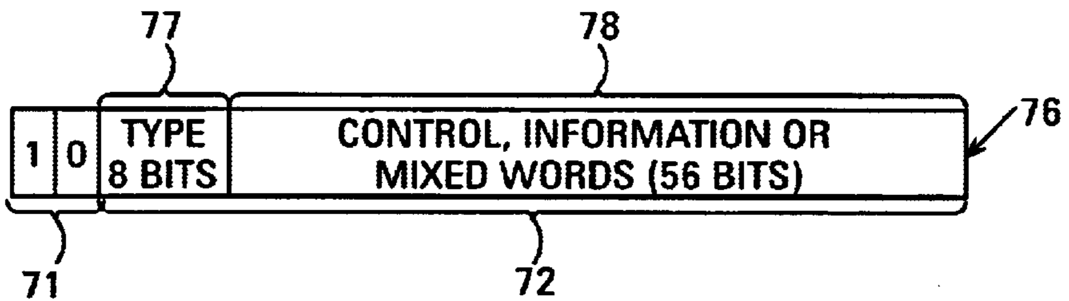
FIG. 2C (PRIOR ART)
