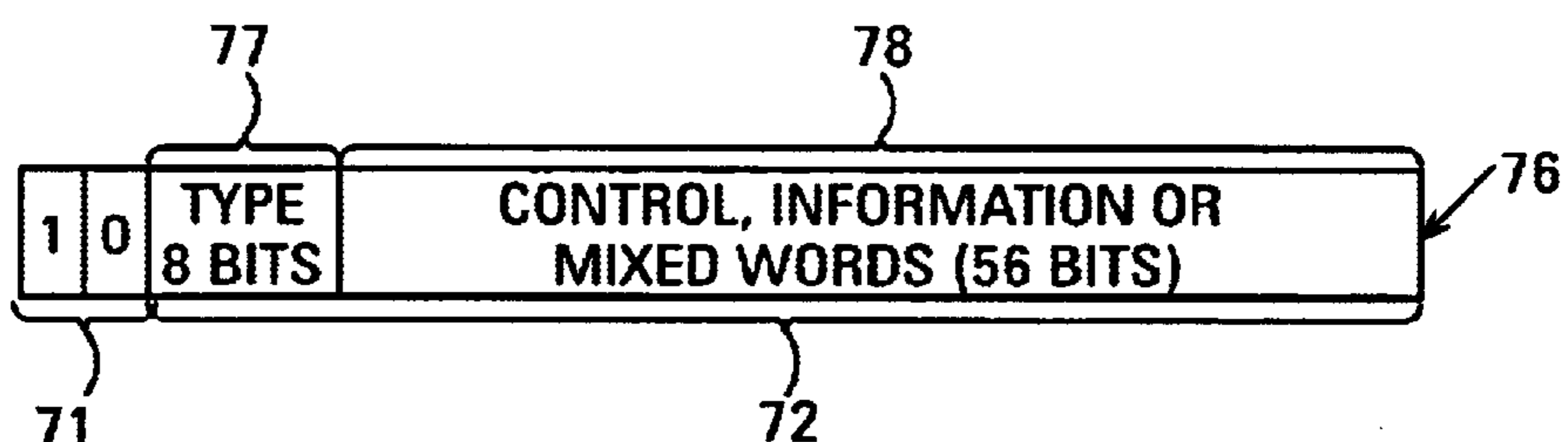
FIG. 2C (PRIOR ART)
