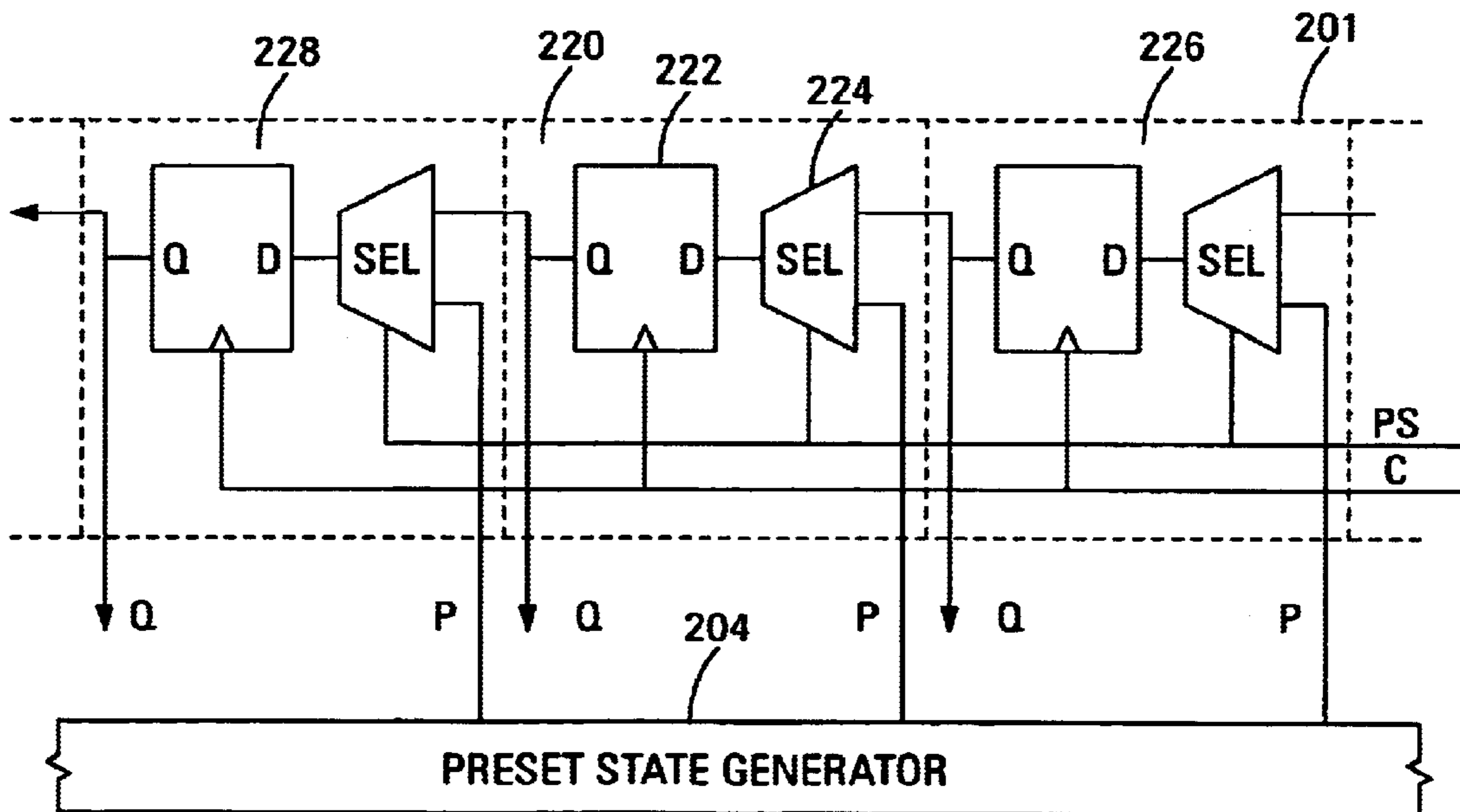
FIG. 2C (PRIOR ART)
