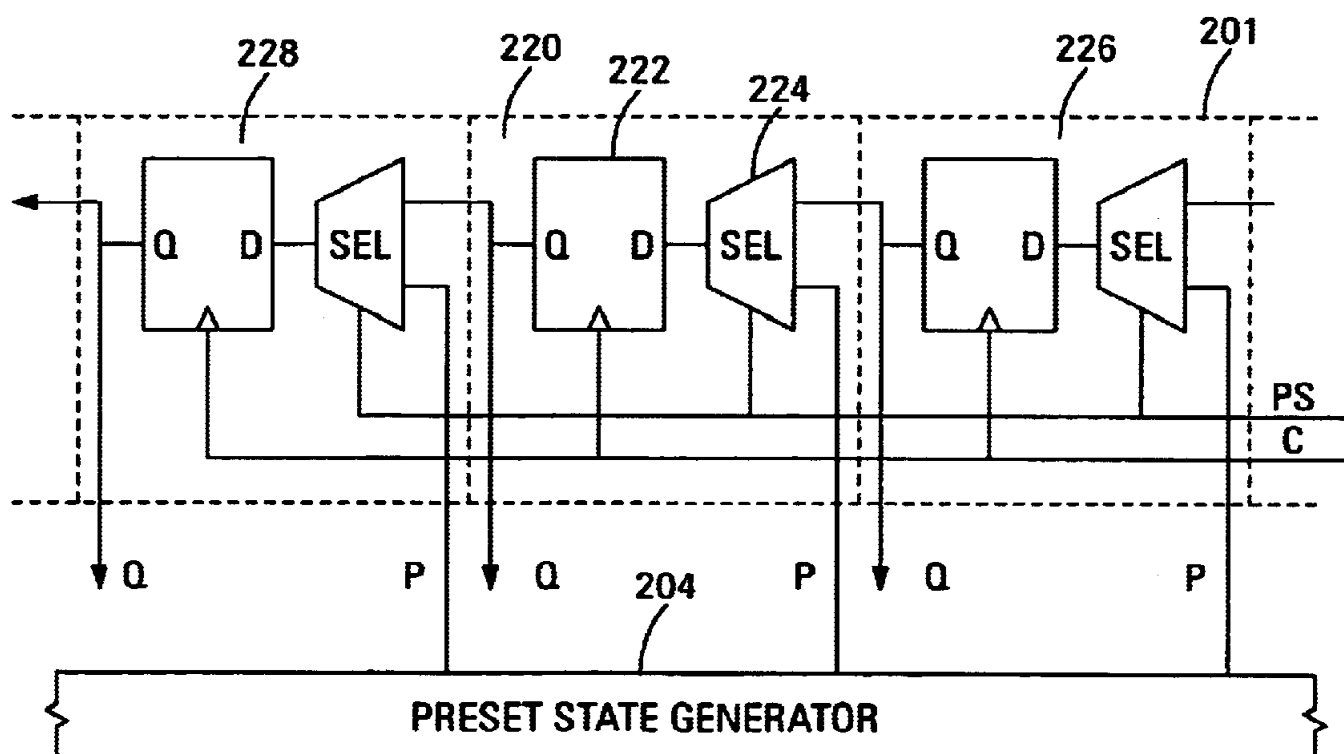
FIG. 2C (PRIOR ART)
