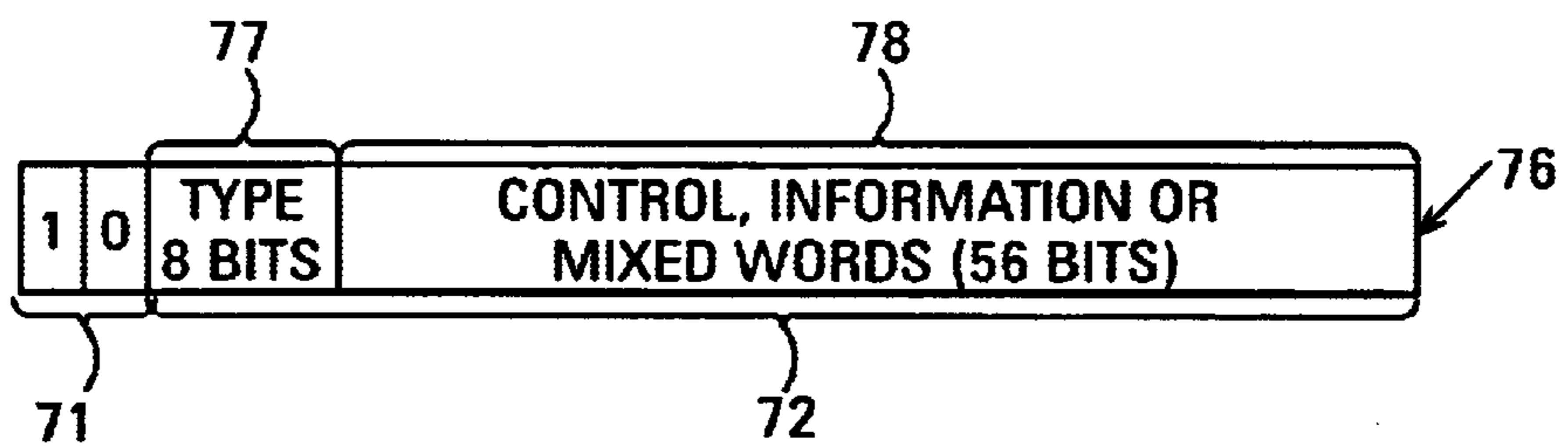
FIG. 2C (PRIOR ART)
