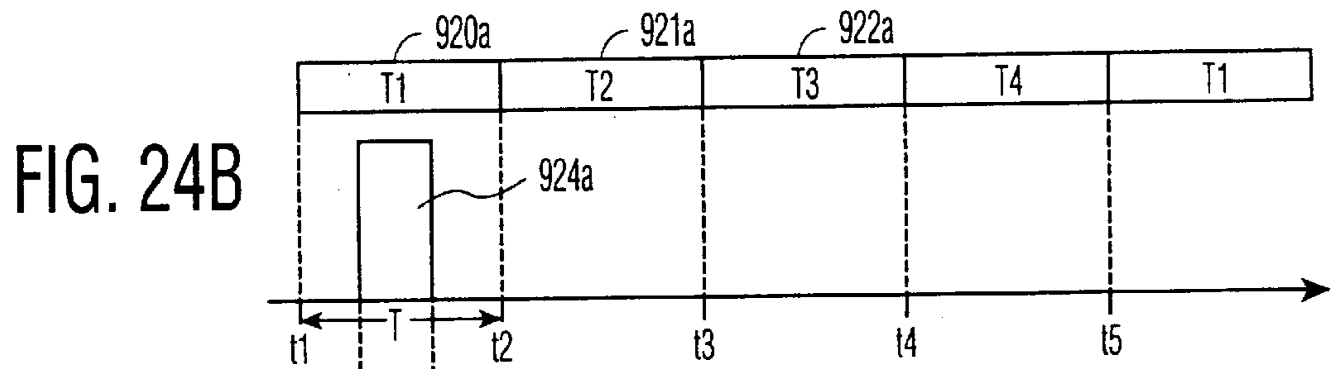
FIG. 24B (2) TRIMMING PATTERN OF "00"
