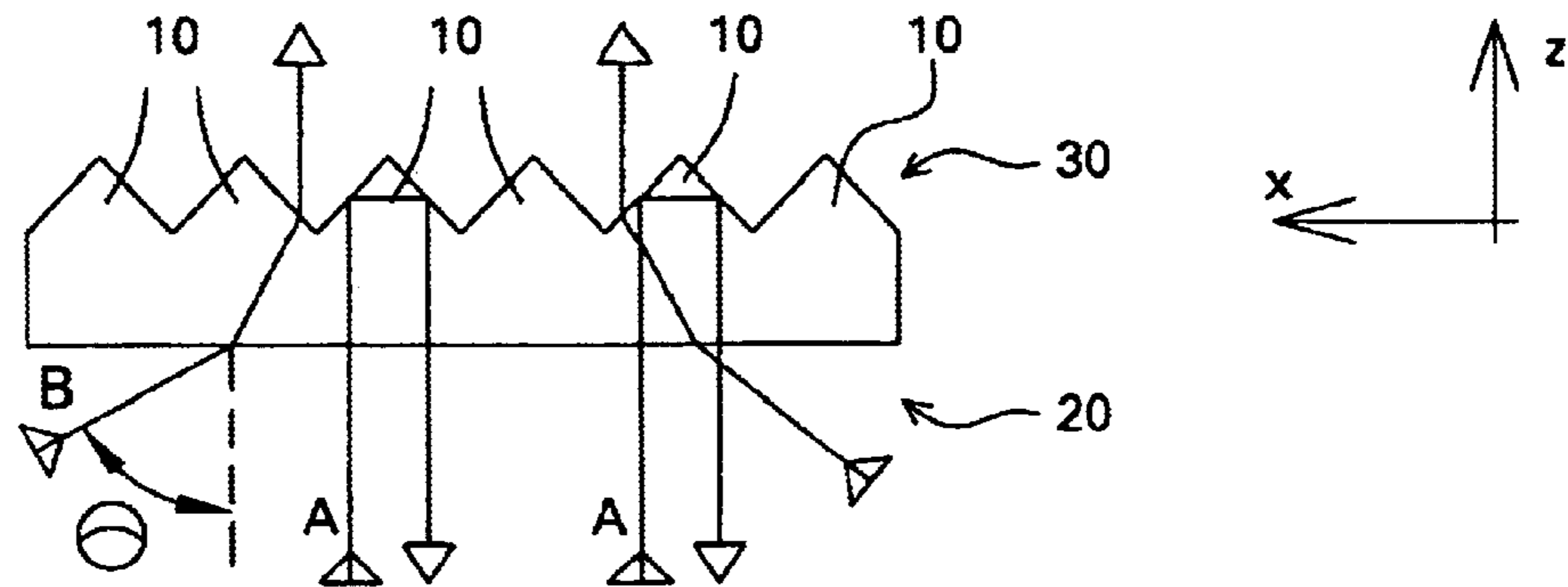
FIG.1 (PRIOR ART)
