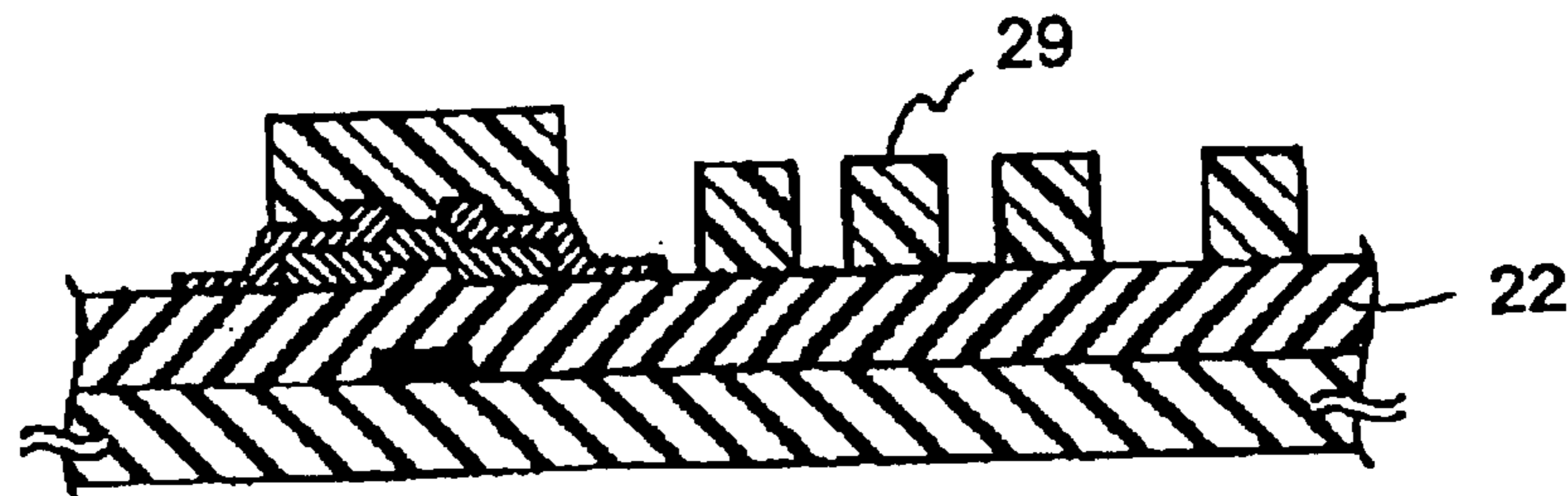
FIG. 2F (PRIOR ART)
