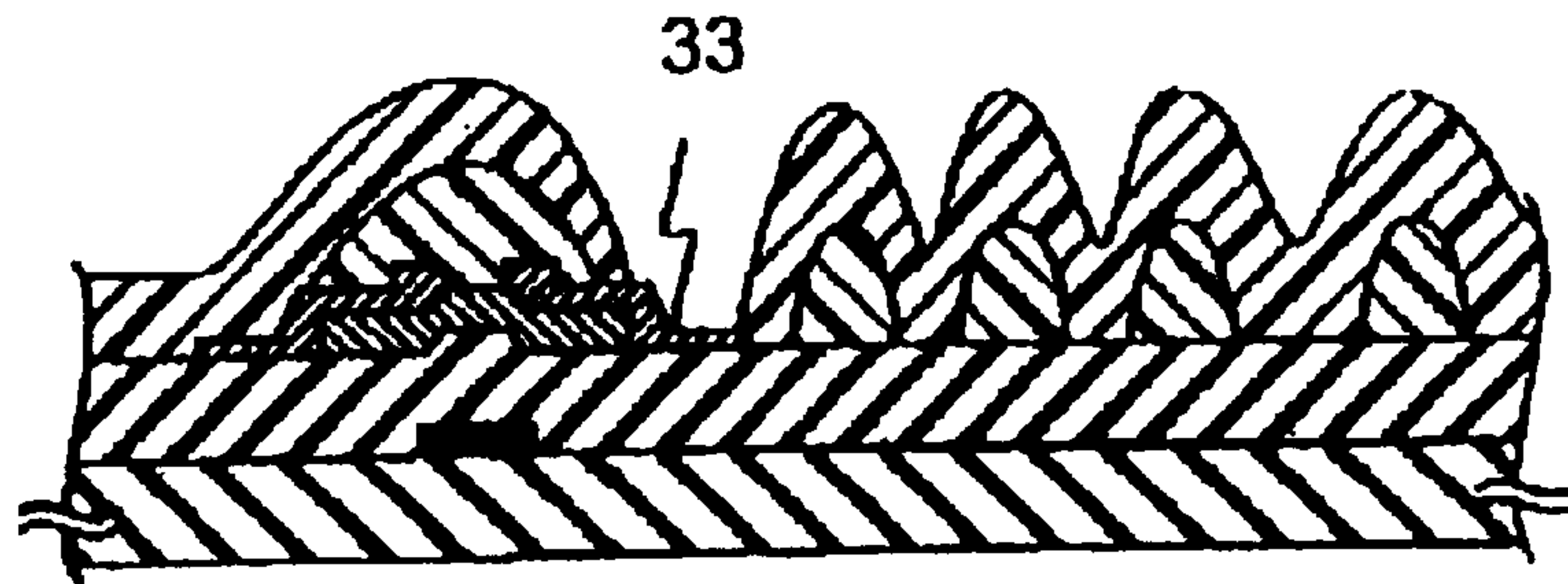
FIG. 2I (PRIOR ART)
