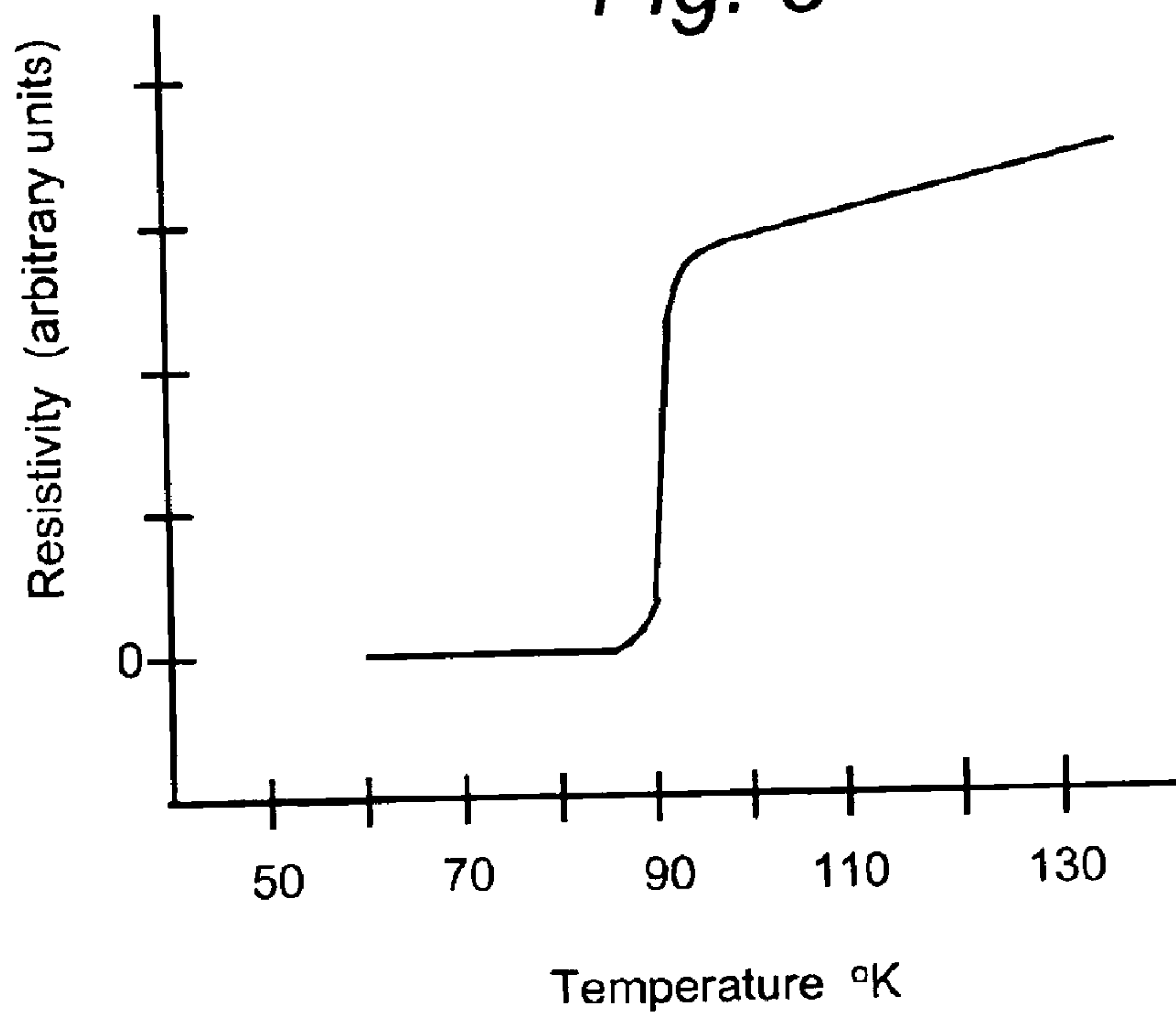
Resistivity vs. temperature of YBa 2 Cu 3 O 7
