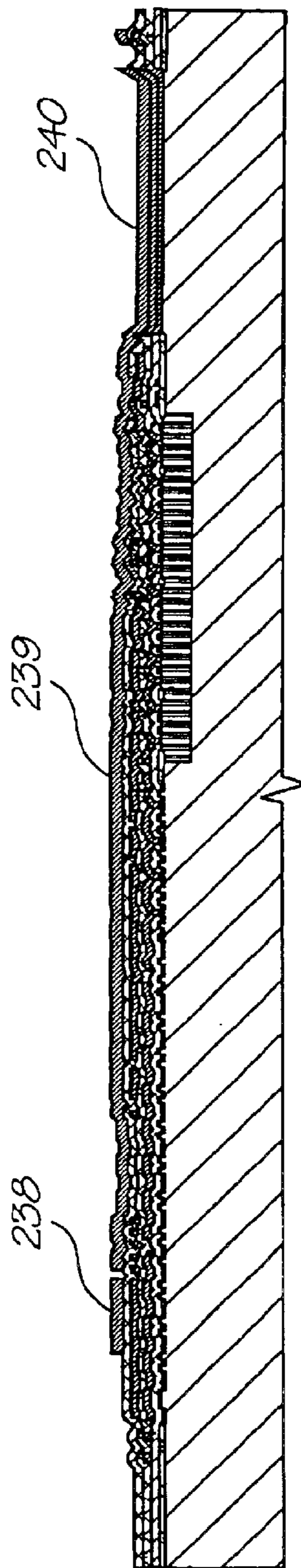
Deposit metal 3
