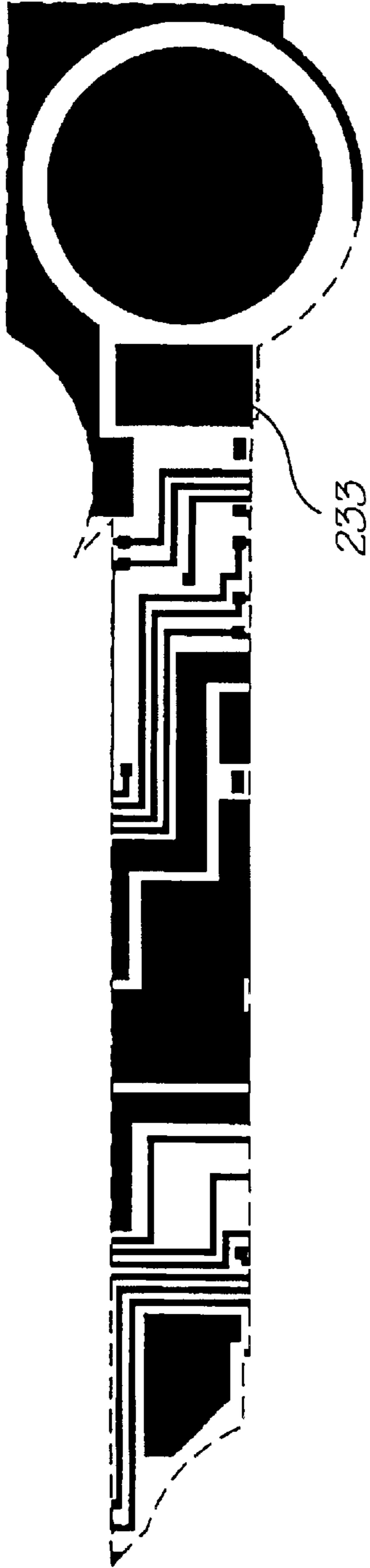
Metal 2 mask
