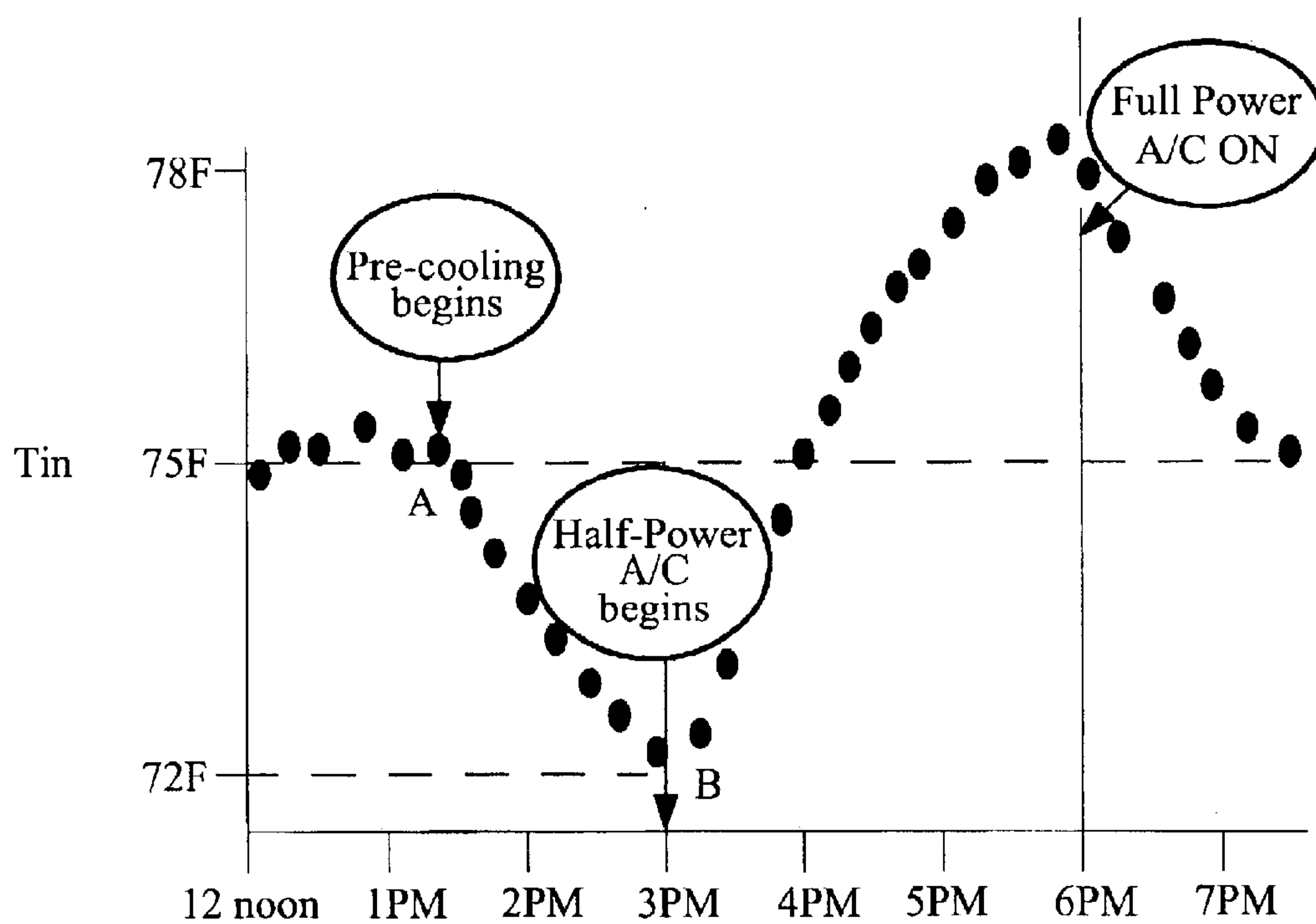
Energy Saver in Peak Demand Reduction Mode
