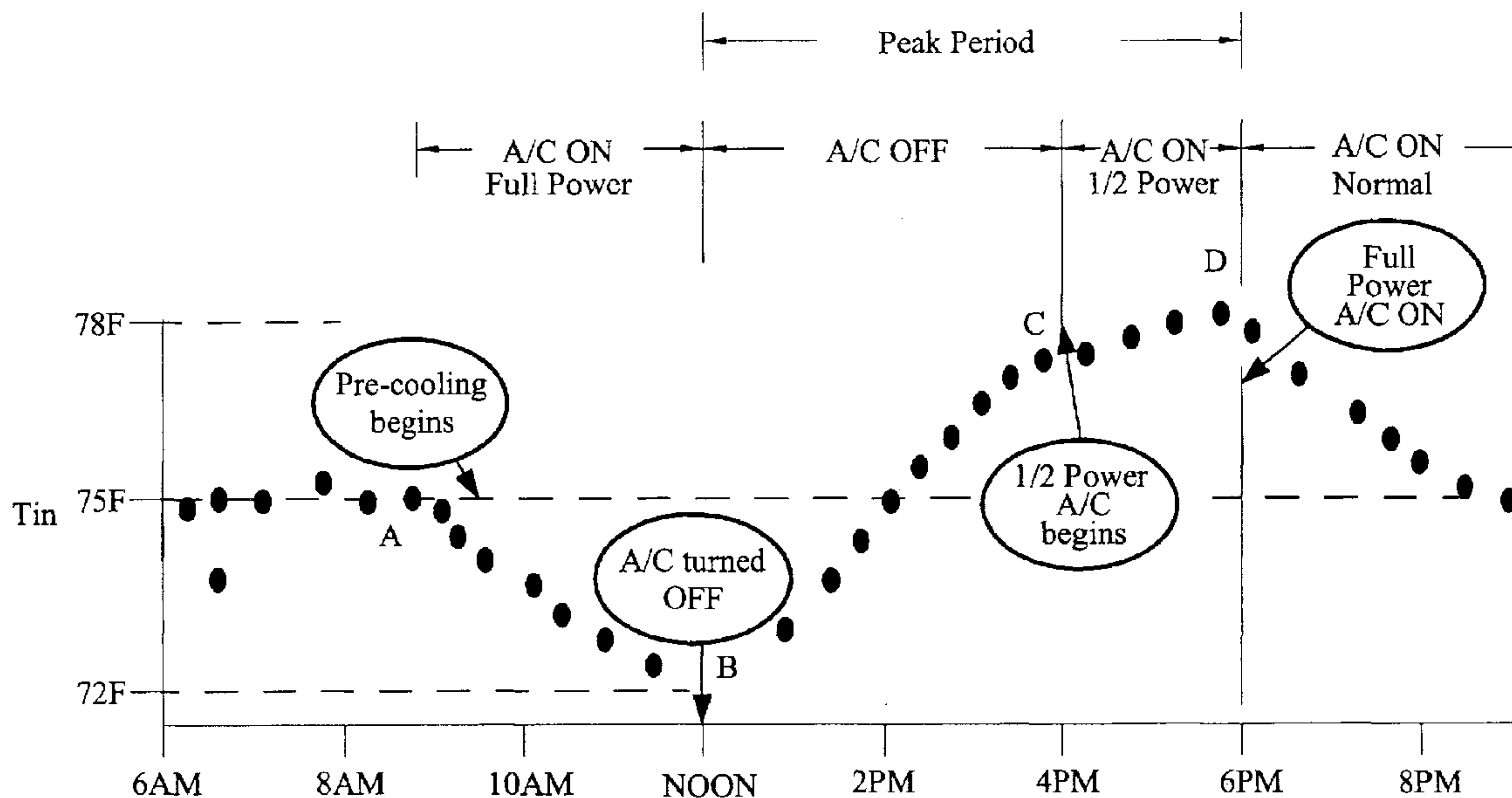
Energy Saver in Peak Reduction Mode for 3-Level System
