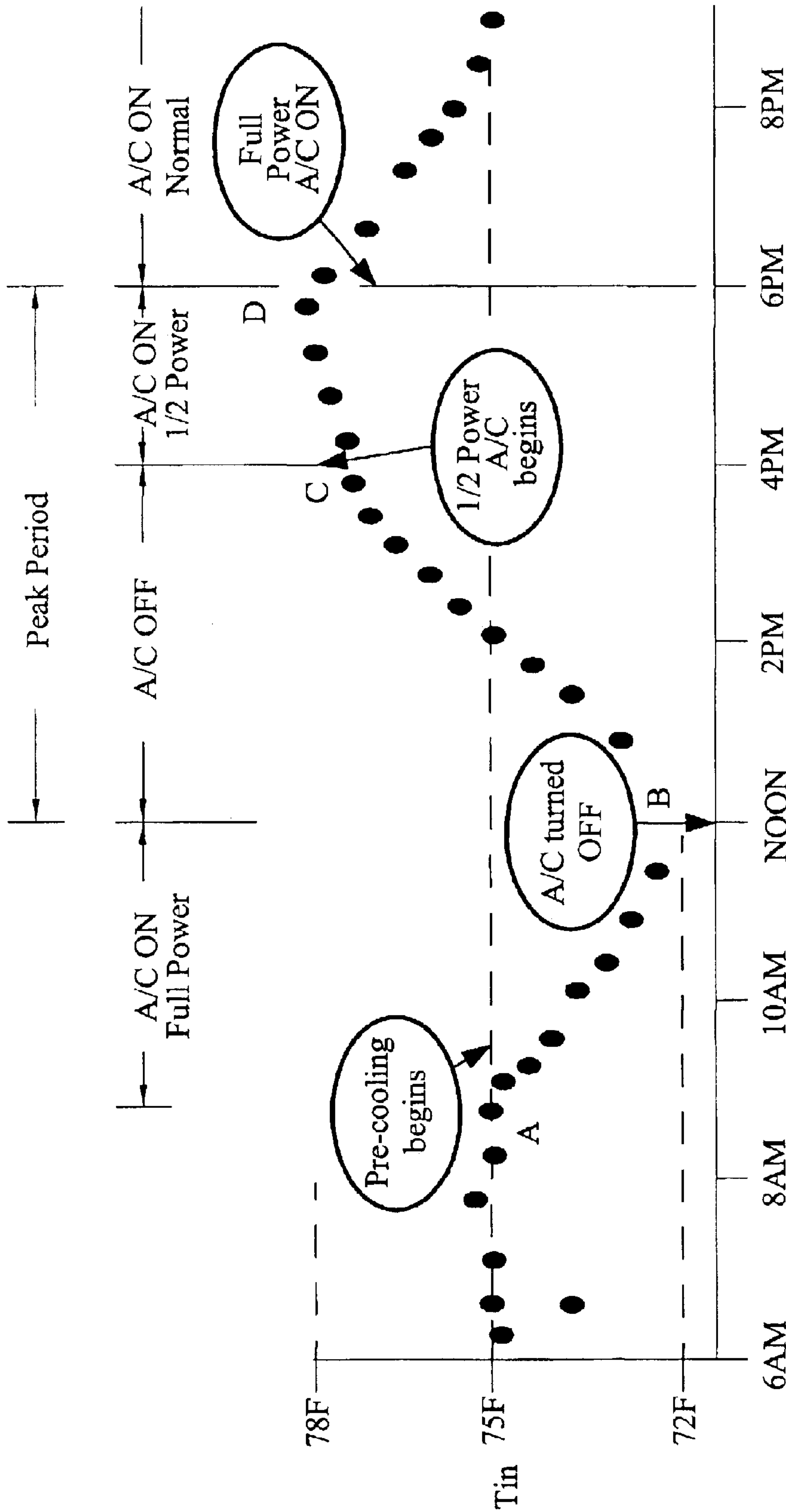
Energy Saver in Peak Reduction Mode for 3-Level System
