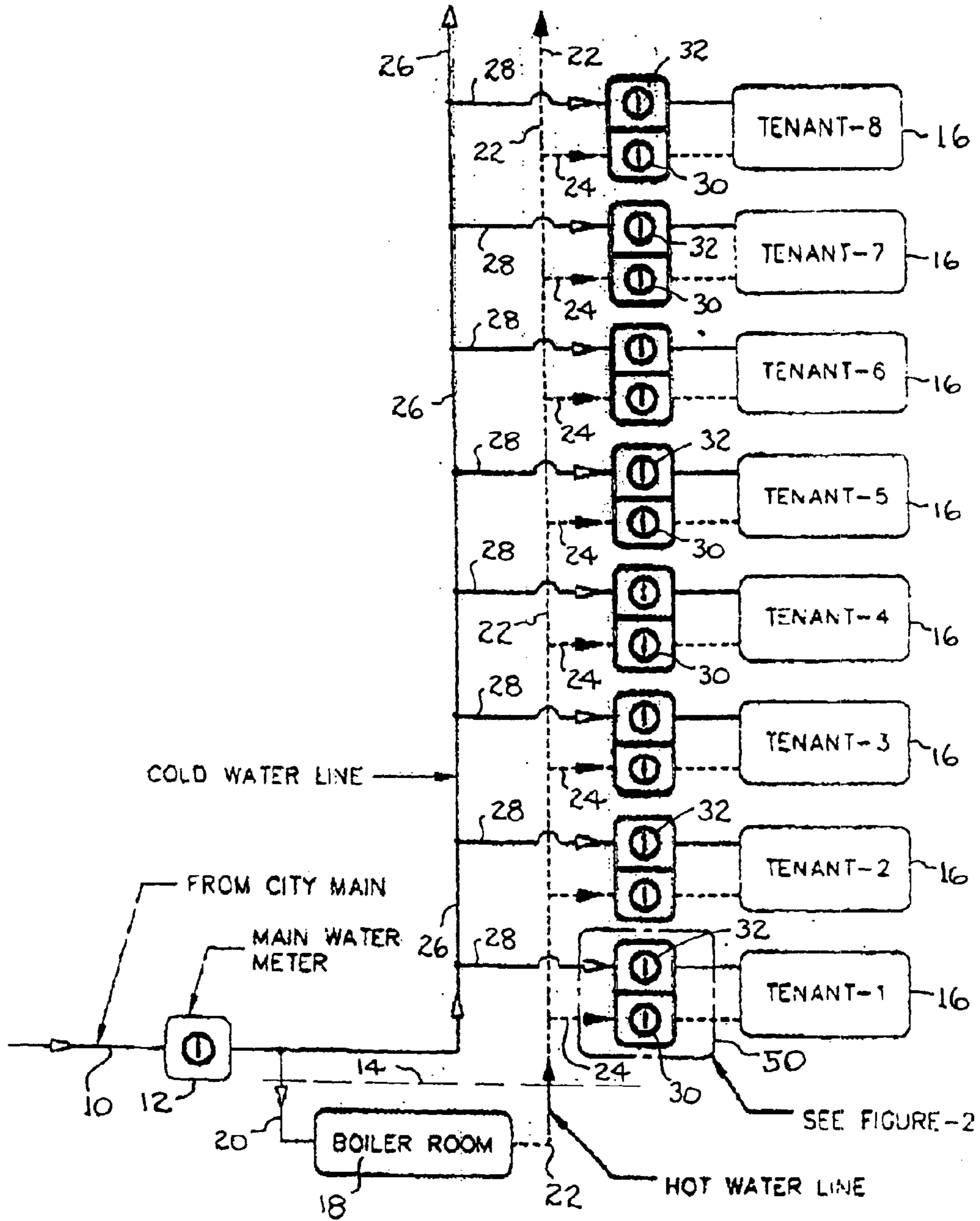
FIGURE-1 WATER LINE DIAGRAM
