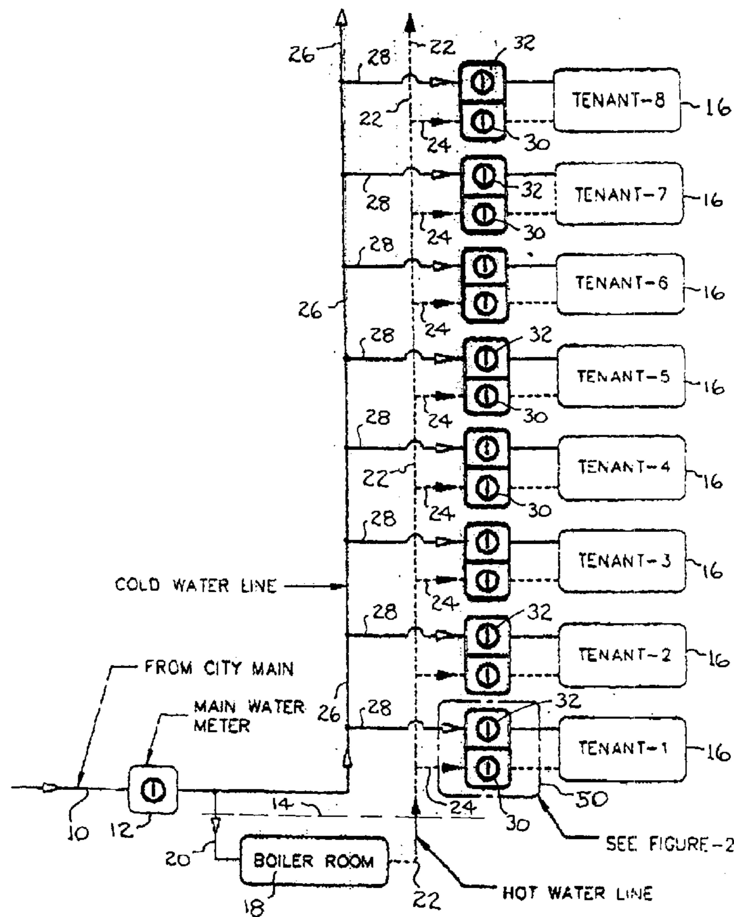
WATER LINE DIAGRAM
