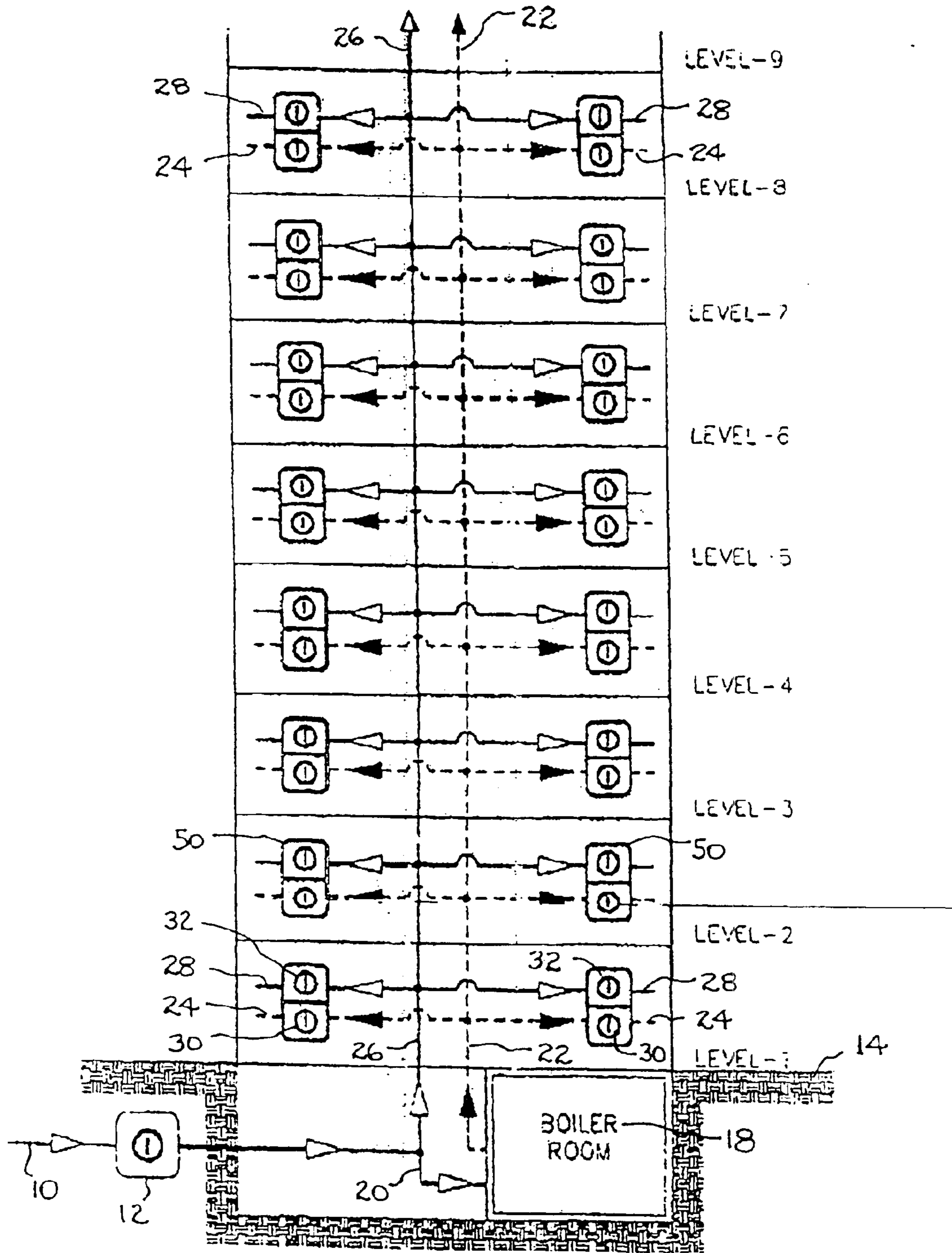
FIGURE-3 HIGH-RISE BUILDING APPLICATION
