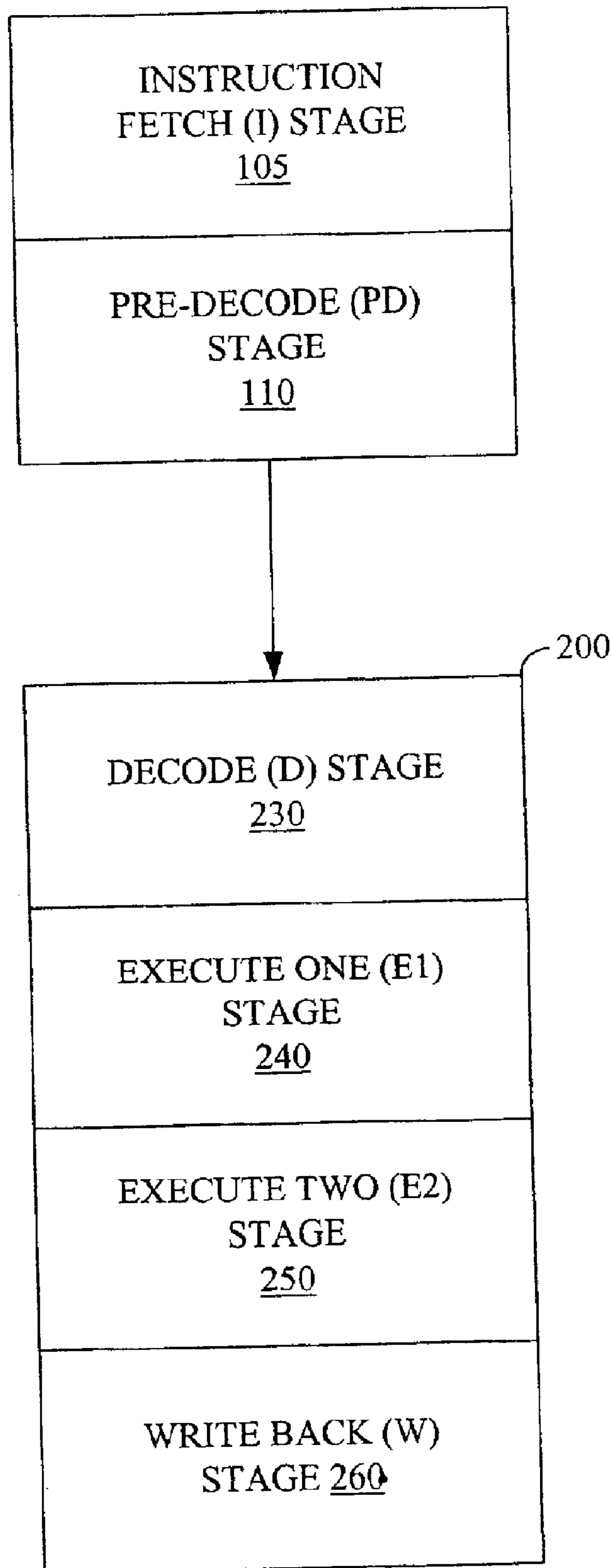
FIGURE 2 (Prior Art)
