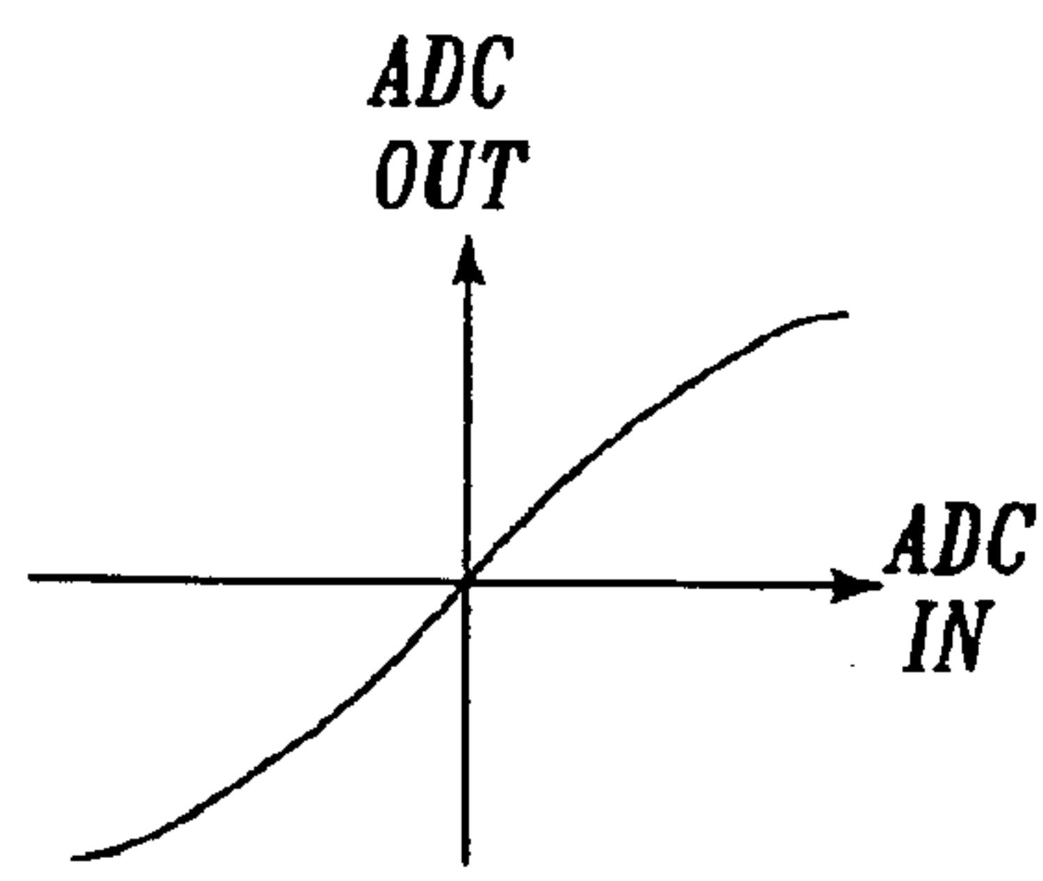
SYMMETRICAL (3RD HARMONIC) DISTORTION IN ADC
