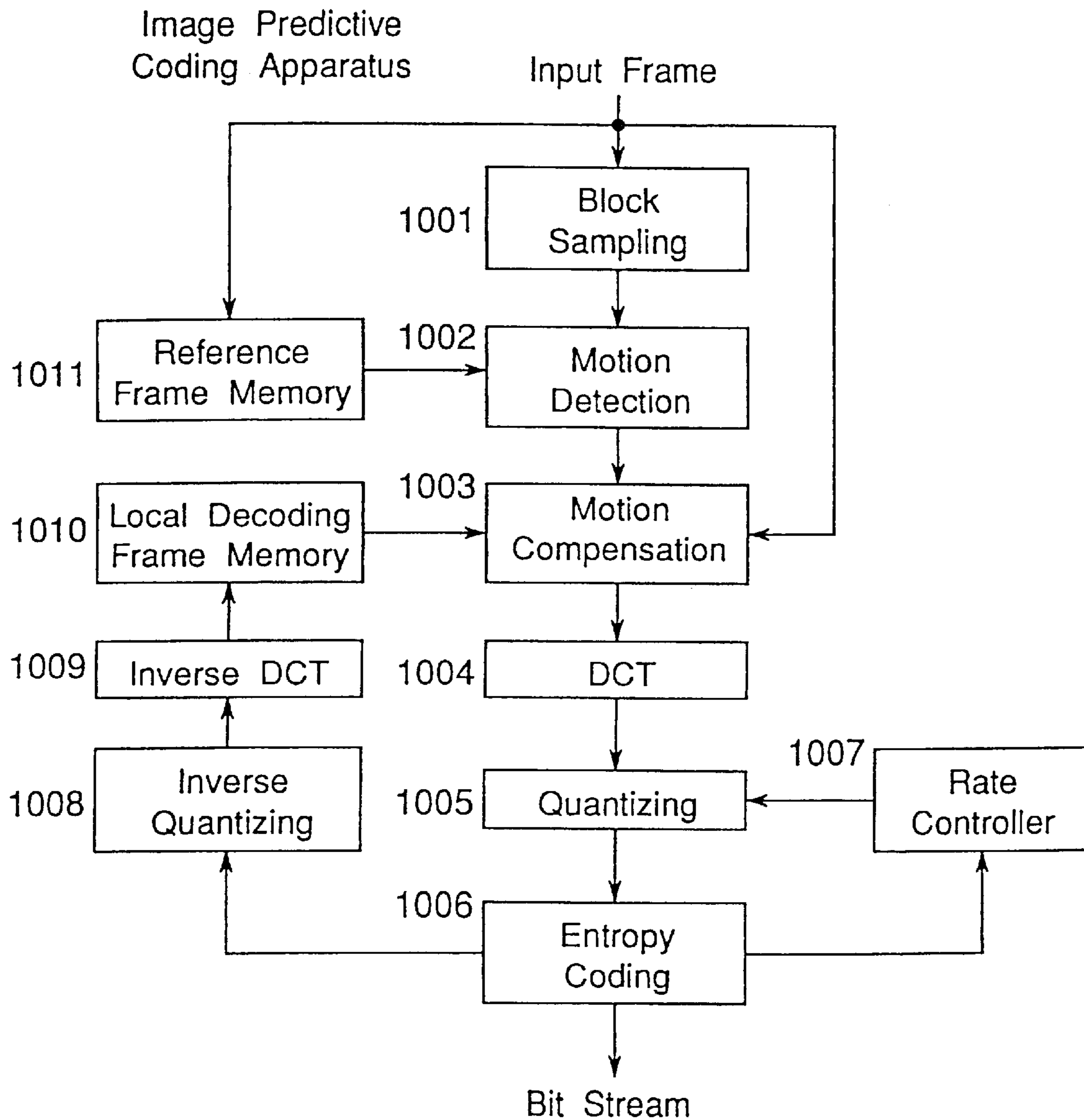
Fig.14 PRIOR ART
