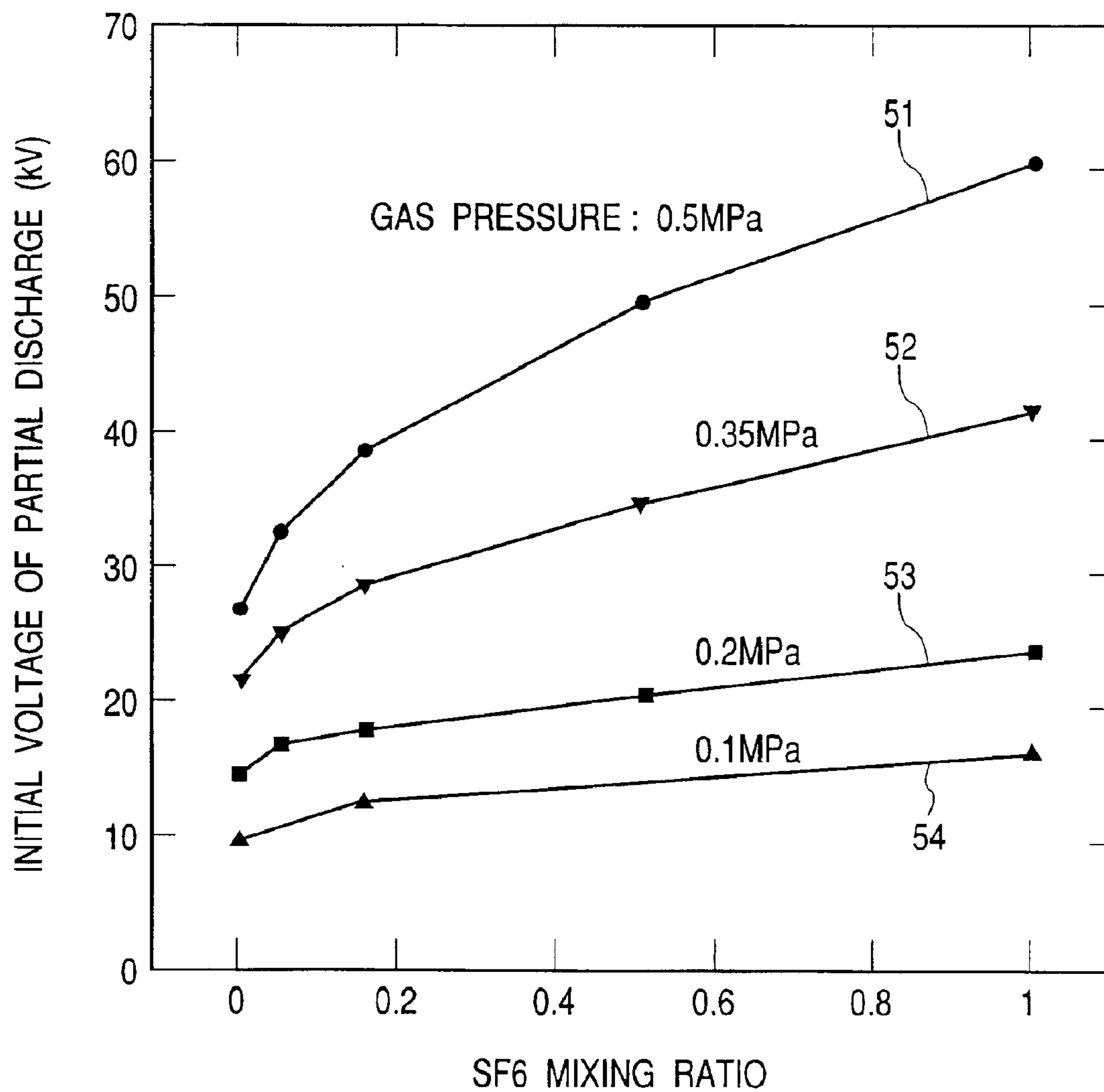
MIXING RATIO PARTIAL DISCHARGE CHARACTERISTICS (KRAFT PAPER)
