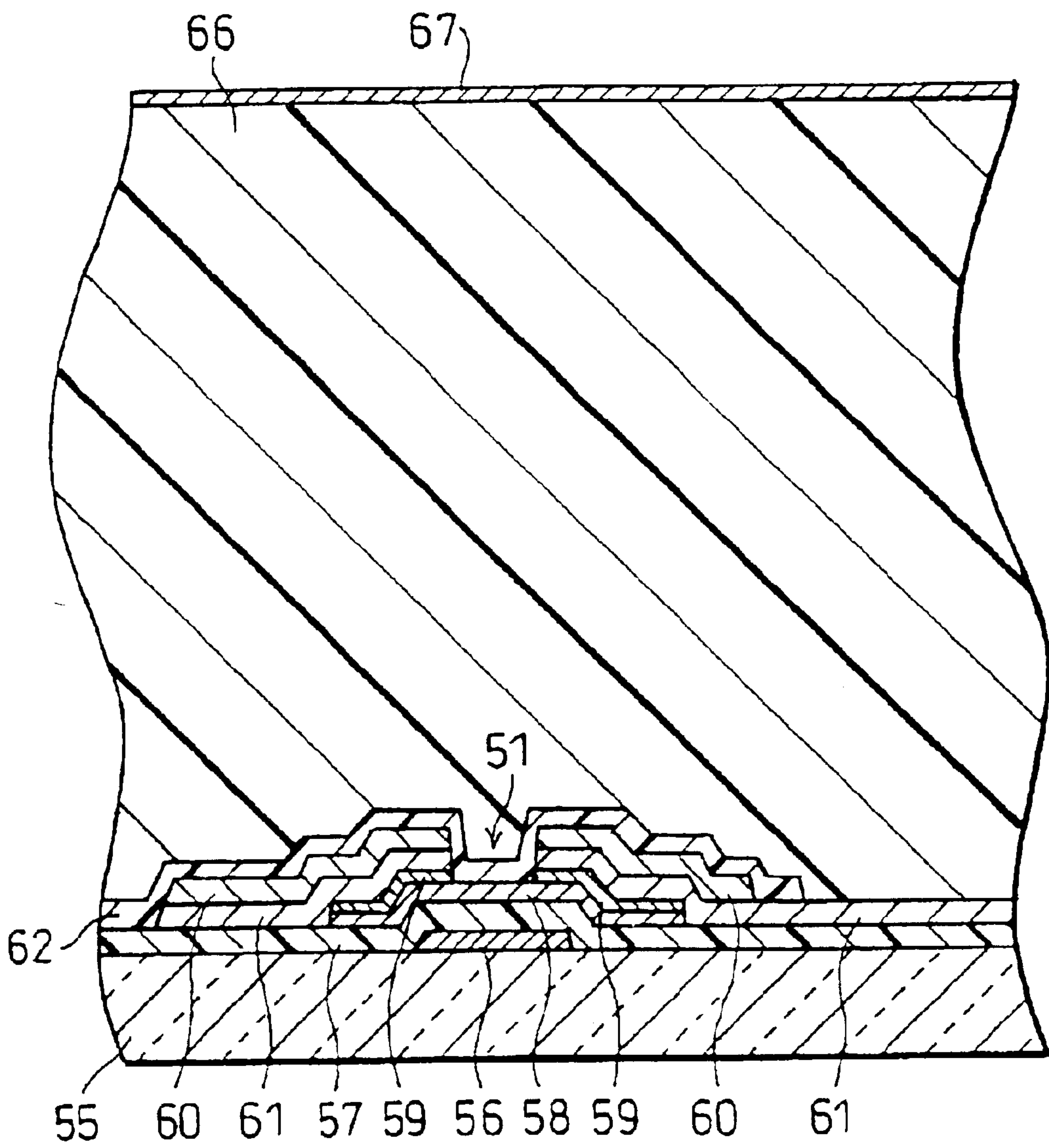
FIG. 6 (PRIOR ART)
