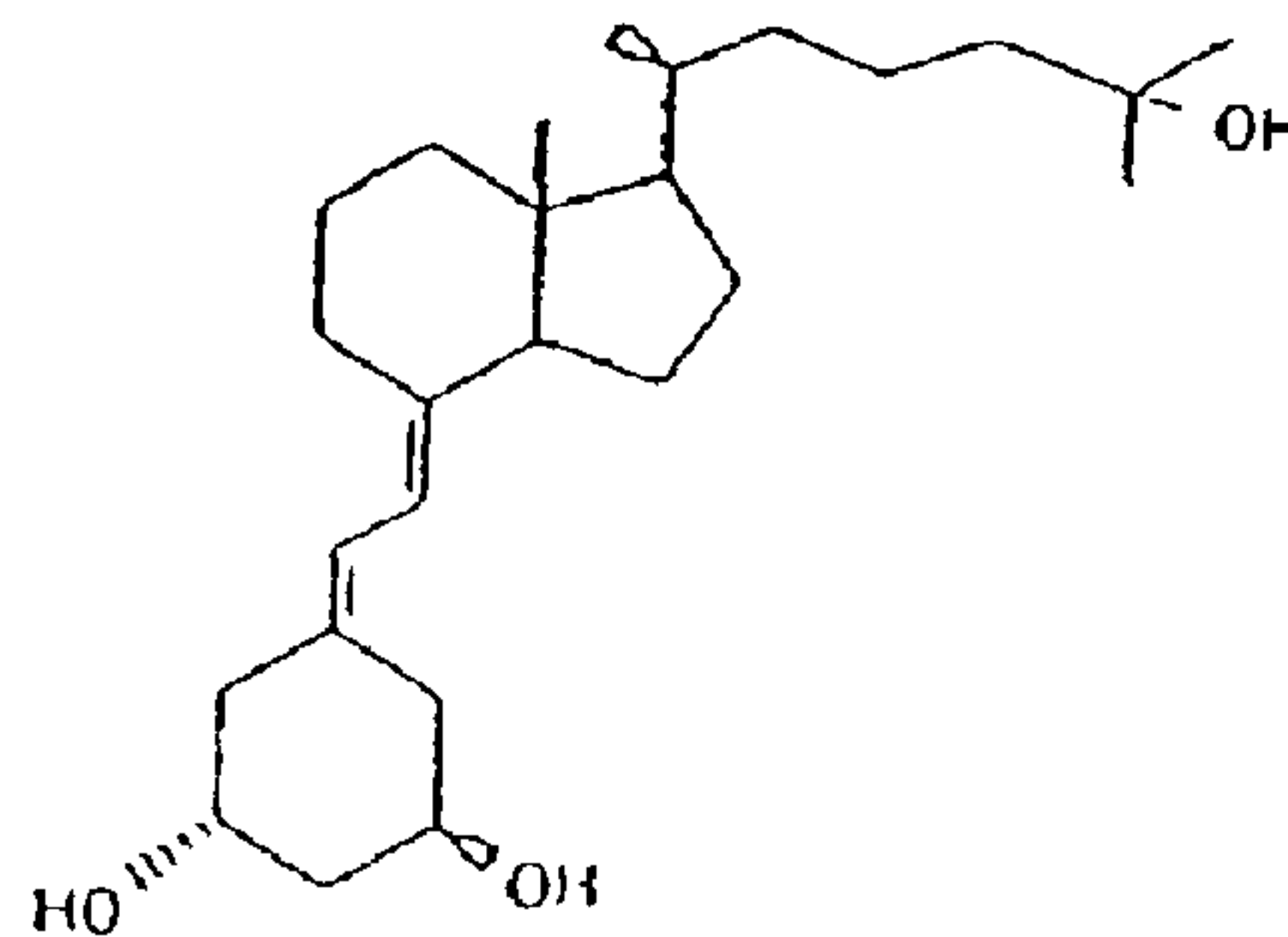
19-nor-21-epi-1 \alpha ,25-dihydroxyvitamin D 3
