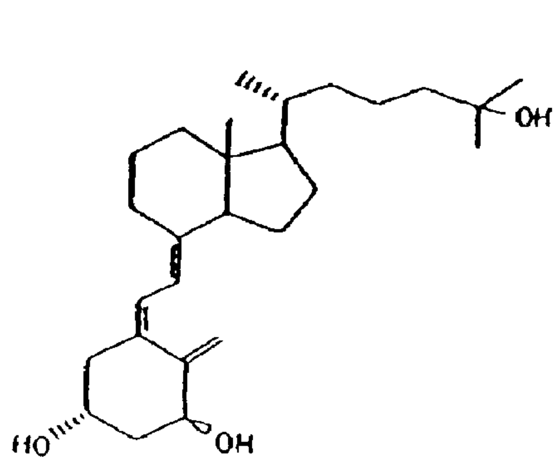
1 \alpha , 25-dihydroxyvitamin D 3
