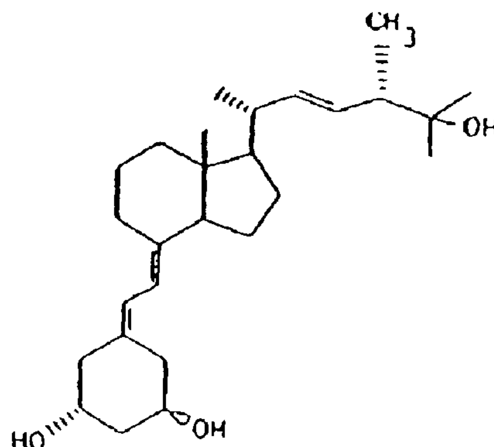
19-nor-1 \alpha ,25-dihydroxyvitamin D 2
