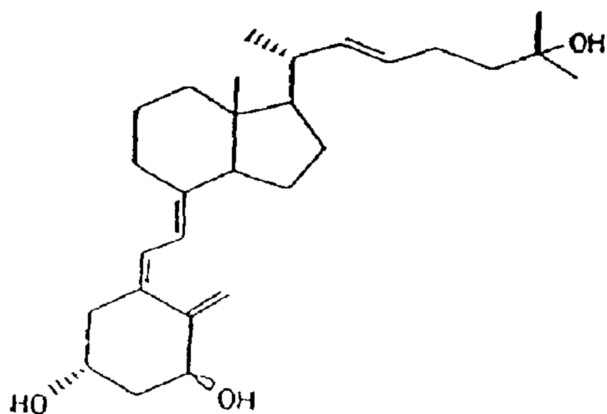
24-homo-22-dehydro-22E-1 \alpha ,25-dihydroxyvitamin D 3
