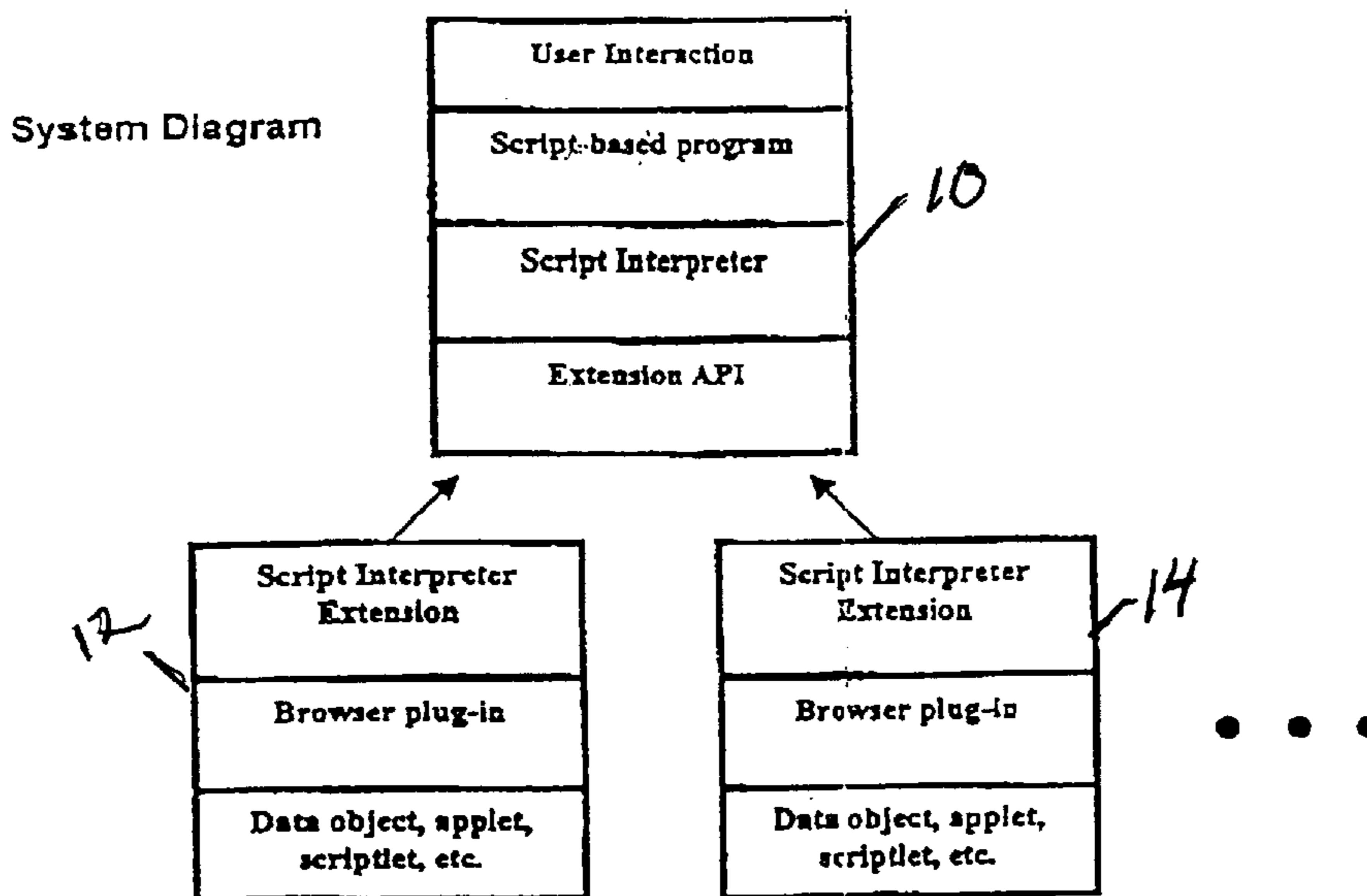
A layer diagram of a typical implementation of the invention using a scripting language platform such as Tcl/Tk. A script interpreter extension provides functions that mimic the browser-side interface of a Web browser plug-in API
