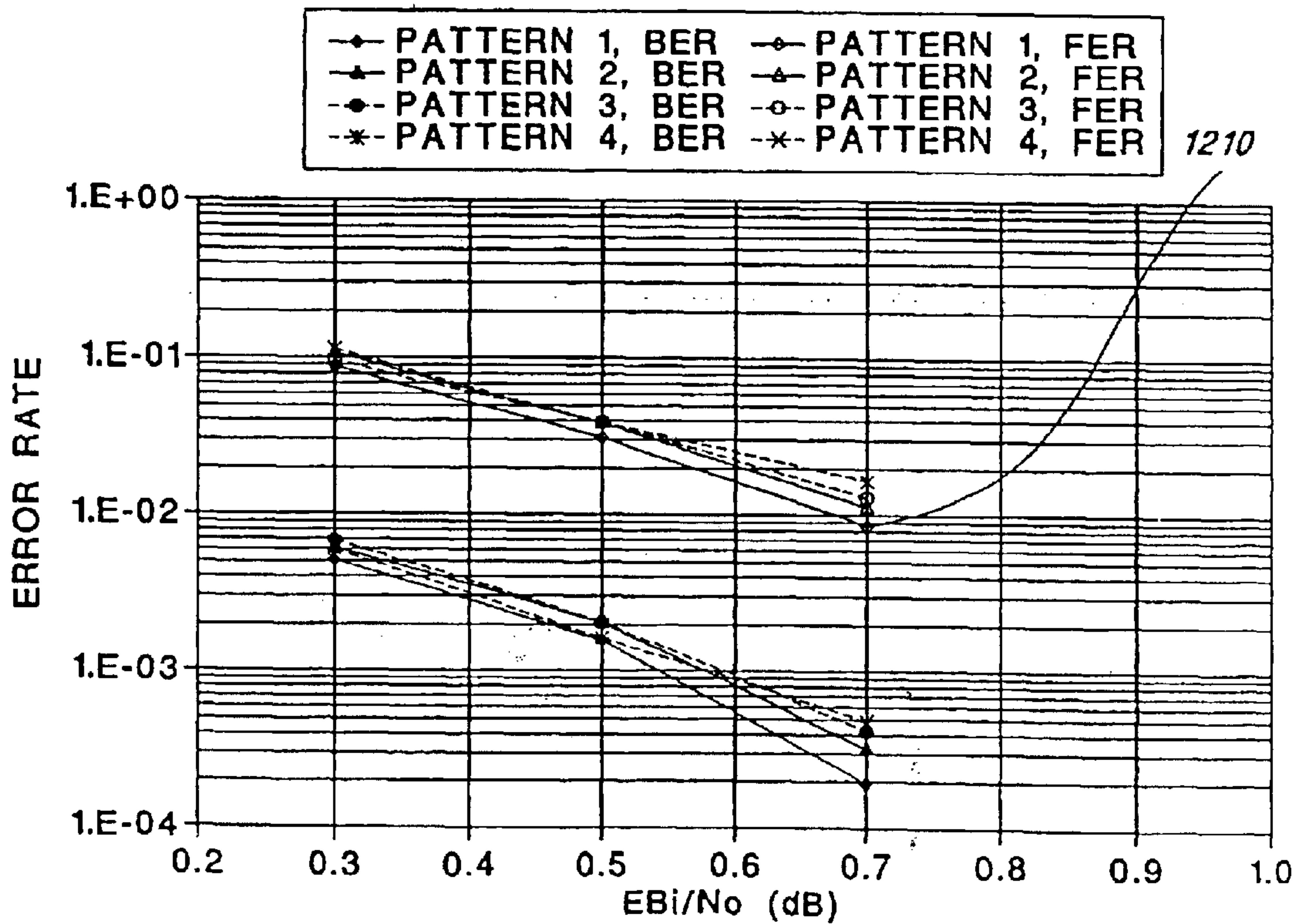
FIG. 12 PERFORMANCE OF CODE #3, FRAME SIZE=512
