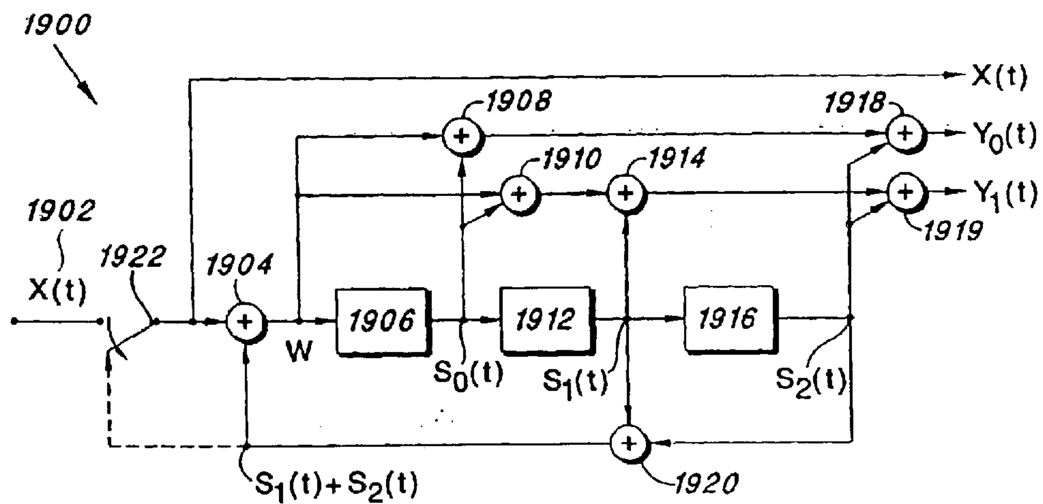
FIG. 19 UNIVERSAL CONSTITUENT ENCODER RECOMMENDED FOR FORWARD LINK TURBO CODES OF VARYING INTERLEAVER DEPTH
