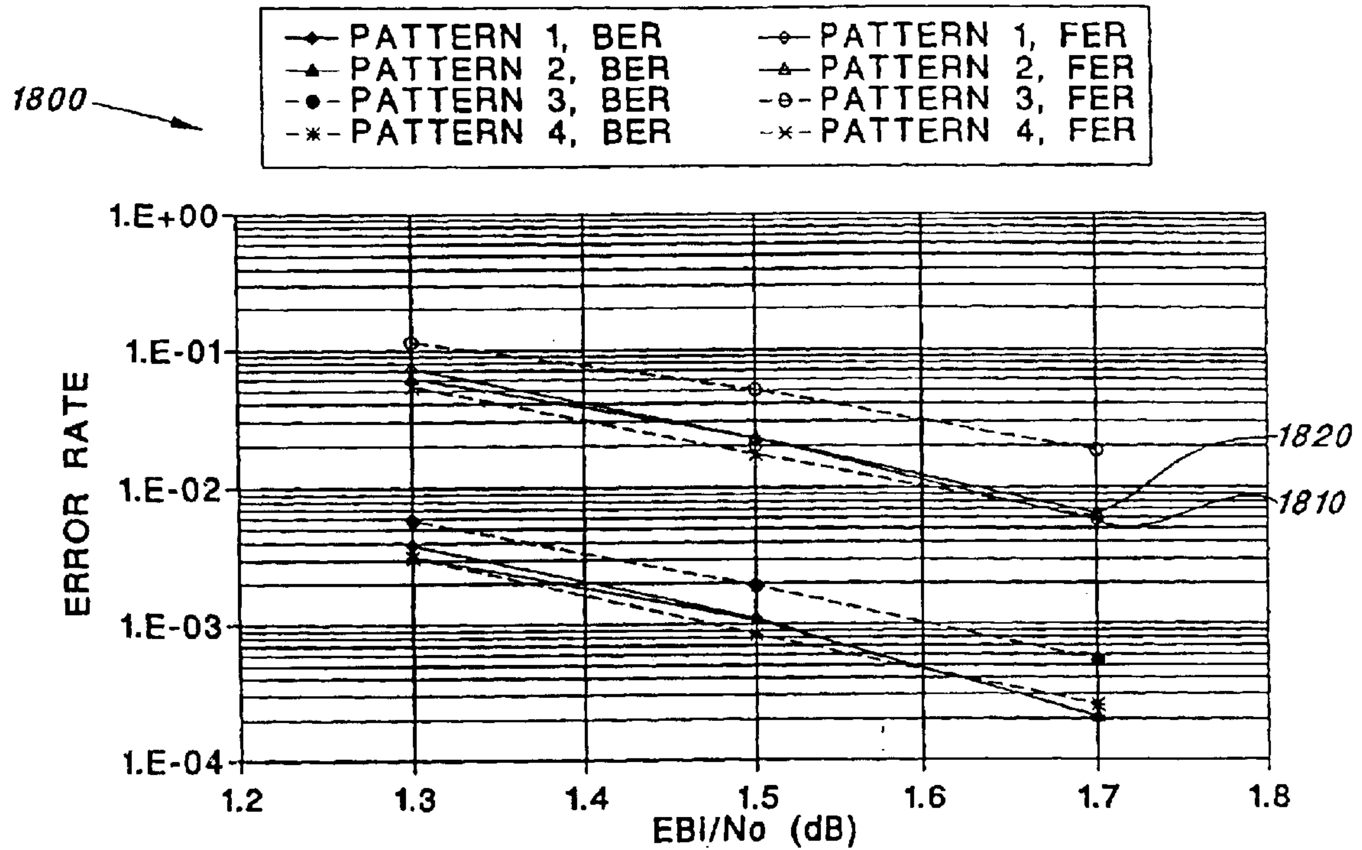
FIG. 18 RATE 1/2 PUNCTURING COMPARISON, FRAME=512
