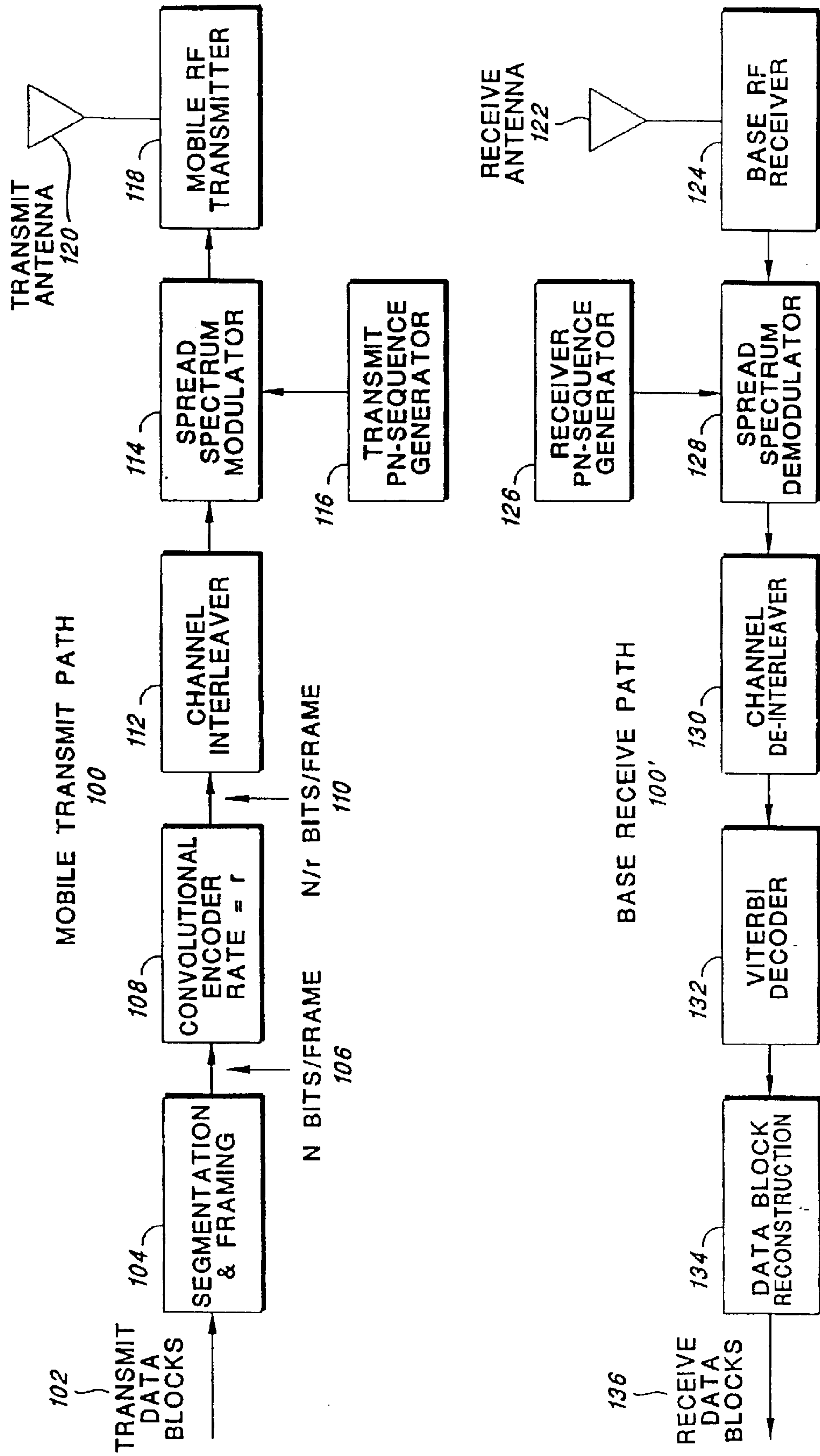
BLOCK DIAGRAM OF A DIRECT SEQUENCE CDMA DIGITAL CELLULAR MOBILE TRANSMITTER AND BASE RECEIVER
