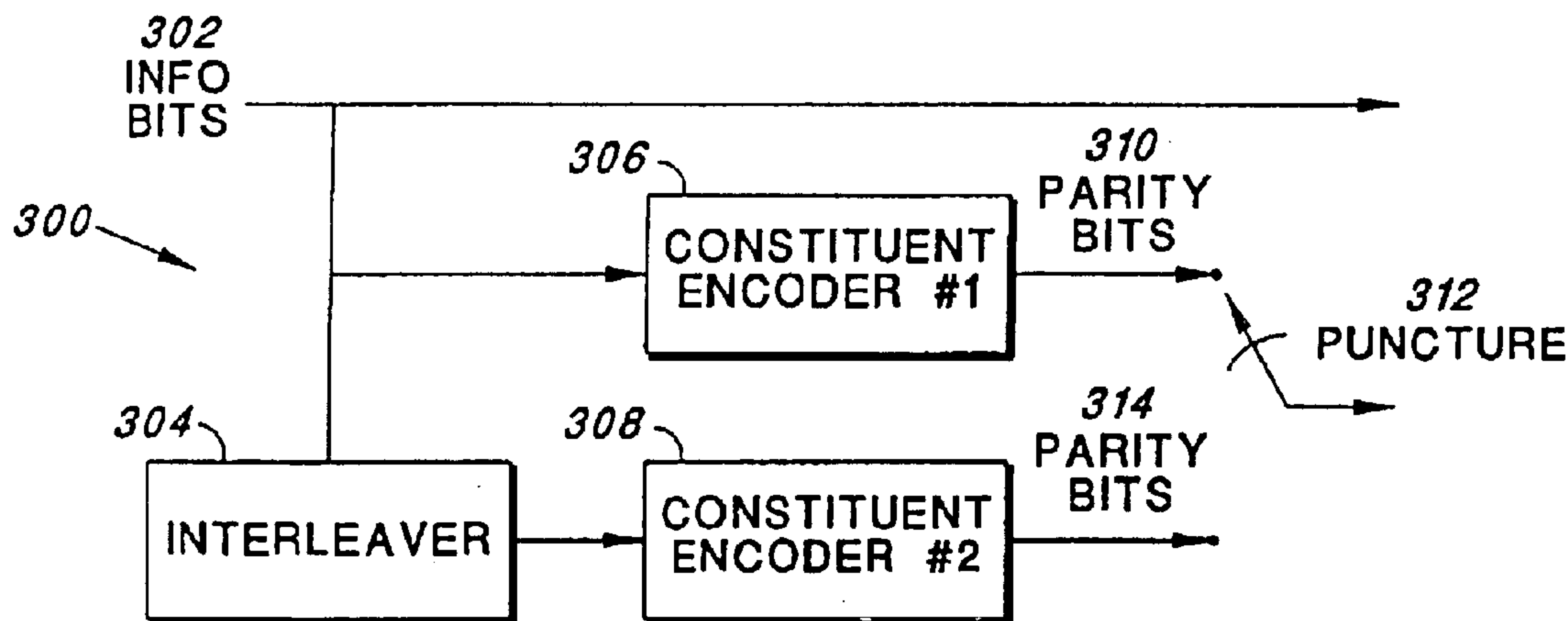
GENERIC TURBO CODE ENCODER BLOCK DIAGRAM
