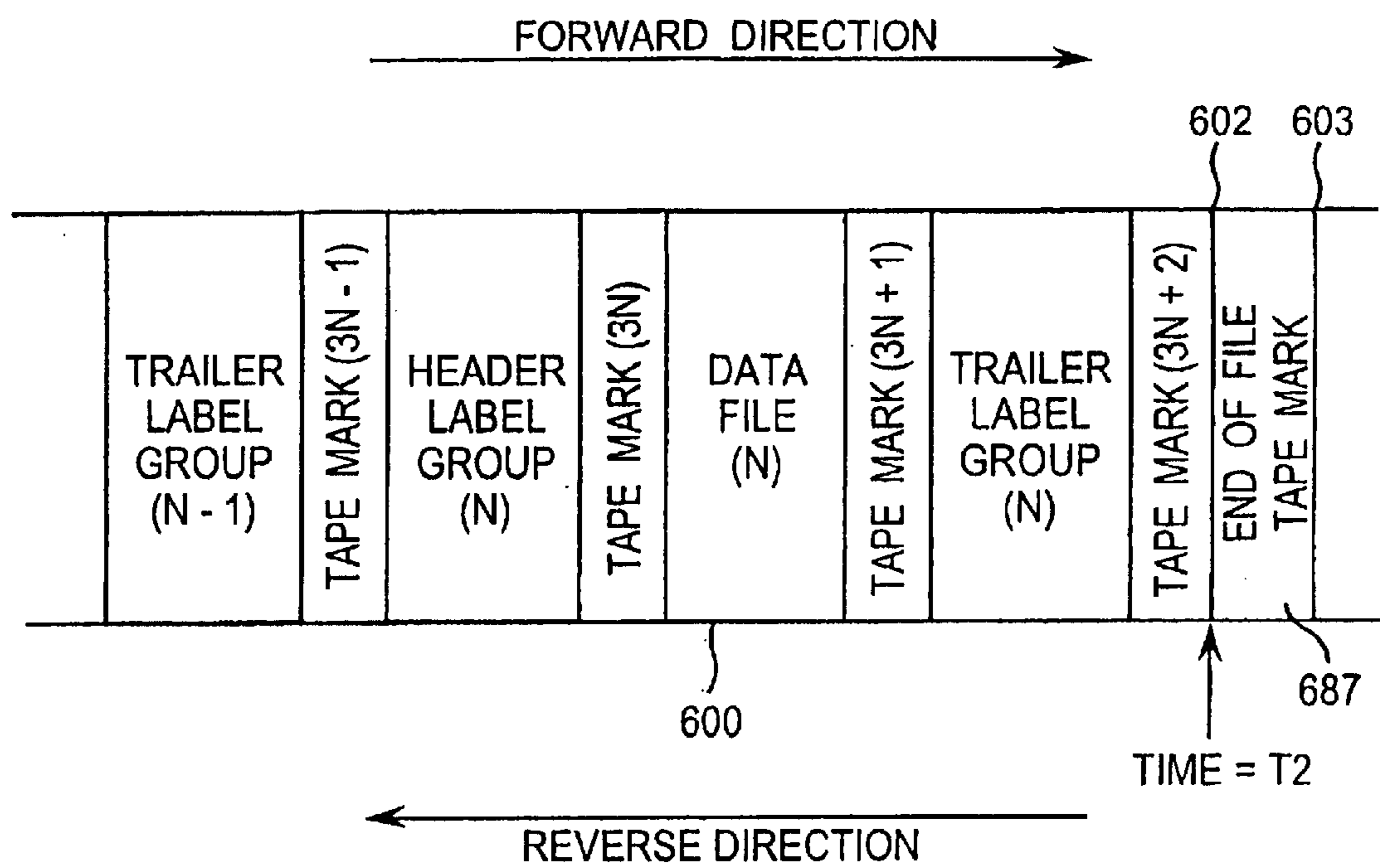
FIG. 6D PRIOR ART
