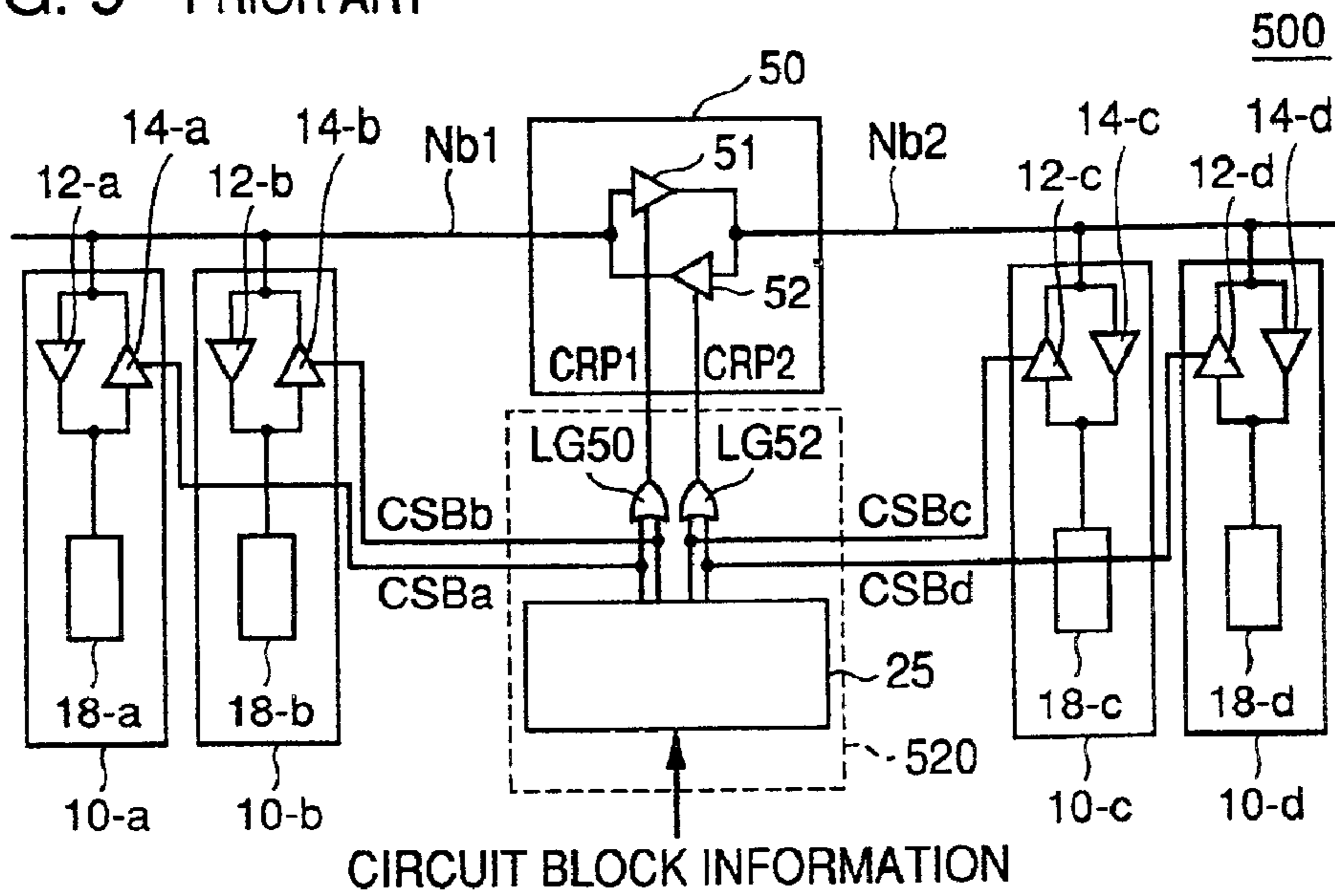
FIG. 9 PRIOR ART
