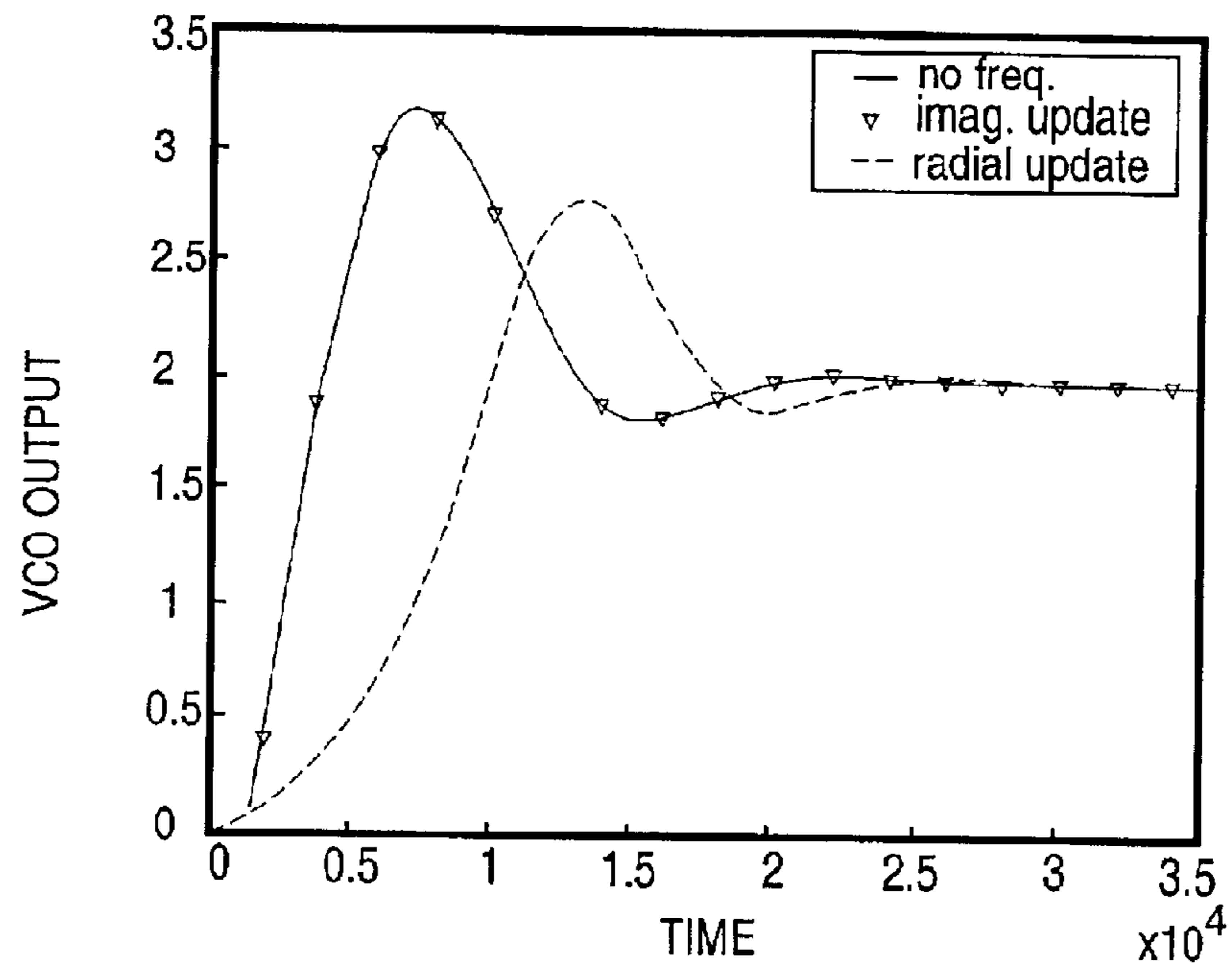
Transient Response for 0dB attenuation
