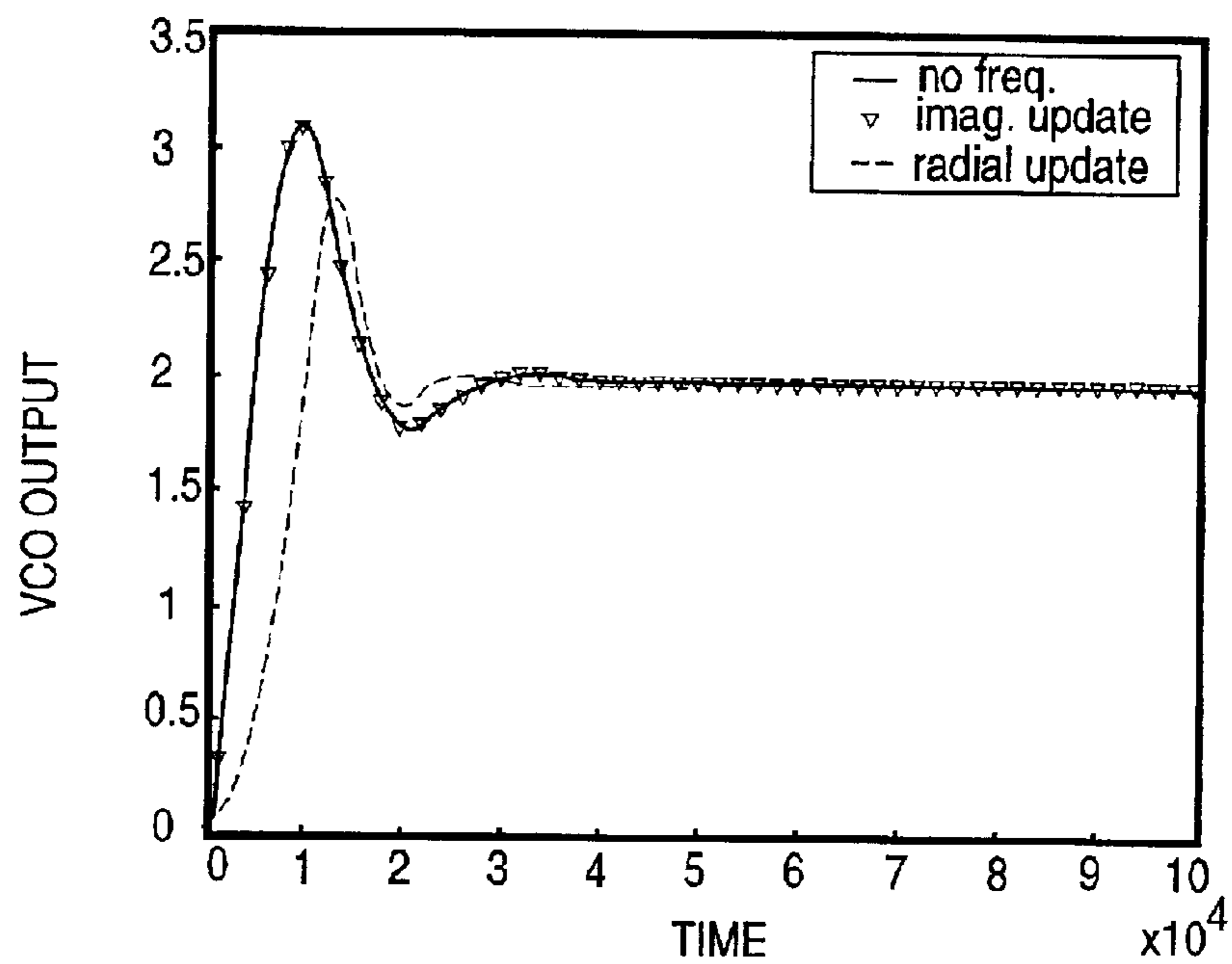
Transient Response for 3dB attenuation
