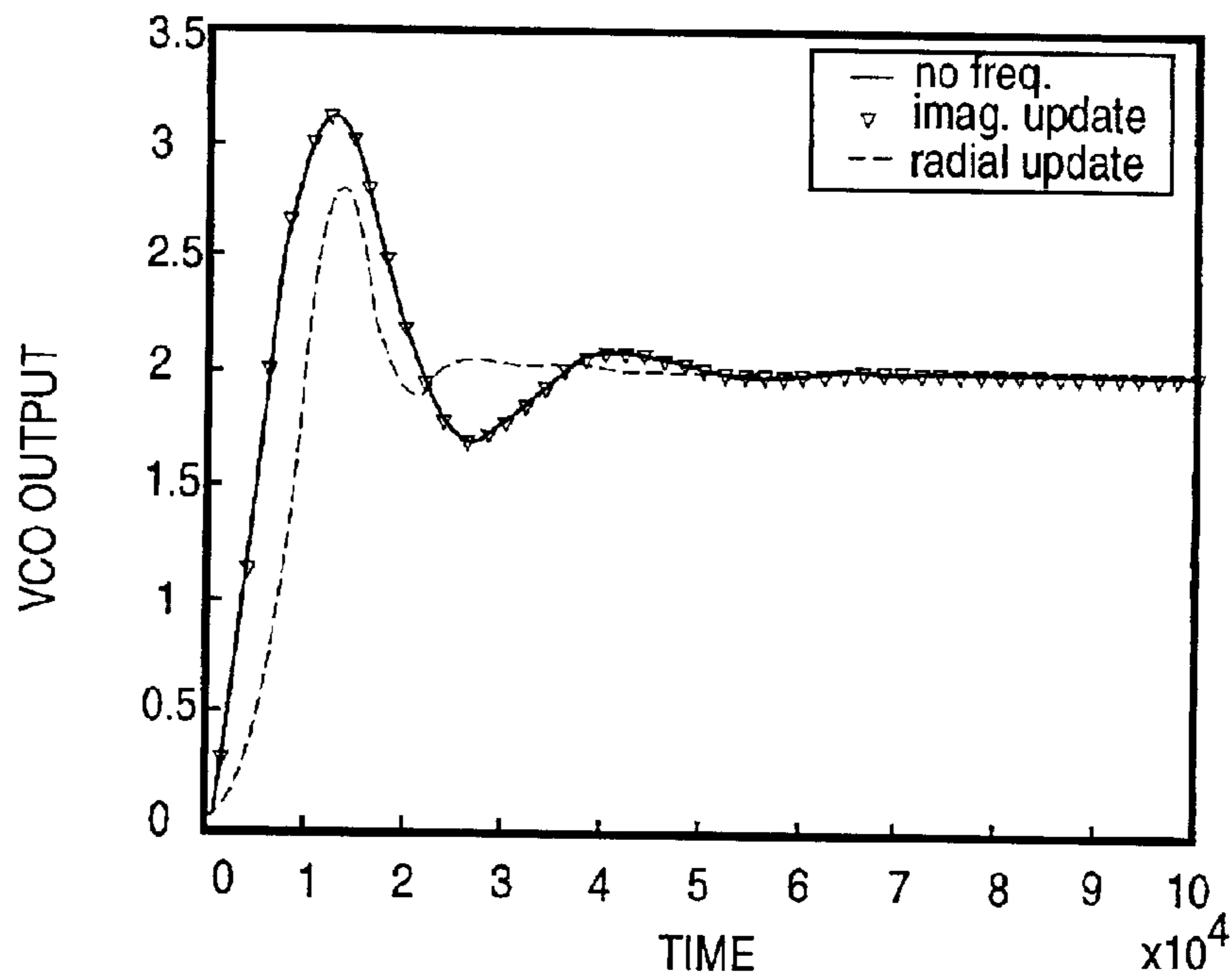
Transient Response for 6dB attenuation
