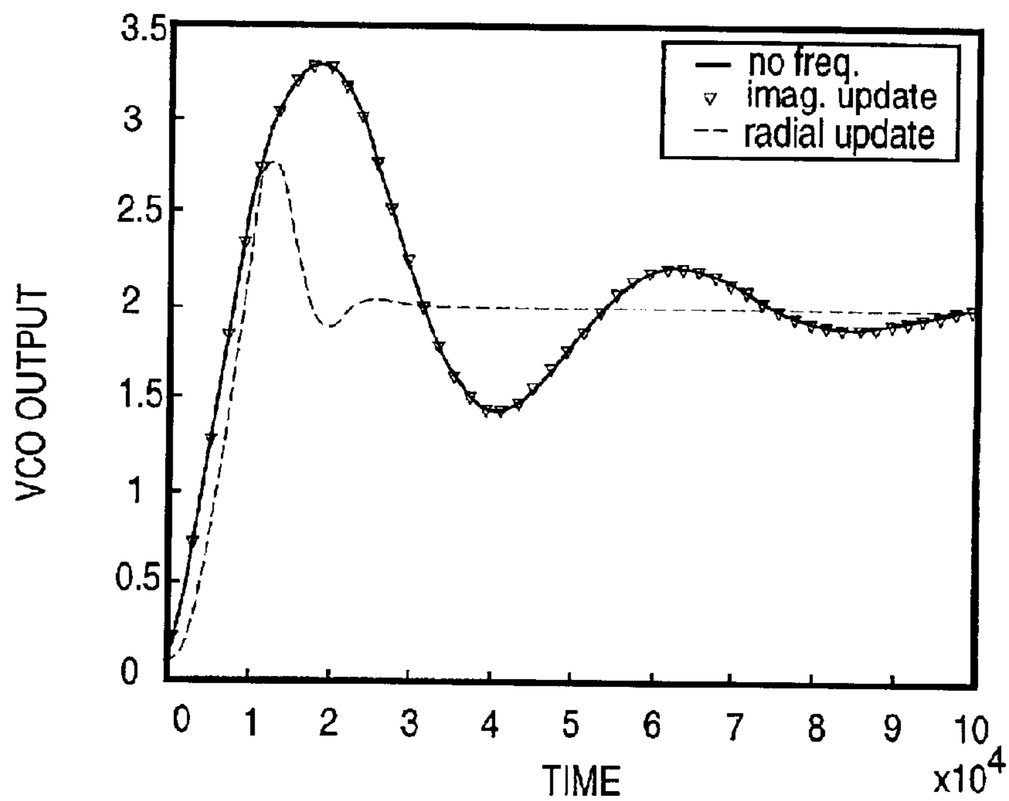
Transient Response for 12dB attenuation
